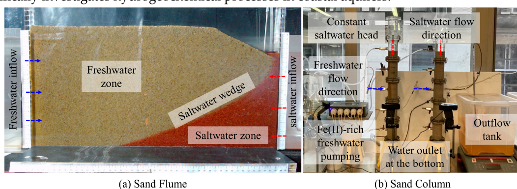
Figure 5. Schematic illustration of (a) sand flume and (b) sand column. A sand flume test can be used to investigate pathways and mechanisms under various predetermined forcing circumstances, such as different tidal ranges and net groundwater flow rates, while a sand column test can be typically utilized to explore the migration of certain compounds in a particular substrate. .
