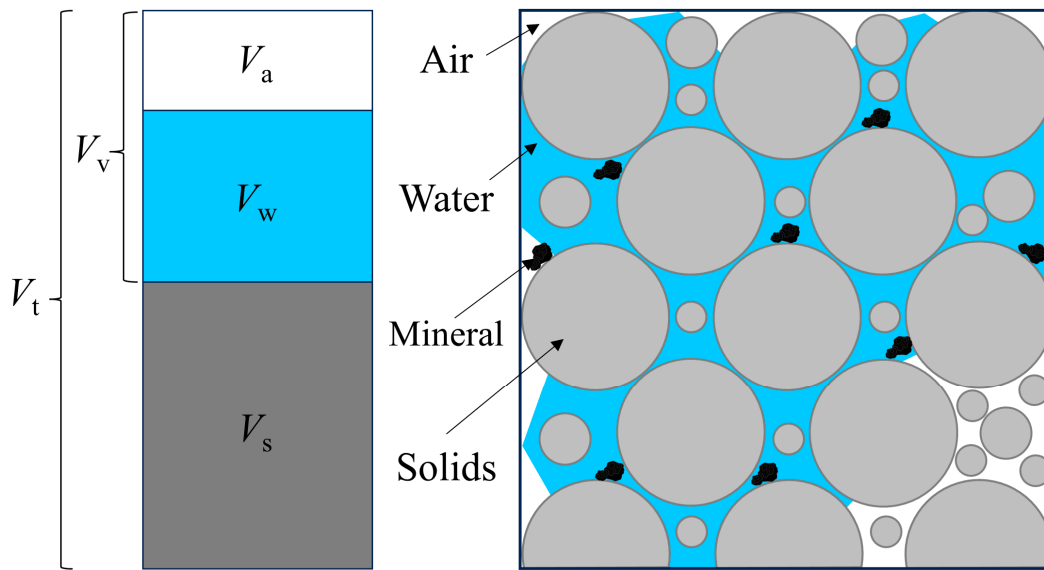
Figure 9. Phase relationship diagram in a cross section of REV-scale porous media, where V_t is the total volume, V_v is the void volume, which equals the water volume V_w under fully saturated conditions, and V_s is the volume of solid particles and precipitated minerals.
