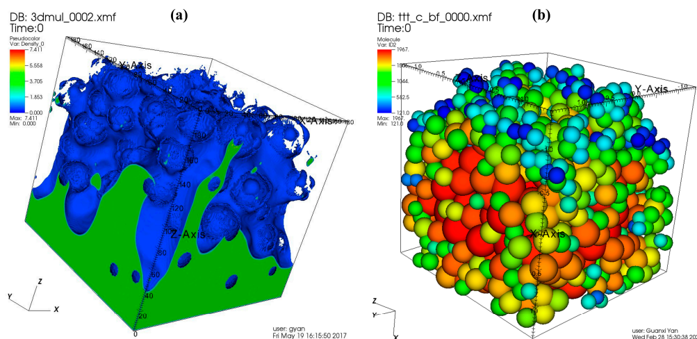
Figure 15. A demonstration of CFD using LBM coupled with DEM: (a) CFD carried out using LBM and (b) soil particle package set inside a REV using DEM.
