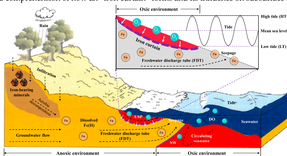
Figure 2. Conceptual model illustrating the hydrological and geochemical processes in the intertidal area [31]. The colored areas indicate different geochemical zonations, and black dashed arrows represent groundwater flow. In between the saltwater wedge (SW) and the upper saline plume (USP) lies a freshwater discharge tube (FDT).
