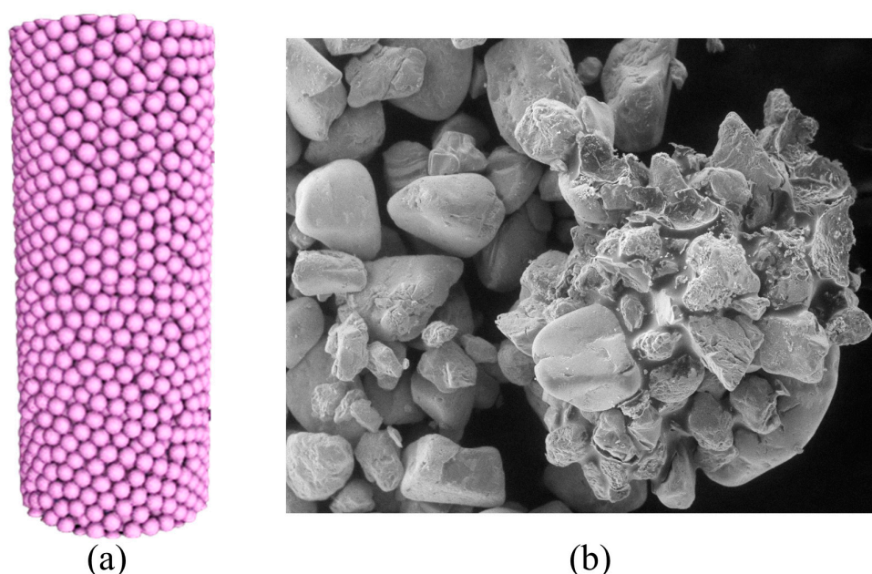
Figure 8. a) 3-D micro-CT image of solid particles, and (b) SEM image of sand grains and pore space changes due to Fe precipitation.
