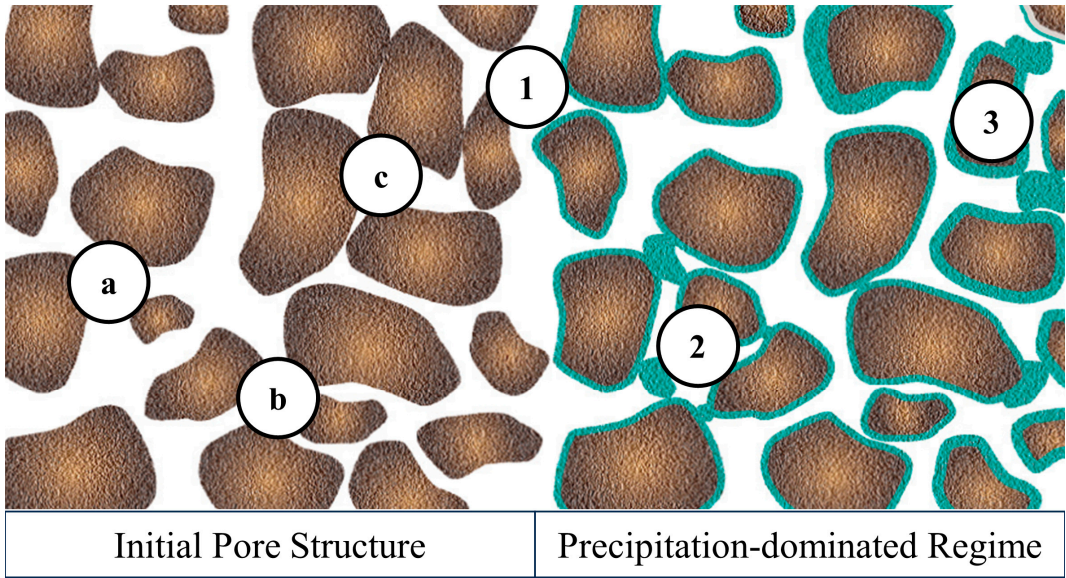
Figure 7. Schematic illustration of the effect of precipitation process on pore structure. Brown area represents solid particles (e.g., quartz sand), while green coatings are solid-phase precipitation.
