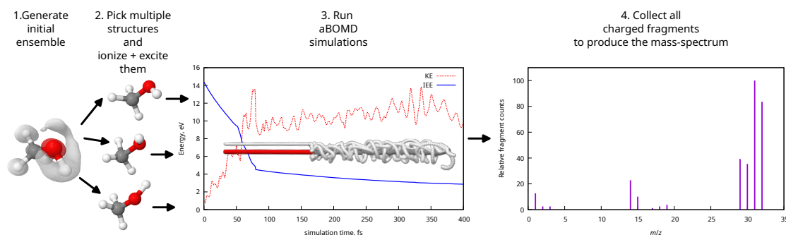
Figure 3. Graphical representation of a mass spectra simulation using aBOMD approach.
