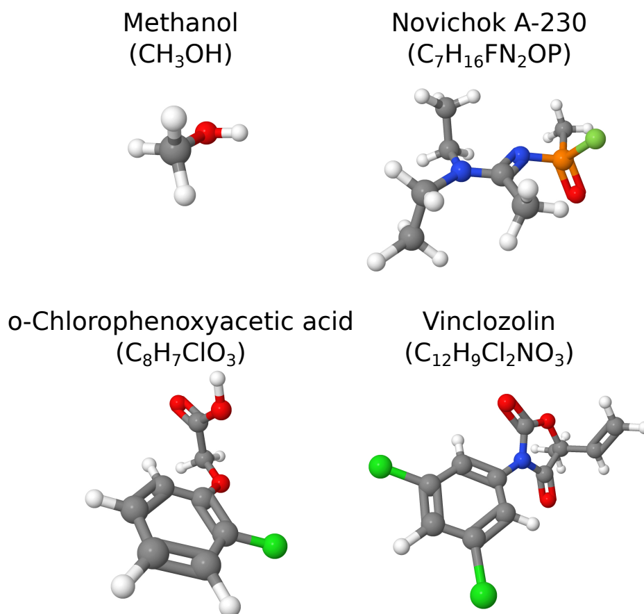
Figure 4. The most stable conformers of four test molecules used in the theoretical mass-spectra prediction.
