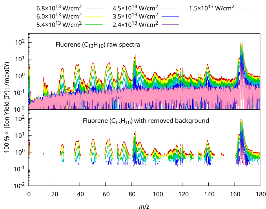
Figure 7. Experimental mass spectra of fluorene ( \text{C}_{13}\text{H}_{10} ) obtained by strong-field ionization with ultrashort laser pulses of varied peak intensity. The top figure shows raw experimental spectra, while the bottom one is after the background removal. Note that the logarithmic scale on the absolute intensity is used for y -axis, and the curve disappearance in the bottom figure means that the signal is zero.
