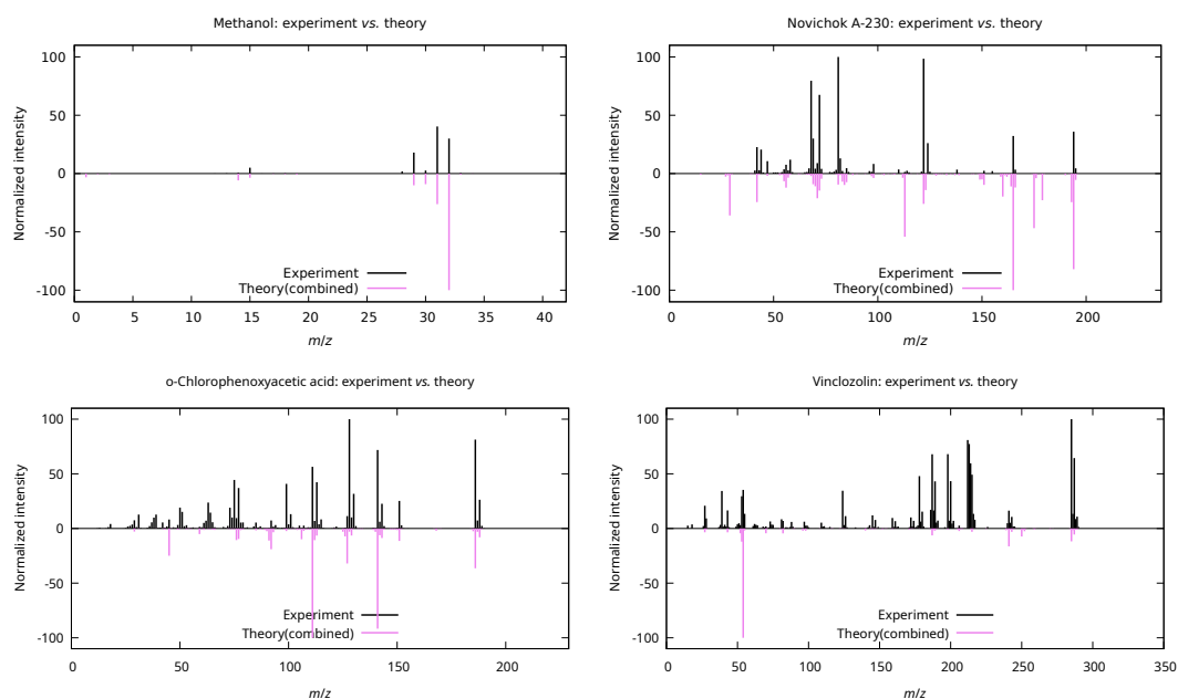
Figure 6. Comparison of the combined theoretical mass spectrum with the experimental one from the database for four test molecules (methanol, novichok A-230, o-chlorophenoxyacetic acid, and vinclozolin from Fig. 4).
