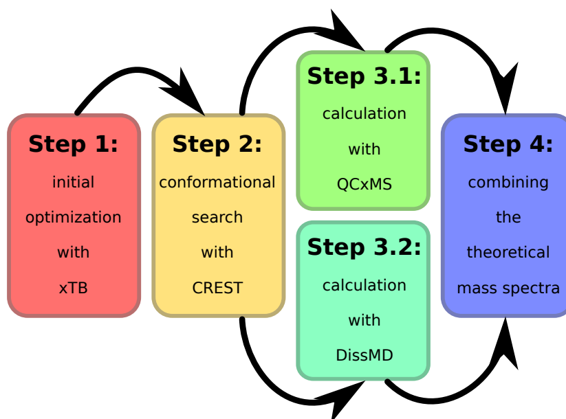
Figure 2. A general workflow scheme applied for the theoretical MS prediction for a given molecule.
