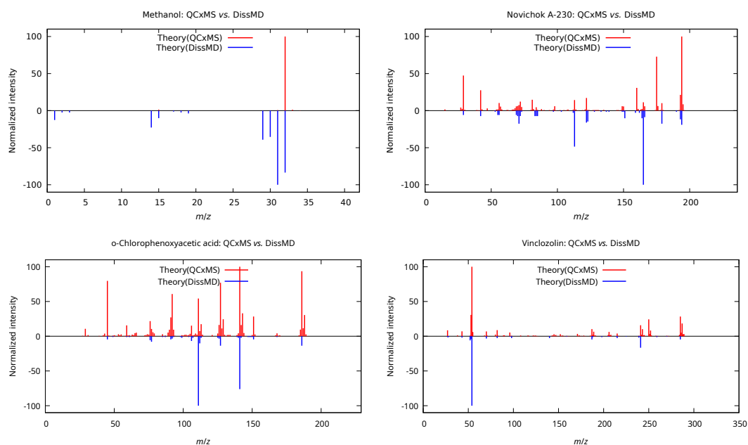
Figure 5. Comparison of the two theoretical mass spectra computed with QCxMS or DissMD software, for four test molecules (methanol, novichok A-230, o-chlorophenoxyacetic acid, and vinclozolin from Fig. 4).
