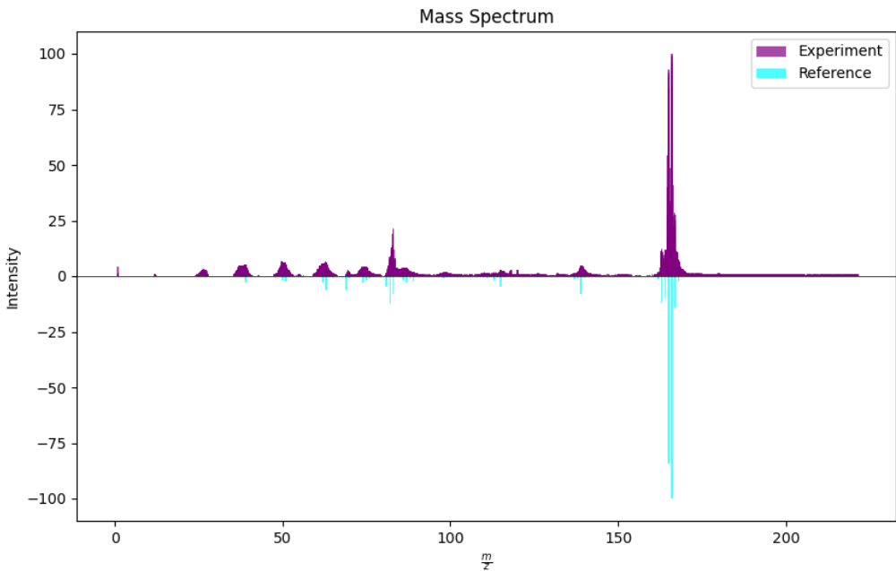
Figure 8. Comparison of the experimental and reference spectrum of fluorene for the highest ( 6.8 \times 10^{13} W/cm 2 ) peak power mass spectra.
