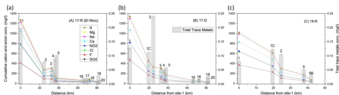
Figure 2. Spatial and temporal variation in cations ( \text{Na}^+ , \text{Ca}^{2+} , \text{Mg}^{2+} , \text{K}^+ : line graphs), anions ( \text{SO}_4^{2-} , \text{Cl}^- , \text{F}^- , \text{NO}_3^- : line graphs) and total trace metals ( \text{Cd} , \text{Cu} , \text{Co} , \text{Cr} , \text{Li} , \text{Pb} , \text{Mo} , \text{Ni} , \text{Se} , \text{U} , \text{V} , \text{Zn} : bar graphs) in water samples from Moquegua river sites. (a) January 2017 (17-R), (b) July 2017 (17-D) and (c) January 2018 (18-R). Error bars represent standard deviation of measurement. Site numbers are given in the labels.
