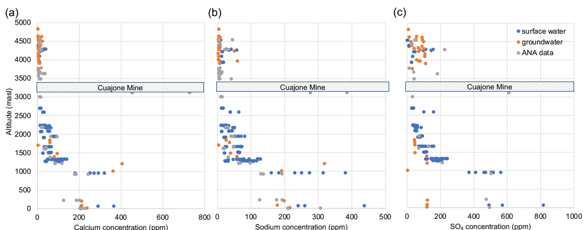
Figure 9. Combined data sources from field work, ANA data and INGEMMET groundwater reports [55, 76–78]. Concentration of major ions in the Torata river system.
