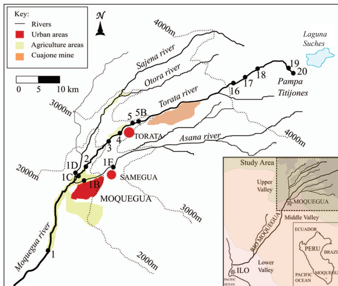
Figure 1. Map of selected study site locations in the foothill and headwaters. (site-0A, 40 km downstream from site 1 near Ilo, is not shown). Inset shows underlying geological units adapted from Decou et al. [29]. Geological lithologies coded by colours: pink- Coastal Batholith (intrusive 145-55 Ma); buff- Moquegua Group (sedimentary 50-4 Ma); green- Cretaceous volcanics and Eocene intrusives; grey- Miocene to recent pyroclastic deposits. Study area shown in dashed box.
