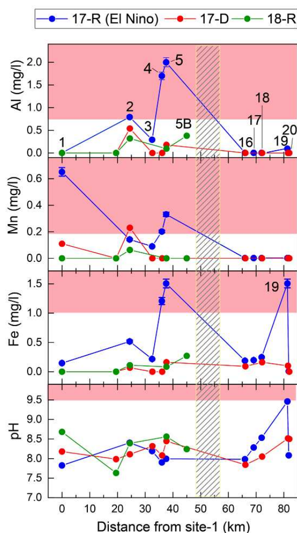
Figure 4. Al, Fe and Mn concentrations and pH, showing elevated wet season metal concentrations in the Torata river below the Cuajone mine. Distance is measured upstream from Site-1. Red shaded regions show the concentration levels above the safe limits for aquatic life. Cuajone mine is located between site-5B and site-16 (vertical shaded region). Error bars represent standard deviation of measurement fluctuation. Labels represent site numbers.
