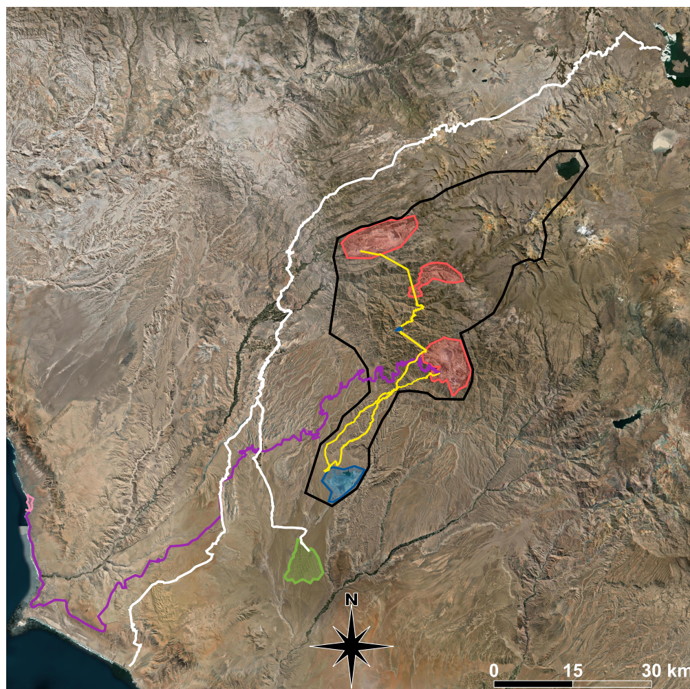
Figure A1. Black polygon: area of direct mining and mine related infrastructural impact. Red polygons: upper red polygon = Southern Copper Cuajone mine, middle red polygon = Anglo American Quellaveco mine, lower red polygon = Southern Copper Toquepala mine. Yellow lines: mine waste channels. Blue polygons: Cortaderas 2 and Quebrada Honda tailings dams. Purple line: railway line to Ilo smelter. Pink polygon: Ilo smelter. White lines: Pasto Grande project irrigation canals (tunnels, concrete lined channels and existing river channels). Green polygon: AH Pampa Sitana irrigation project.
