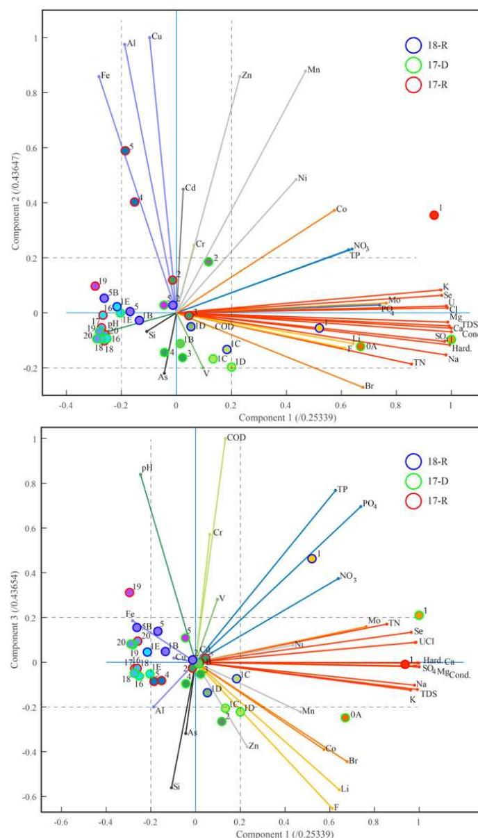
Figure 8. PCA biplots using 33 water parameters measured at 17 Torata-Moquegua sample sites in the three seasons 17-R, 17-D and 18-R. Colours of parameter vectors are taken from Figure 7a. Colours for site points are taken from Figure 7b,c. (a) PC1 vs PC2 (b) PC1 vs PC3. Dashed lines at \pm 0.2 indicate the qualitative boundary used to indicate where components become significant at a site.
