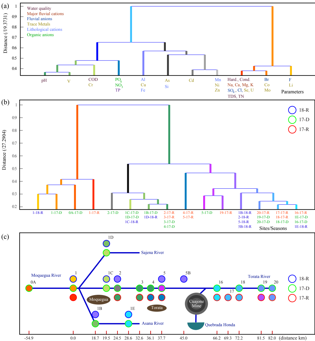
Figure 7. (a) Dendrogram showing the Euclidean dissimilarity between the 33 measured water parameters taking 17 Torata-Moquegua sample sites and three seasons 17-R, 17-D and 18-R into account.(b) Dendrogram showing the largest dissimilarity between the 17 Torata-Moquegua sample sites in different seasons taking 33 measured water parameters into account (c) Beck map showing the spatial distribution of site clusters. The colour map is the same as in (b). The colour of the outer ring of each circle identifies the season using the key on the right.
