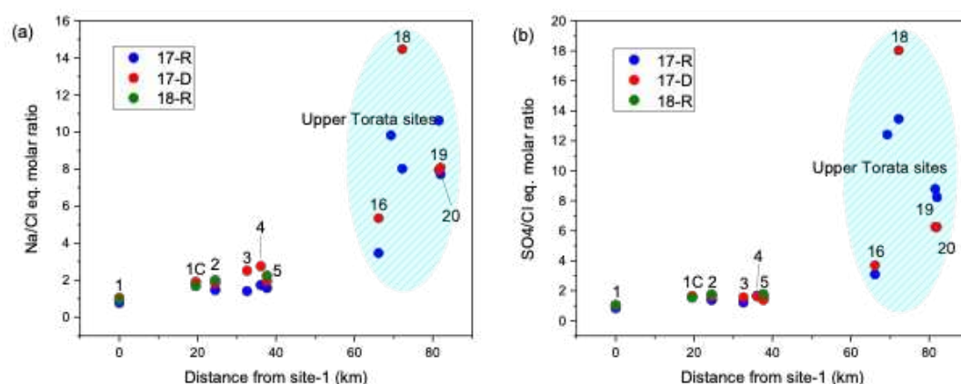
Figure 3. Na/Cl equivalent molar ratio (a) and \text{SO}_4/\text{Cl} equivalent molar ratio (b) graphs for Moquegua river system. This shows that upper Torata sites have significantly higher ratios indicating ground water recharge in this region.
