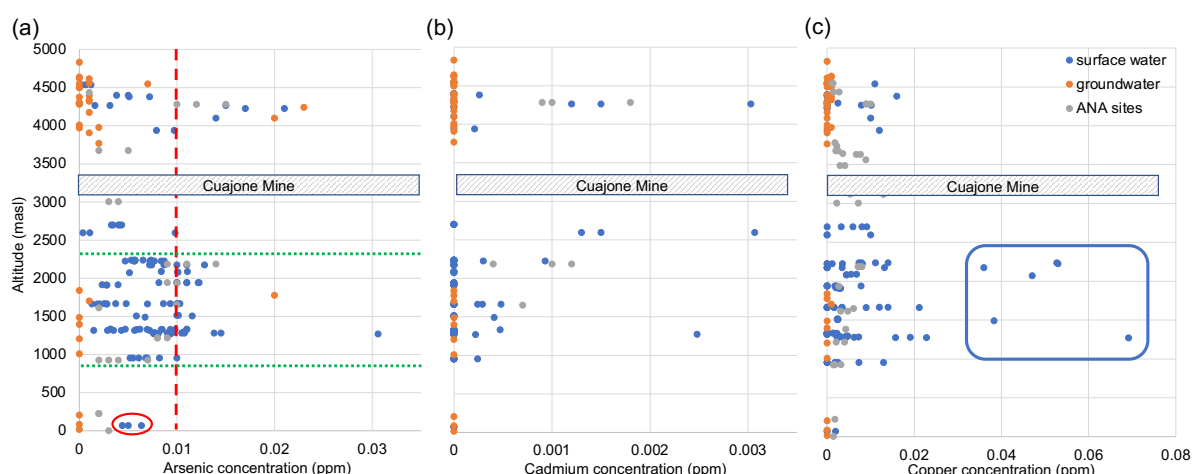
Figure 10. Combined data sources from field work, ANA data and INGEMMET groundwater report [55, 76–78]. Concentration of trace elements in the Torata river system. The red dashed line in panel (a) indicates the safe limit for arsenic. The safety limits for cadmium and copper concentrations do not appear in panels (b) and (c) as they are above every data point. The green dotted lines in panel (a) delimit the area of intensive agricultural land ranging from above Torata to below Moquegua. The red circle in panel (a) identify data taken at Site O. The blue box in panel (c) outline data that were taken after a flash flood event.
