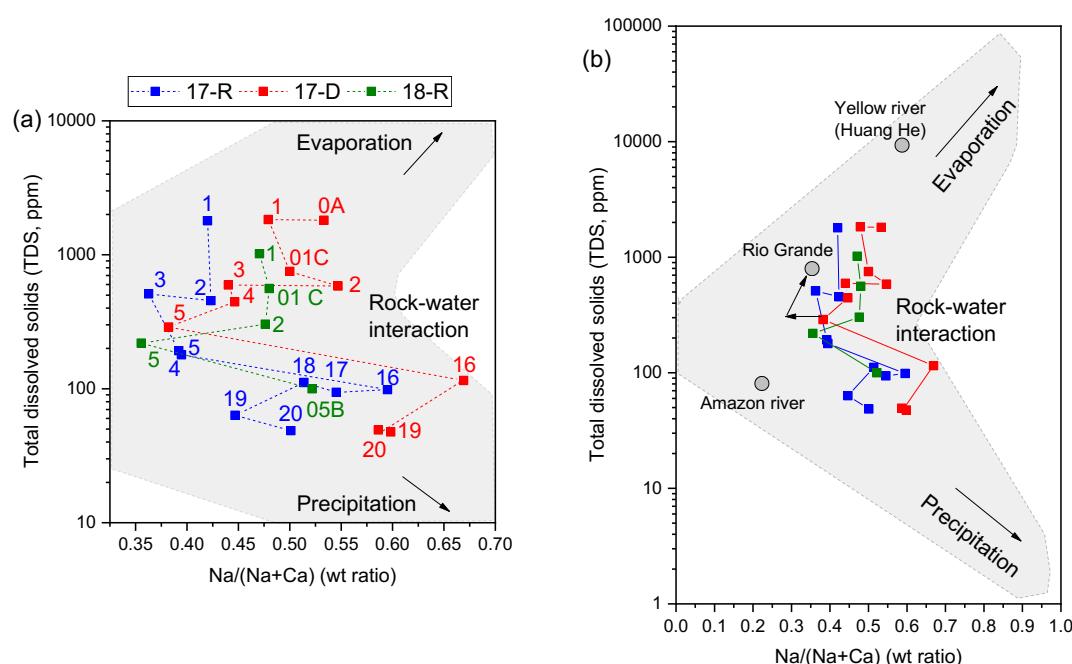
Figure 5 : (a) Gibbs plot for the Moquegua river showing changes in water chemistry along the river and (b) compared with other major rivers, Huang He river, China and Amazon river, Rio Grande, USA and Amazon river, South America. Data from [58,59].
