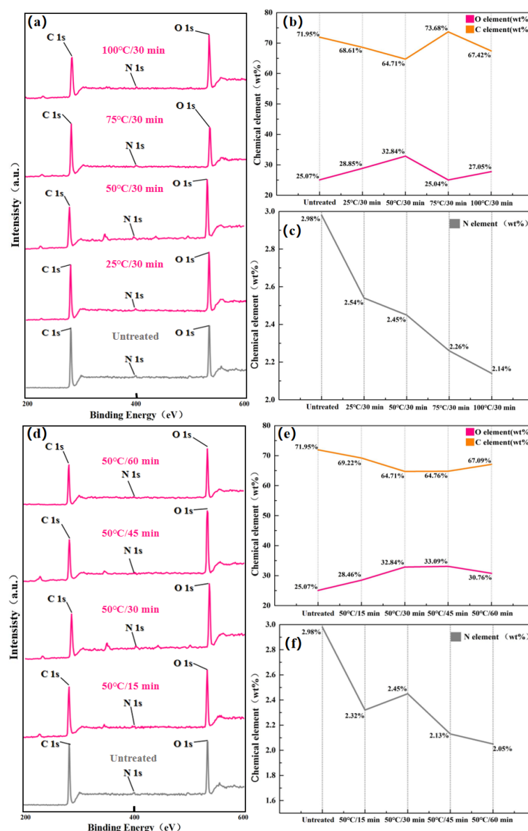
Figure 8. Surface elemental content before and after Acid-etching. (a)XPS full spectrum of chemical elements in the surface of laminate (Temperature-variable experimental groups). (b)Percentage of elemental content of C and O in the surface of laminate (Temperature-variable experimental groups). (c)Percentage of elemental content of N in the surface surface of laminate (Temperature-variable experimental groups). (d)XPS full spectrum of chemical elements in the surface of laminate (Time-variable experimental groups). (e)Percentage of elemental content of C and O in the surface layer of laminate (Time-variable experimental groups). (f)Percentage of elemental content of N in the surface of laminate (Time-variable experimental groups).
