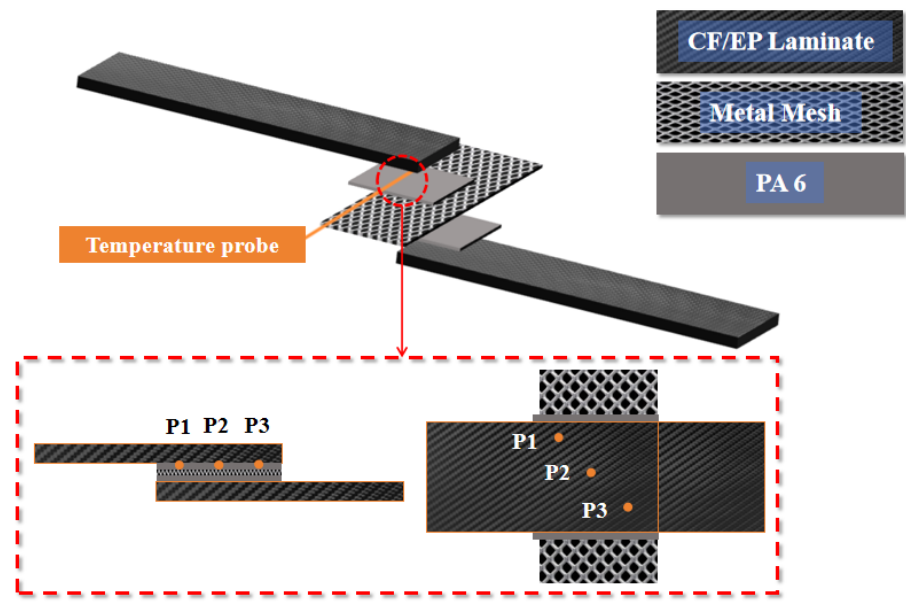
Figure 2. Heat detection method.
