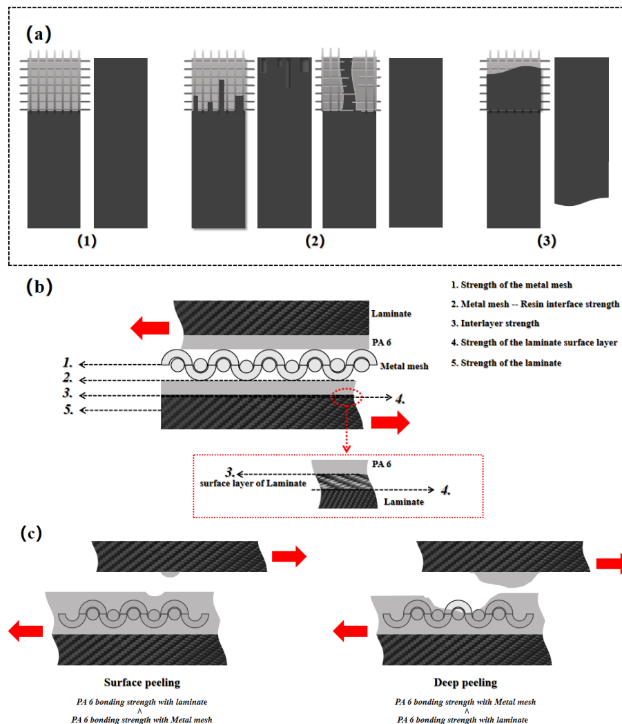
Figure 11. (a)welded joint failure mode. (b)critical strength interface. (c)thermoplastic resin layer failure mode.
