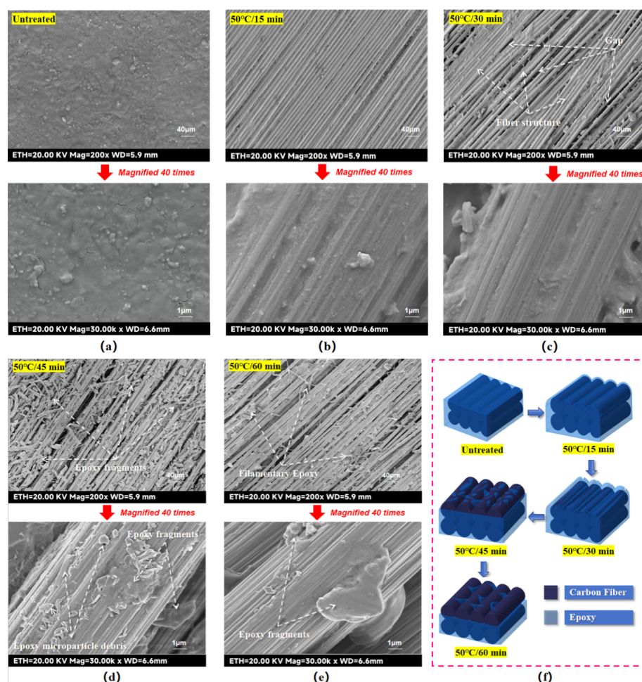
Figure 6. FE-SEM observation of Acid-etching effect (Time-variable experimental groups). (a)Untreated sample. (b)50°C/15 min-treated sample. (c)50°C/30 min-treated sample. (d)50°C/45 min-treated sample. (e)50°C/60 min-treated sample. and (f)Mechanism diagram of Acid-etching action.
