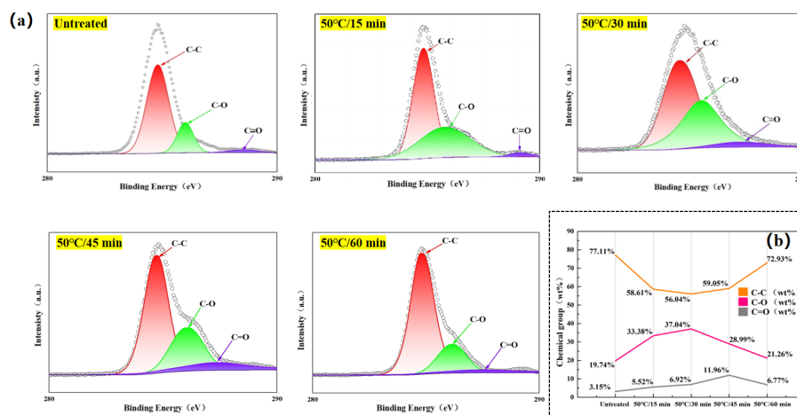
Figure 10. Results of XPS analysis of samples (Time-variable experimental groups). (a) High-resolution C 1s fitted peaks of laminates. (b) Percentage of chemical groups content in the surface layer.
