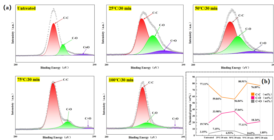
Figure 9. Results of XPS analysis of samples (Temperature-variable experimental groups). (a) High-resolution C 1s fitted peaks of laminates. (b) Percentage of chemical groups content in the surface layer.
