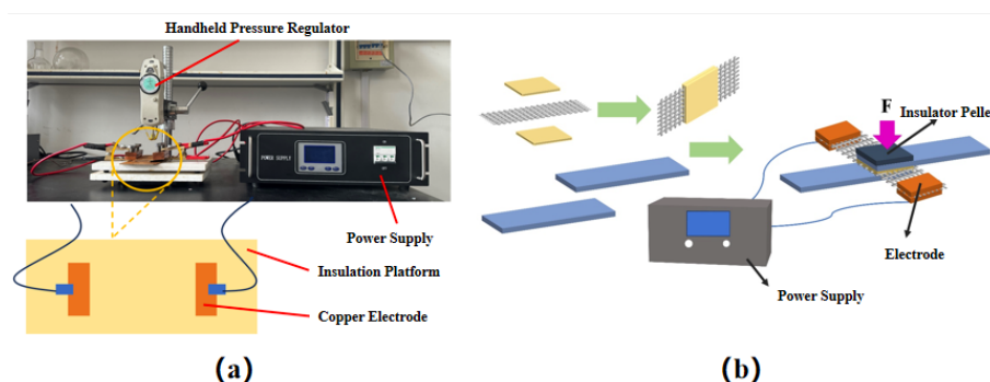
Figure 1. Resistance welding platform and welding process. (a) Self-built resistance welding platform. (b) Resistance welding process.
