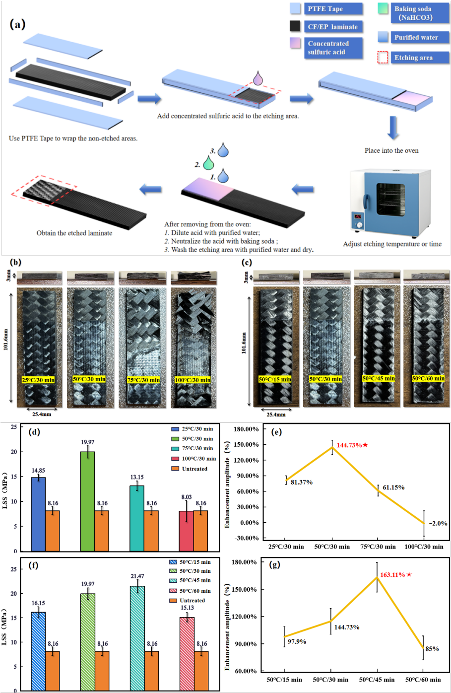
Figure 4. Acid-etching treatment of CF/EP laminates. (a) Acid-etching method. (b) Surface morphology of laminates for Temperature-variable groups. (c) Surface morphology of laminates for Time-variable groups. (d) LSS for Temperature-variable groups. (e) Percentage of increase in LSS for Temperature-variable groups. (f) LSS for Time-variable groups. (g) Percentage of increase in LSS for Time-variable groups.
