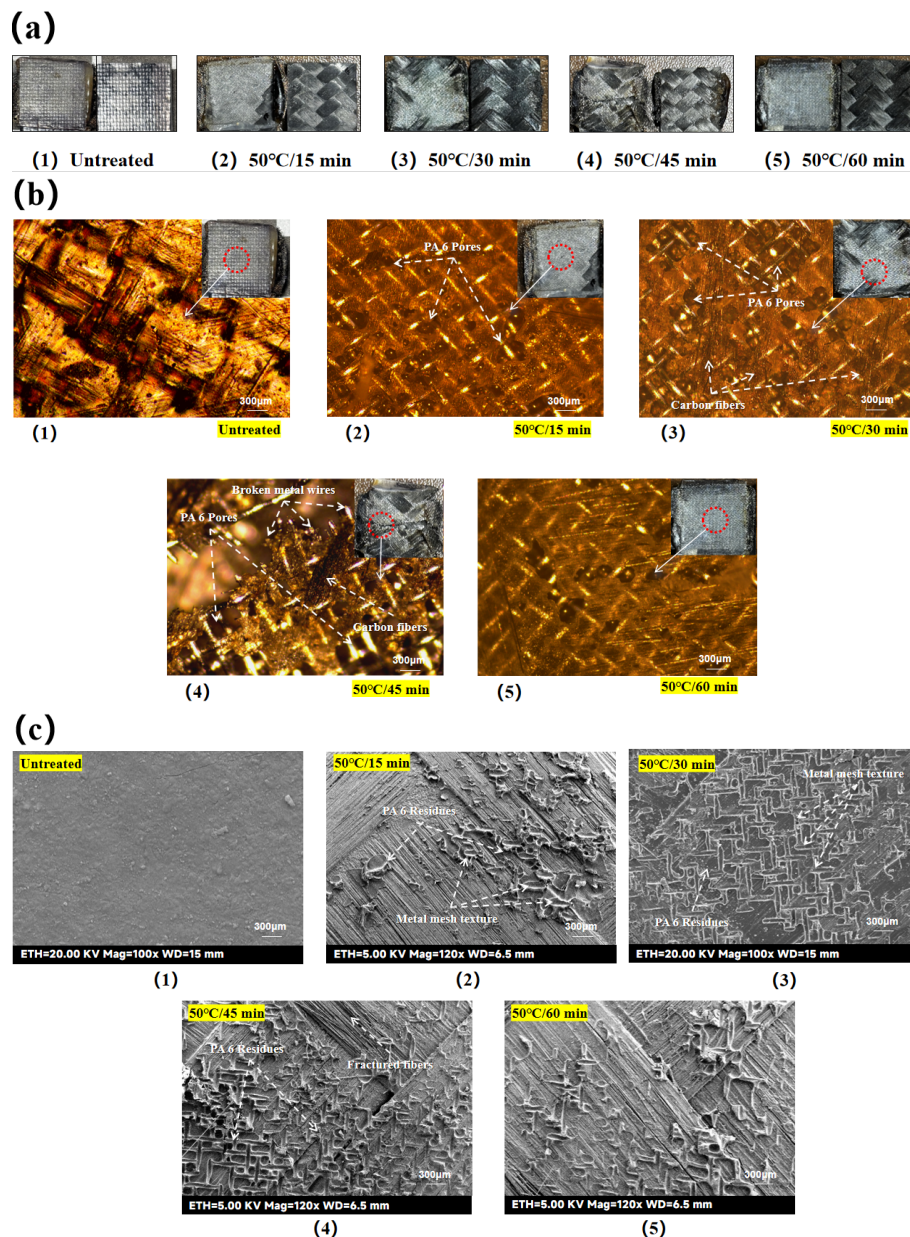
Figure 13. Morphological observation of welded joint failure interface (Time-variable experimental groups). (a)welded joint failure interface. (b)heating element failure interface. (c)laminate failure interface.
