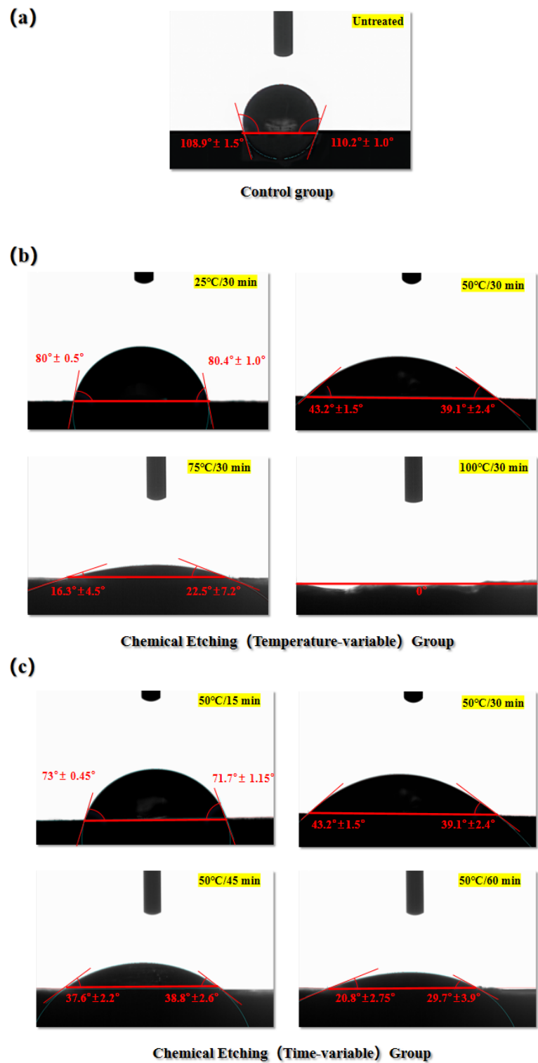
Figure 7. Surface contact angle of materials after surface treatment with different variable (Time-variable, Temperature-variable) groups. (a)Surface contact angle of untreated parts. (b)Surface contact angle of Temperature-variable experimental groups. (c)Surface contact angle of Time-variable experimental groups.
