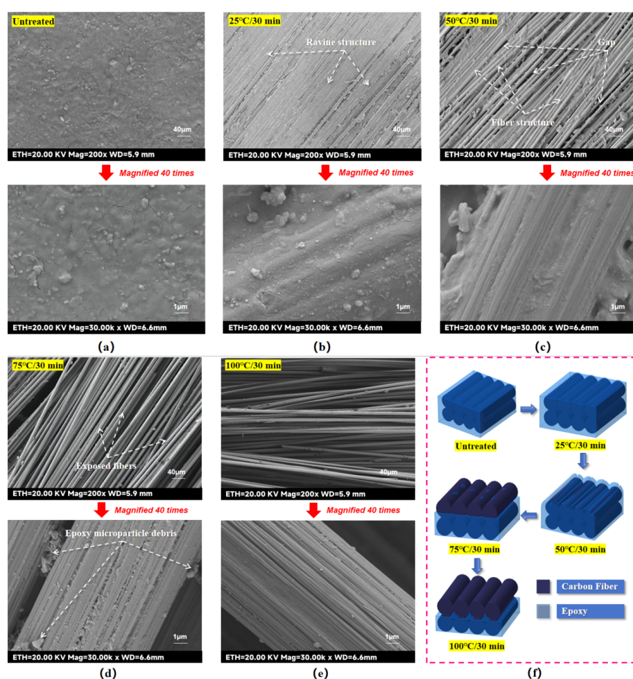
Figure 5. FE-SEM observation of Acid-etching effect (Temperature-variable experimental groups). (a) Untreated sample. (b) 25°C/30 min-treated sample. (c) 50°C/30 min-treated sample. (d) 75°C/30 min-treated sample. (e) 100°C/30 min-treated sample. and (f) Mechanism diagram of Acid-etching action.
