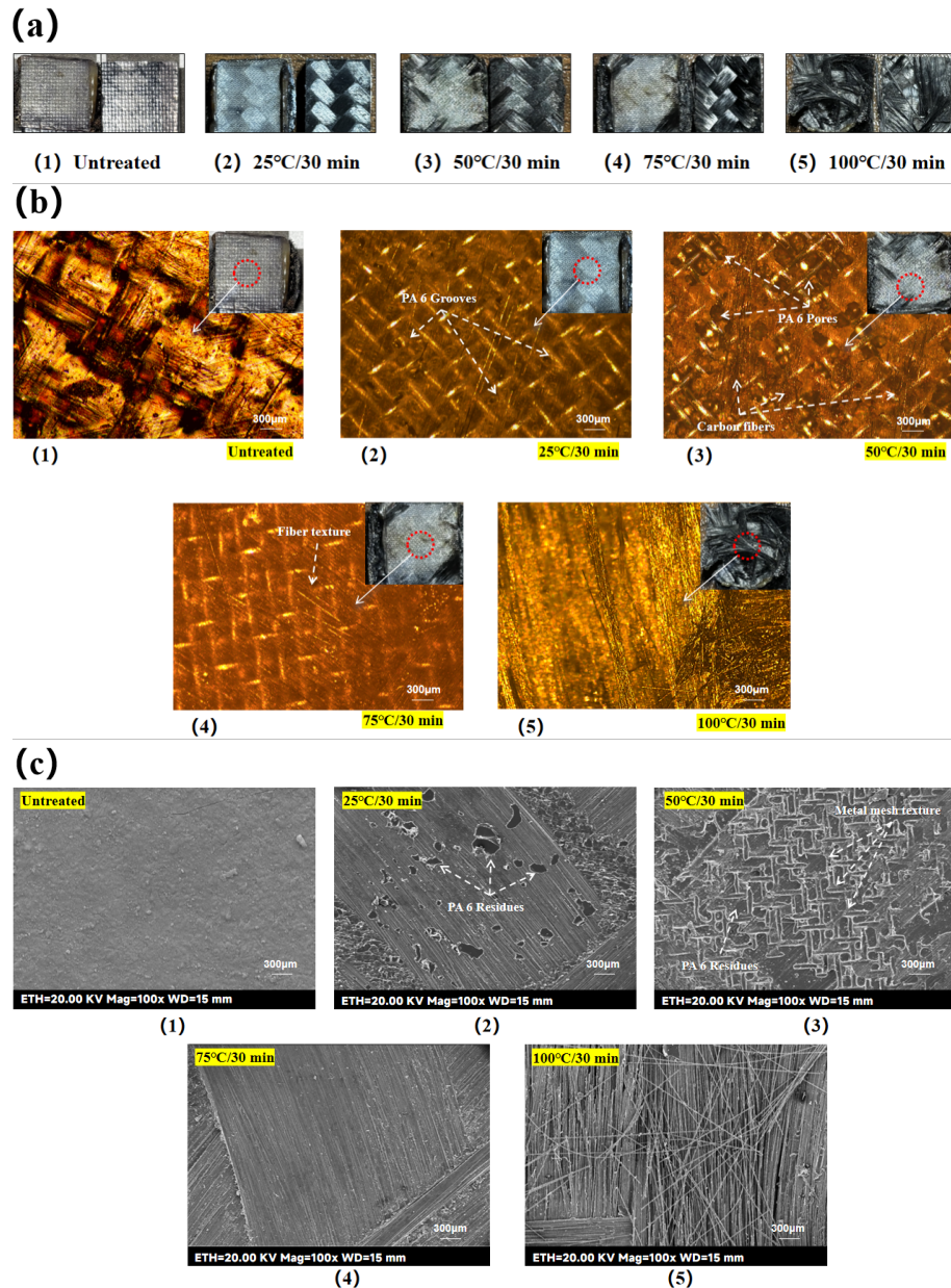
Figure 12. Morphological observation of welded joint failure interface (Temperature-variable experimental groups). (a)welded joint failure interface. (b)heating element failure interface. (c)laminate failure interface.
