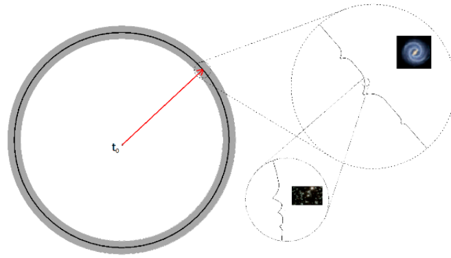
Figure 1. Visualisation of expansion wave cross section cutting through the expansion dimension (as shown by the radius) and a single space dimension (as shown by the circumference). This expansion wave started at time t_0 and has reached time t_1 signified by the dark black line. Two gravitationally distinct objects would expand away from each other in space as the expansion wave increases. Where objects have clumped together then dimples in the wavefront would show up as you zoom in. The thin black line shows the observable slice of time with the grey areas showing the possibility of matter existing outside of our observable time window.
