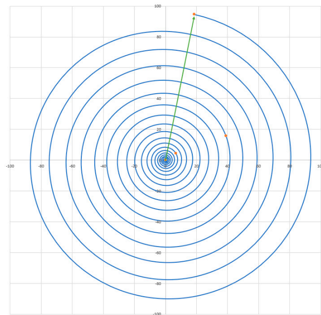
Figure 2. Visualisation of the spiral effect a light beam would take to reach us if it originated at the big bang in an expanding universe. Scale for both x and y is in Mpc. Distant, and therefore historic, objects in the universe, if observed from point A will appear as if on a spiral path reaching back to time zero. The above figure was generated using the complex decay model mentioned later in this paper against luminosity data of Betoule et al (2016) and Reis et al (1998). Points highlighted, emanating from the centre of the spiral are, respectively as follows: Time zero, most distant observed object at z of 11.09, Most distant fitted data point, Earth.
