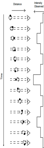
Figure 8. Visual representation of the effect of a photon spinning in time as it approaches an observer and the relative intensity observed at key points in the rotation.
