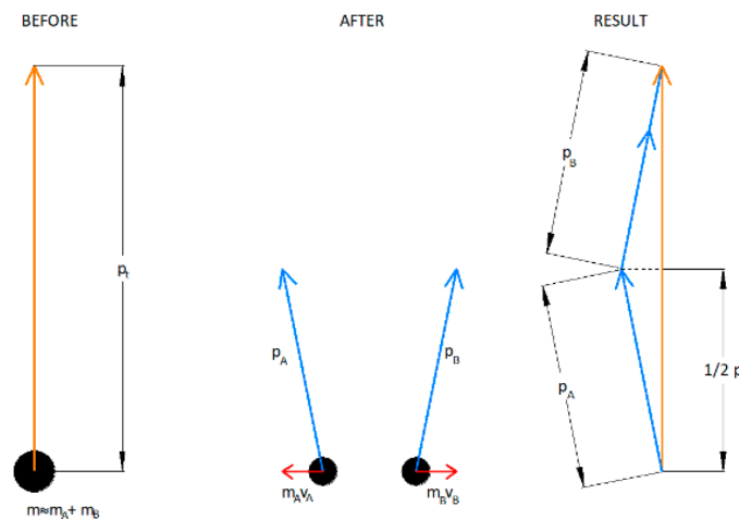
Figure 7. Explanatory figure to illustrate the effects of movement on the resultant momentum vectors in a single time (vertical) and space (horizontal) direction. The case considered here is one of an object breaking up and being pushed apart creating two identical mass objects moving in opposing directions with the same velocity.
