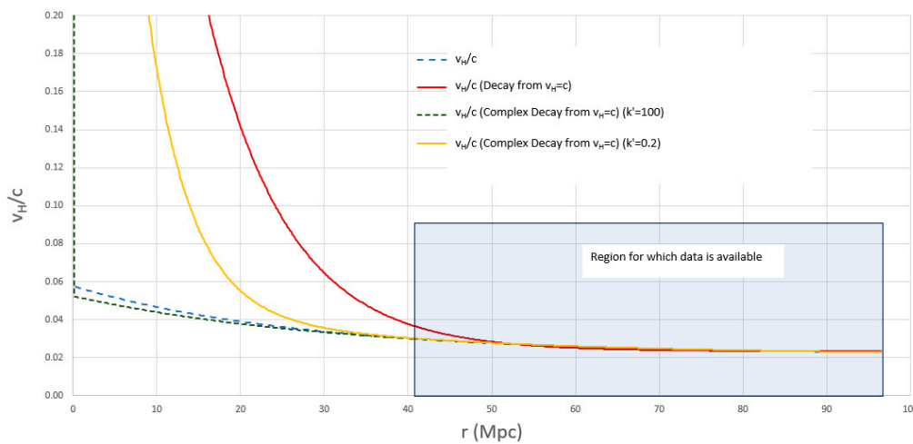
Figure 5. Exponential decay curves showing various possible fits.
