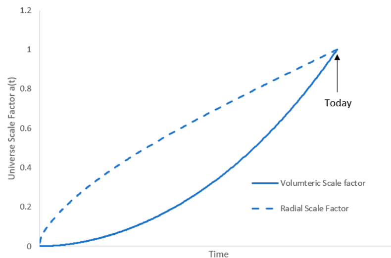
Figure 6. Volumetric and radial universe scale factor as a function of time using time expansion wave theory model calculations.
