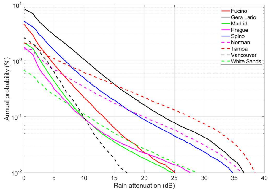
Figure 3. Annual probability distribution (%) P(A) of exceeding the value indicated in abscissa – 80 GHz, circular polarization, zenith paths – at the indicated sites. Spino d'Adda: continuous blue line; Gera Lario: continuous black line; Fucino: continuous red line; Madrid: continuous green line; Prague: continuous magenta line; Tampa: dashed red line; Norman: dashed magenta line; White Sands: dashed green line; Vancouver: dashed blue line.
