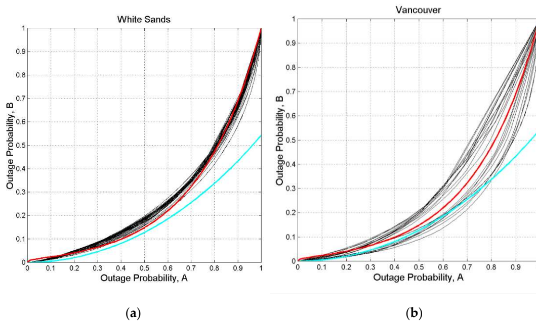
Figure A14. P_{S,B}(D) (y-axis) versus P_{S,A}(D) x-axis, 80 GHz, circular polarization, zenith paths: (a) White Sands, for thresholds from 0 to 40 dB; (b) Vancouver, for thresholds from 0 to 20 dB. The red line is drawn from Equation (3); the cyan line is drawn from Eq. (5).
