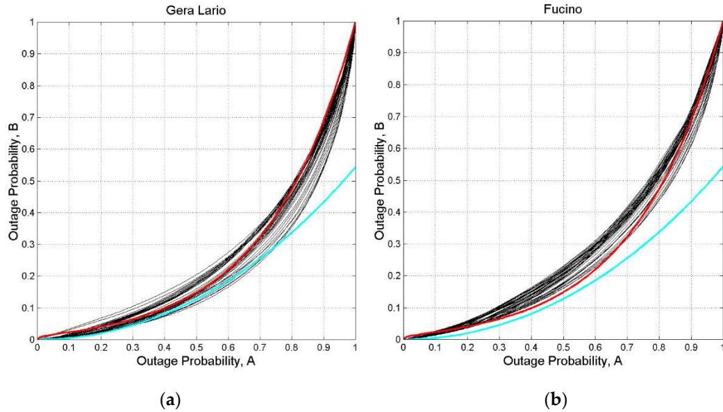
Figure A12 P_{S,B}(D) ( y -axis) versus P_{S,A}(D) ( x -axis), for thresholds from 0 to 40 dB, 80 GHz, circular polarization, zenith paths: (a) Gera Lario; (b) Fucino. The red line is drawn from Equation (3); the cyan line is drawn from Eq. (5).
