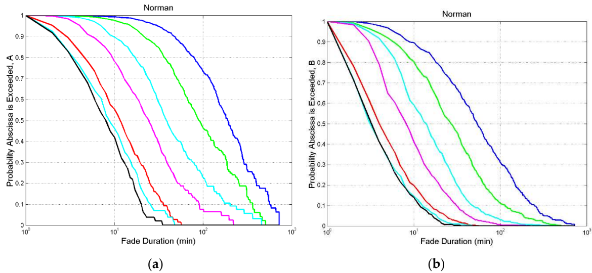
Figure A5. Norman. (a) Probability distribution P_{S,A}(D) of exceeding the value indicated in abscissa at the following thresholds: 0 dB, blue; 3 dB, green; 6 dB, cyan; 10 dB, magenta; 20 dB, red; 29~40 dB, cyan and black.; (b) P_{S,B}(D) , same legend.
