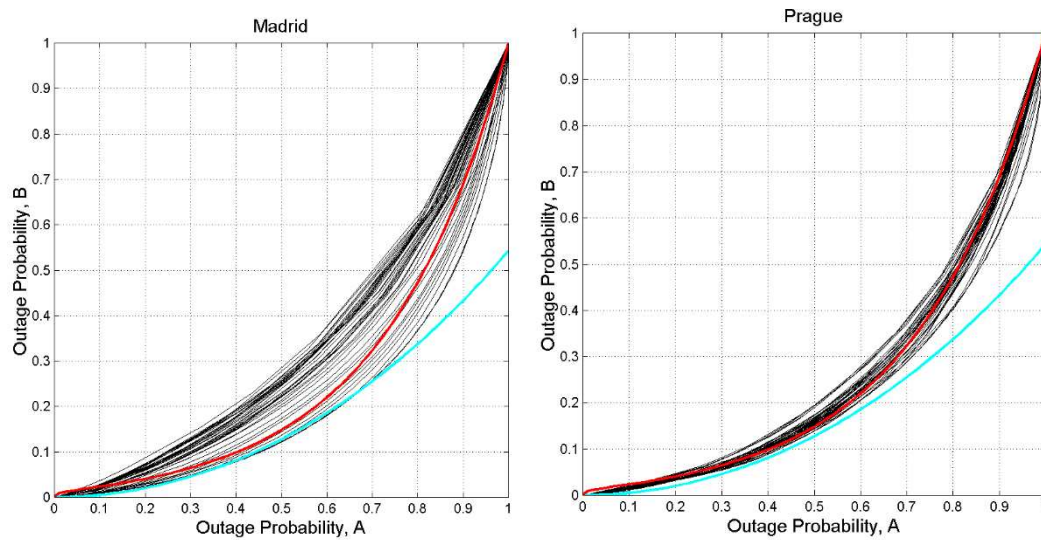
Figure A12. P_{S,B}(D) ( y -axis) versus P_{S,A}(D) ( x -axis), for thresholds from 0 to 40 dB, 80 GHz, circular polarization, zenith paths: (a) Madrid; (b) Prague. The red line is drawn from Equation (3); the cyan line is drawn from Eq. (5).
