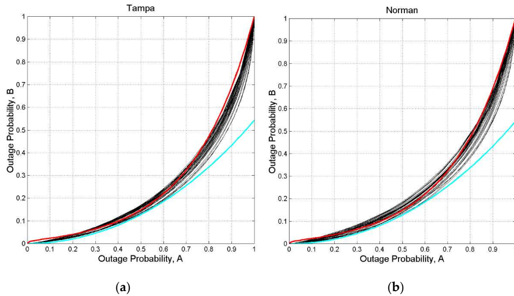
Figure A13. P_{S,B}(D) (y-axis) versus P_{S,A}(D) x-axis, for thresholds from 0 to 40 dB, 80 GHz, circular polarization, zenith paths: (a) Tampa; (b) Norman. The red line is drawn from Equation (3); the cyan line is drawn from Eq. (5).
