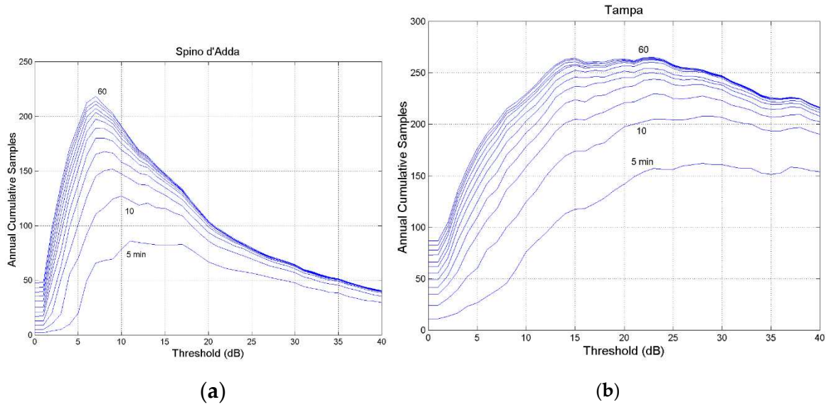
Figure 8. Annual cumulative number of outage occurrences at the threshold indicated in abscissa, 80 GHz, circular polarization, zenith paths: (a), at Spino d'Adda; (b) Tampa. The continuous lines are drawn at equal fade duration, in 5-min steps from \tau = 5 min to \tau = 60 . The y-axis has different range.
