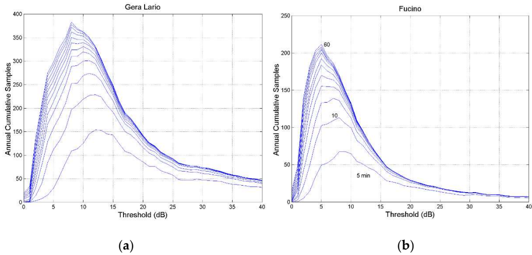
Figure A8. Annual cumulative number of outage occurrences at the threshold indicated in abscissa, 80 GHz, circular polarization, zenith paths: (a) Gera Lario; (b) Fucino. The lines refer to constant fade duration, in 5-min steps, from \tau = 5 min to \tau = 60 . The y -axis has different range.
