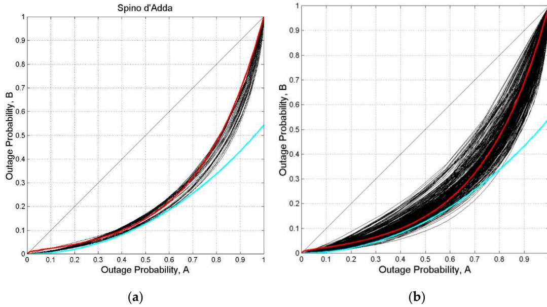
Figure 9. P_{S,B}(D) ( y -axis) versus P_{S,A}(D) ( x -axis), for thresholds from 0 to 40 dB, 80 GHz. The continuous red line is drawn from Equation (3); the continuous cyan line is drawn from Eq. (5). (a) Spino d'Adda; (b) all sites.
