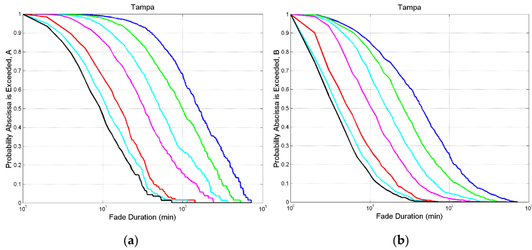
Figure 5. Tampa. (a) Probability distribution P_{S,A}(D) of exceeding the value indicated in abscissa at the following thresholds: 0 dB, blue; 3 dB, green; 6 dB, cyan; 10 dB, magenta; 20 dB, red; 29~40 dB, cyan and black.; (b) P_{S,B}(D) , same legend.
