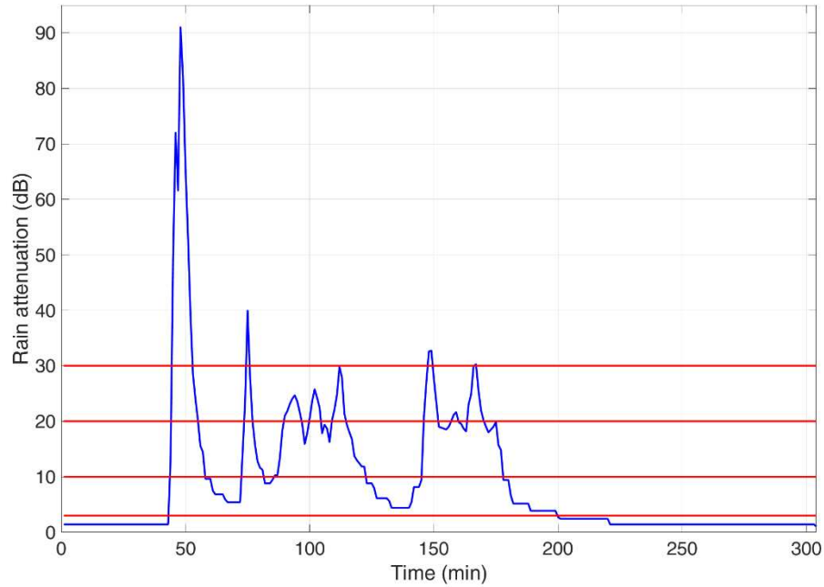
Figure 1. Rain attenuation time series, 80 GHz circular polarization, zenith path, at Spino d’Adda, 6 May 2000, rain event starts at 17.30 local time. The red lines are drawn at thresholds 3, 10, 20 and 30 dB.
