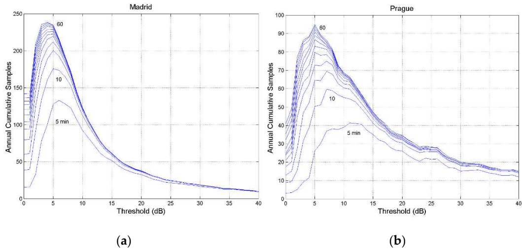
Figure A9. Annual cumulative number of outage occurrences at the threshold indicated in abscissa, 80 GHz, circular polarization, zenith paths: (a) Madrid; (b) Prague. The lines refer to constant fade duration, in 5-min steps, from \tau = 5 min to \tau = 60 . The y-axis has different range.
