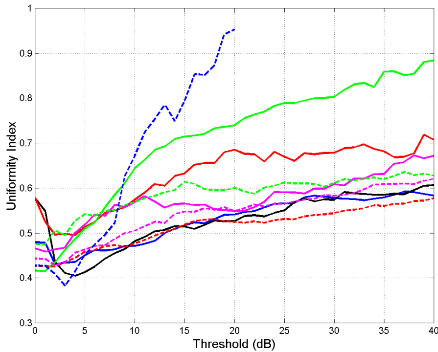
Figure 10. Uniformity index versus the threshold indicated in abscissa at the indicated sites. Spino d'Adda: continuous blue line; Gera Lario: continuous black line; Fucino: continuous red line; Madrid: continuous green line; Prague: continuous magenta line; Tampa: dashed red line; Norman: dashed magenta line; White Sands: dashed green line; Vancouver: dashed blue line.
