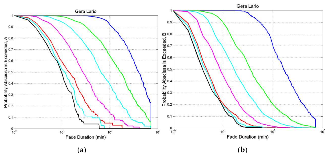
Figure A1. Gera Lario. (a) Probability distribution P_{S,A}(D) of exceeding the value indicated in abscissa at the following thresholds: 0 dB, blue; 3 dB, green; 6 dB, cyan; 10 dB, magenta; 20 dB, red; 29~40 dB, cyan and black.; (b) P_{S,B}(D) , same legend.
