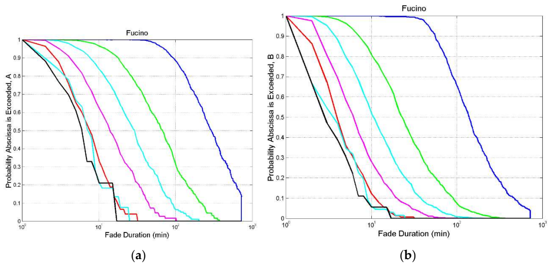
Figure A2. Fucino. (a) Probability distribution P_{S,A}(D) of exceeding the value indicated in abscissa at the following thresholds: 0 dB, blue; 3 dB, green; 6 dB, cyan; 10 dB, magenta; 20 dB, red; 29~40 dB, cyan and black.; (b) P_{S,B}(D) , same legend.
