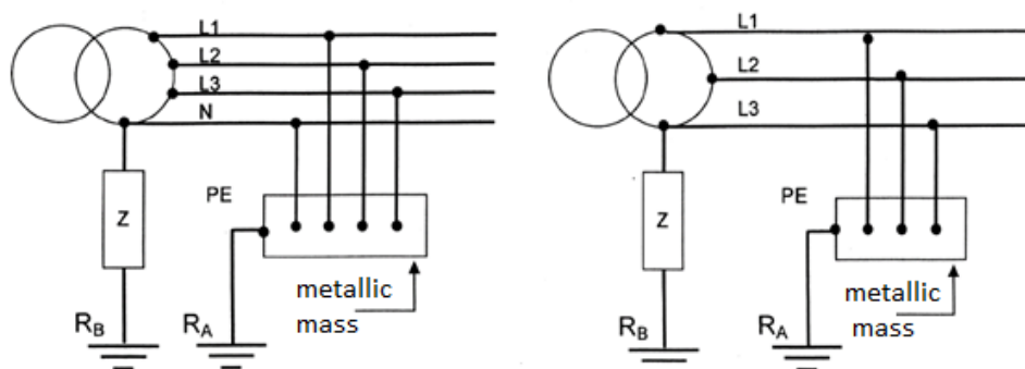
Figure 14. IT Grounding Scheme, with and without distributed neutral conductor. [19].
