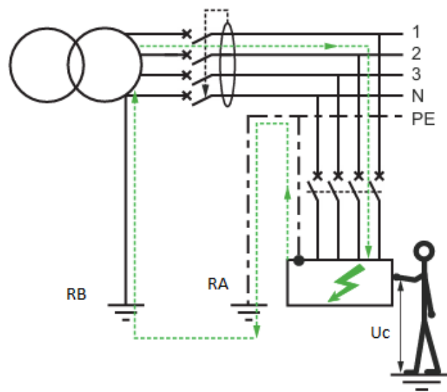
Figure 9. TT scheme: fault loop path. [20].
