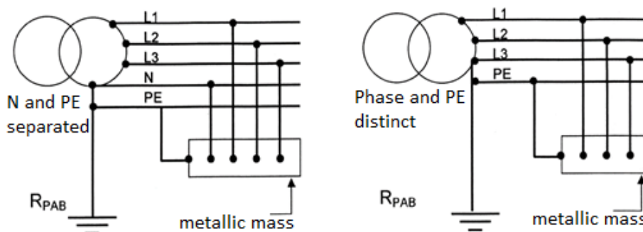
Figure 11. TN-S grounding scheme. With and without the presence of a neutral in the supply.
