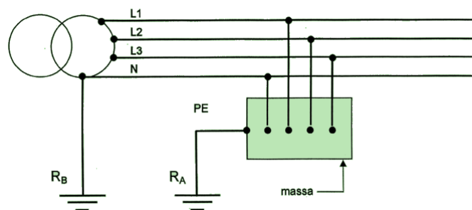
Figure 8. TT grounding scheme [19].
