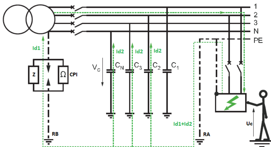
Figure 15. First fault loop in an IT type ELT. [20].
