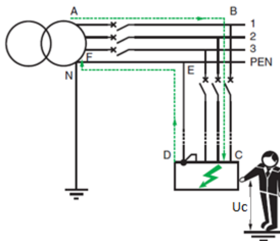
Figure 13. Fault loop in a TN-C type ELT. [20].
