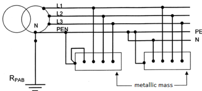
Figure 12. TN-C-S grounding scheme. [19].
