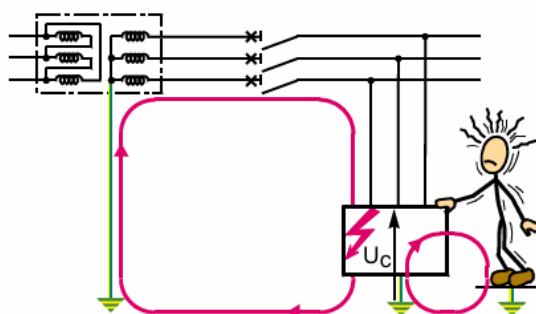
Figure 7. Electrical diagram of indirect contact: electrical contact of a person with a body accidentally placed under voltage [20].
