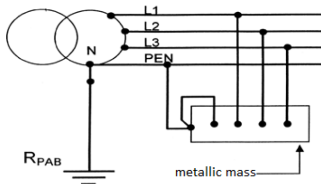
Figure 10. TN-C grounding scheme. [19].
