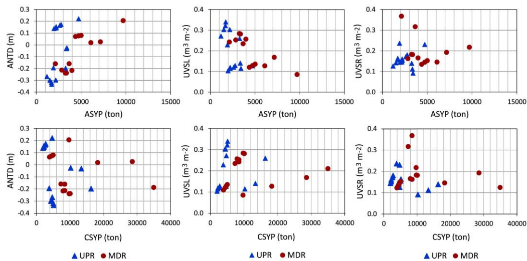
Figure 12. Average and cumulative sediment yield per PECP sub-period (ASYP and CSYP, respectively), estimated at the entrance of the upper (UPR) and middle (MDR) channel reaches, versus ANTD, UVSL, and UVSR.
