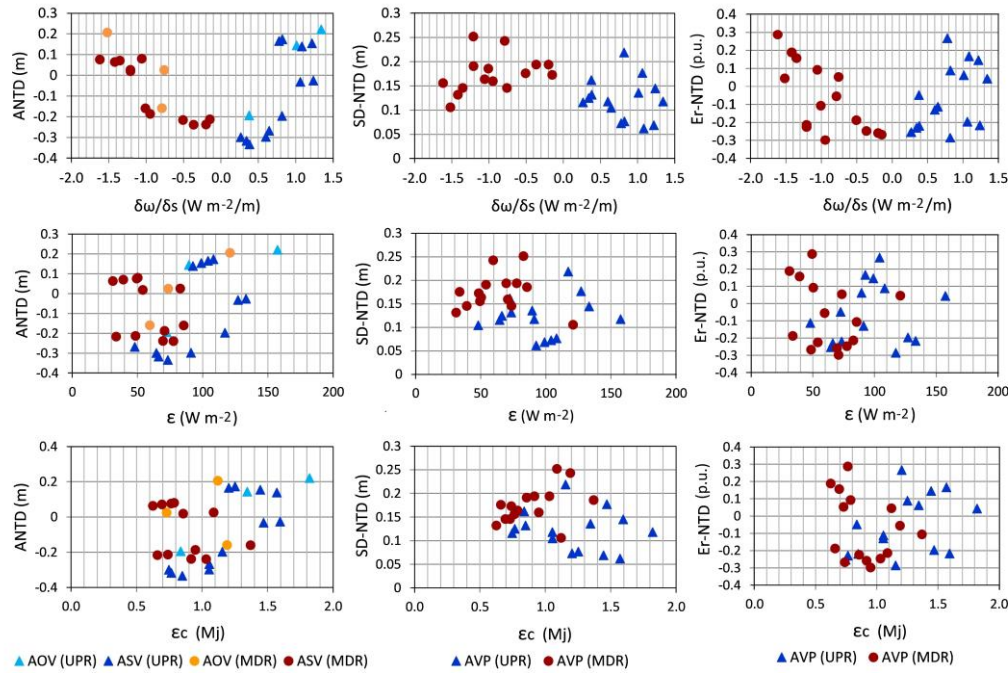
Figure 13. Values of stream power variables ( \partial\omega/\partial s , \epsilon , and \epsilon_c ) versus parameters related to the net thickness difference (ANTD, SD-NTD, and Er-NTD). AVP = average values per PCEP sub-period; AOV and ASV are, respectively, the observed and simulated mean values for each sub-period. Er-NTD expressed per unit (p.u.).
