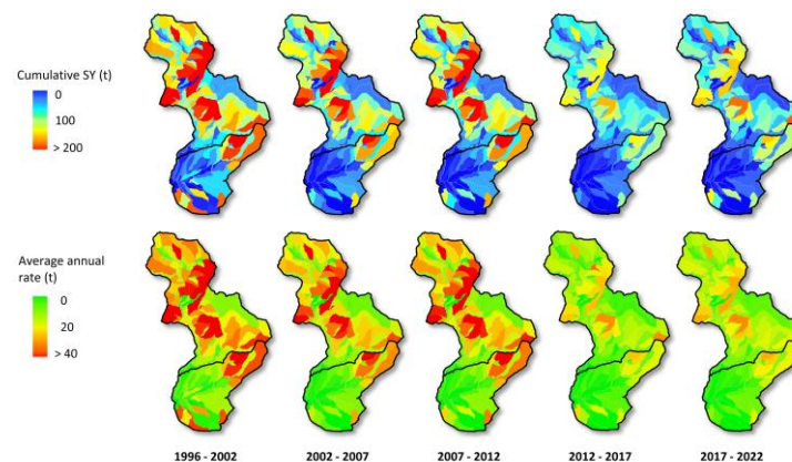
Figure 4. Spatial distribution of the cumulative (CSY) and average (ASY) sediment yields, estimated using GeoWEPP for retroactive five-year periods in the middle and upper sub-catchments of the Azohía Rambla.
