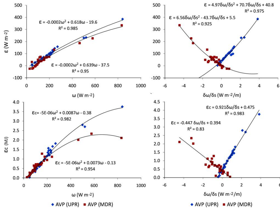
Figure 11. \omega - \epsilon and \omega - \epsilon_c relationships (left-hand graphs) and \partial\omega/\partial s - \epsilon and \partial\omega/\partial s - \epsilon_c relationships (right-hand graphs), at a significance level (p-value) < 0.05. AVP = average values per PCEP sub-period.
