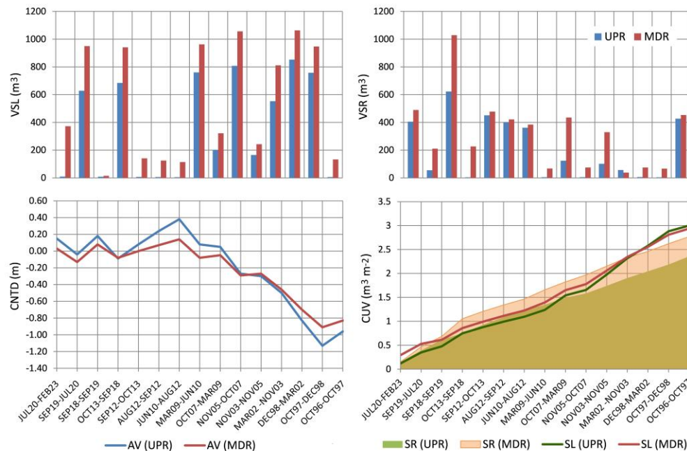
Figure 8. The upper histograms represent the total volumes of lowered (VSL) and raised (VSR) surfaces for all PECPs; at the bottom, the left-hand figure shows the cumulative net thickness difference (CNTD), and the right-hand figure shows the profiles depicting the cumulative unit volume (CUV) of surface lowering (SL) and raising (SR) for the same sub-periods and channel reaches. AV = average values for each sub-period.
