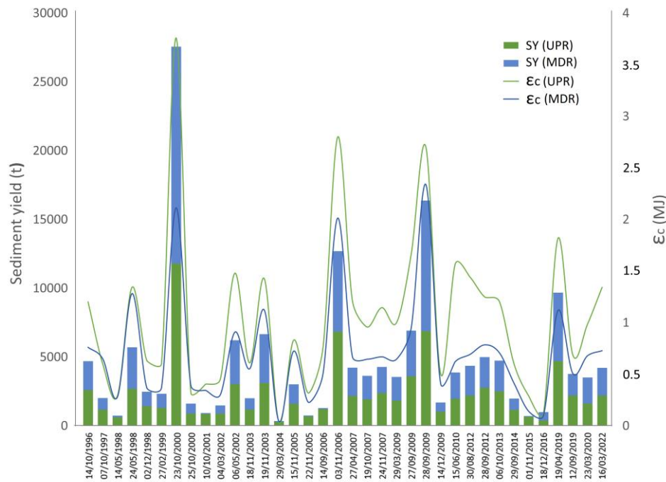
Figure 15. Comparison of the sediment yield and excess accumulated energy estimated for each of the events that occurred in the period 1996-2022 along UPR and MDR.
