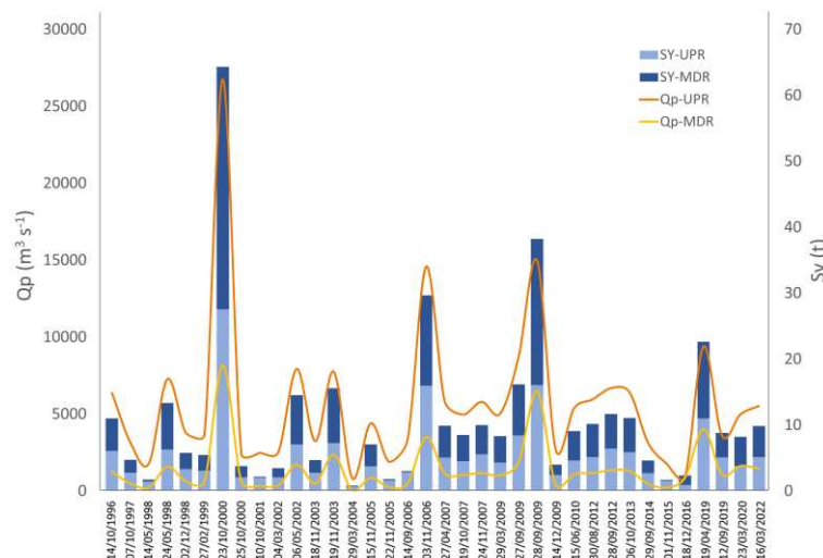
Figure 5. Peak discharges and potential average sediment outputs estimated with GeoWEPP for the flow events that occurred during the period 1996-2022.
