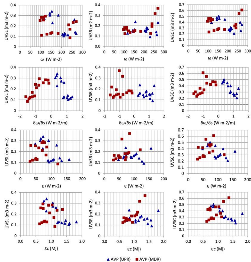
Figure 14. Values of stream power variables ( \partial\omega/\partial s , \varepsilon , and \varepsilon_c ) versus unit volume of surface lowering (UVSL), raising (UVSR), and changing (UVSC). The values are averaged per PCEP sub-period (AVP).
