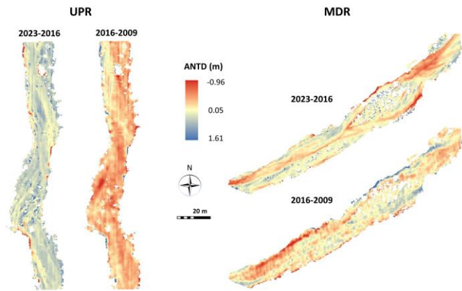
Figure 6. DoDs resulting from the difference between the DEMs derived from the NPAO 2009 and 2016 LiDAR point clouds (0.5 m per pixel) and those generated with SfM-MVS in 2018 and 2023 after being converted to the same resolution. Upper and Middle RCRs.
