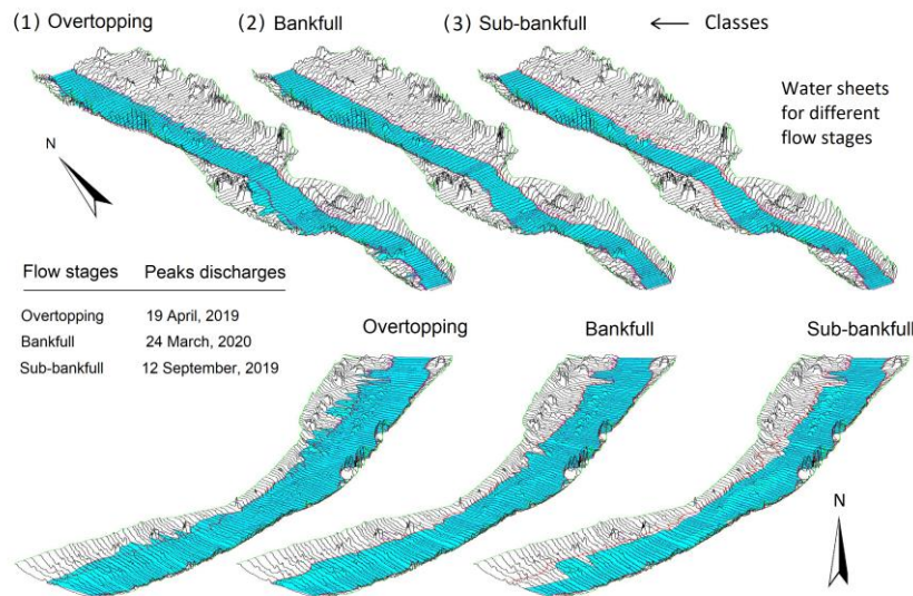
Figure 3. Water sheets for the flow stages defined for classes 1 (overbank flow), 2 (bankfull discharge), and 3 (sub-bankfull discharge), obtained using HEC-RAS from field survey data.
