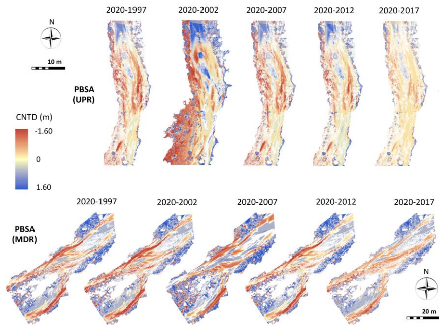
Figure 9. Cumulative HRDODs retrospectively simulated for the period 1997-2020 in the upper and middle RCRs, combining pre- and post-event ECs with TLS-derived DTMs over the monitoring stage (2018-2020).
