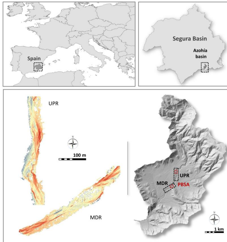
Figure 1. Location of the study area (Azohía Rambla basin) in southeastern Spain, and indication of the monitored channel reaches (upper and middle RCRs and their respective PBSAs).
