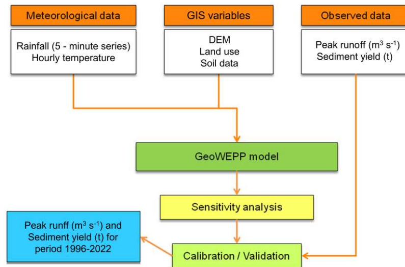
Figure 2. Flowchart displaying the steps in the event-scale GeoWEPP implementation process for the period 1996-2022. Process flow diagram applied to the sub-catchment of each RCR.
