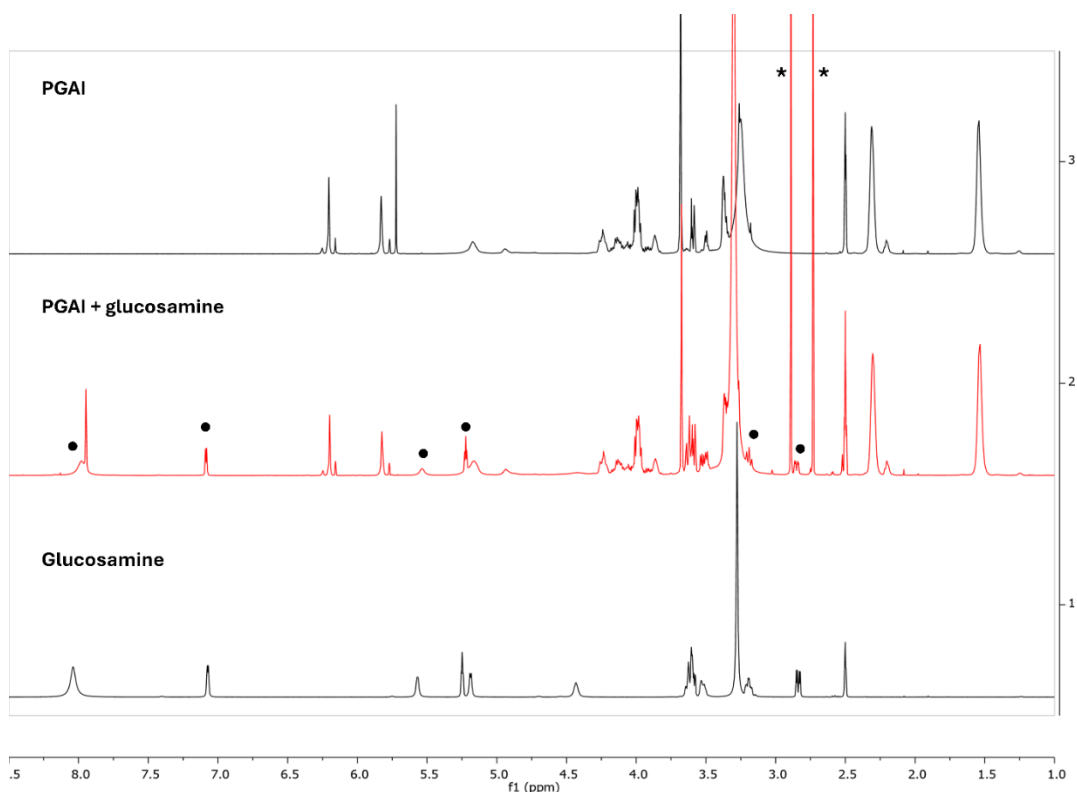
Figure 10. ^1\text{H} NMR spectra (500 MHz, \text{DMSO-d}_6 , 45^\circ\text{C} ) of the PGAI terpolymer (above), its reaction product with glucosamine experiment 4 (middle) and glucosamine used for the reaction (bottom). Black dots indicate signals of glucosamine present in the reaction product spectrum. Chemical shifts are referred to the DMSO residual signal (2.5 ppm).
