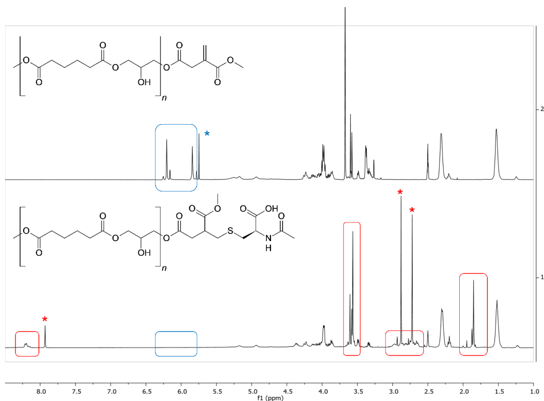
Figure 7. Comparison between the ^1\text{H} NMR spectra (400 MHz, \text{DMSO-d}_6 , 25^\circ\text{C} ) of the PGAI terpolymer (above) and its reaction product with N-acetyl cysteine (below). In red, signals of NAC in the product spectrum; in blue, signals of the vinyl protons of DMI. Blue asterisks indicate DCM impurities; red asterisks indicate DMF impurities. Chemical shifts are referred to the DMSO residual signal (2.5 ppm).
