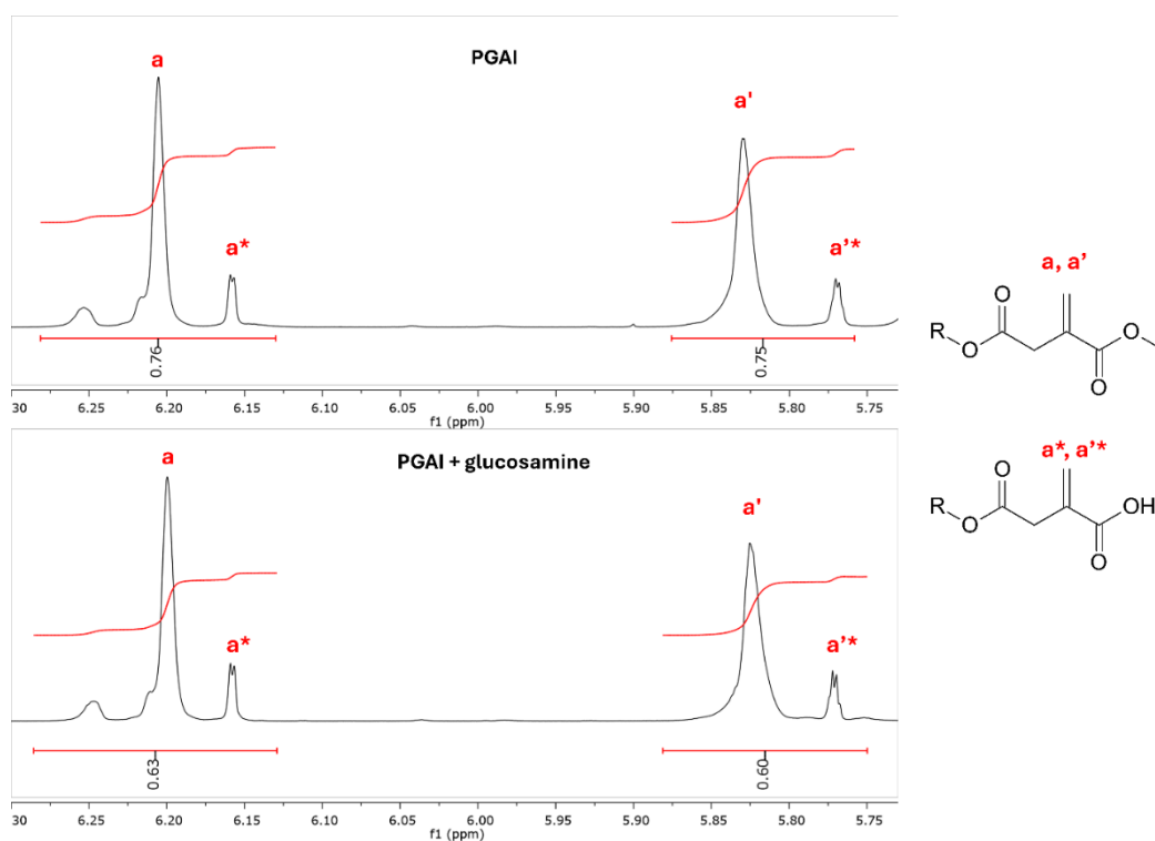
Figure 11. Enlargement of the range between 6.30 and 5.75 ppm of the ^1\text{H} NMR spectra of the PGAI terpolymer (above), and its reaction product with glucosamine (below). Integral areas were normalized referring to the signal at 1.5 ppm (4 H, aliphatic protons adipic acid).
