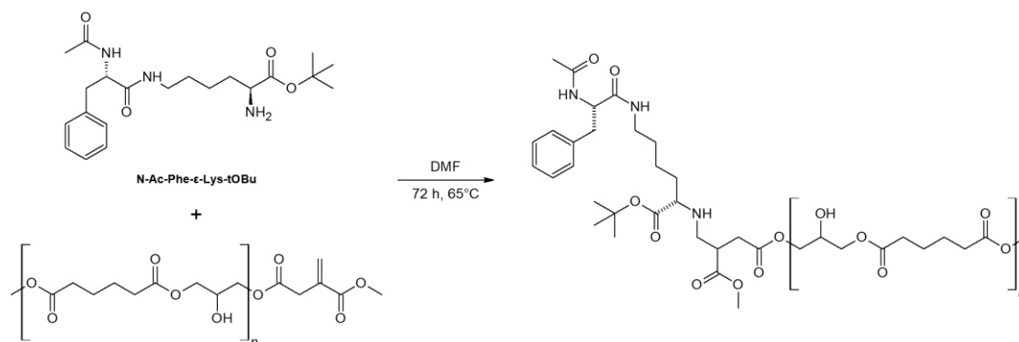
Scheme 3. Aza-Michael addition of N-Ac-Phe-ε-Lys-tOBu to the vinyl moiety of PGAI.
