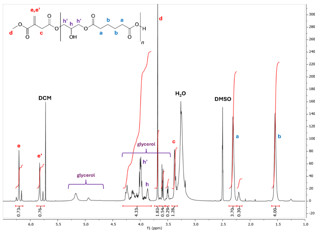
Figure 5. ^1\text{H} NMR spectrum (500 MHz, \text{DMSO-d}_6 ) for the PGAI terpolymer after purification. Labeled in blue, signals of the adipic acid monomer; in red, signals of the dimethyl itaconate monomer; in purple, signals of glycerol; in black, solvent impurities.
