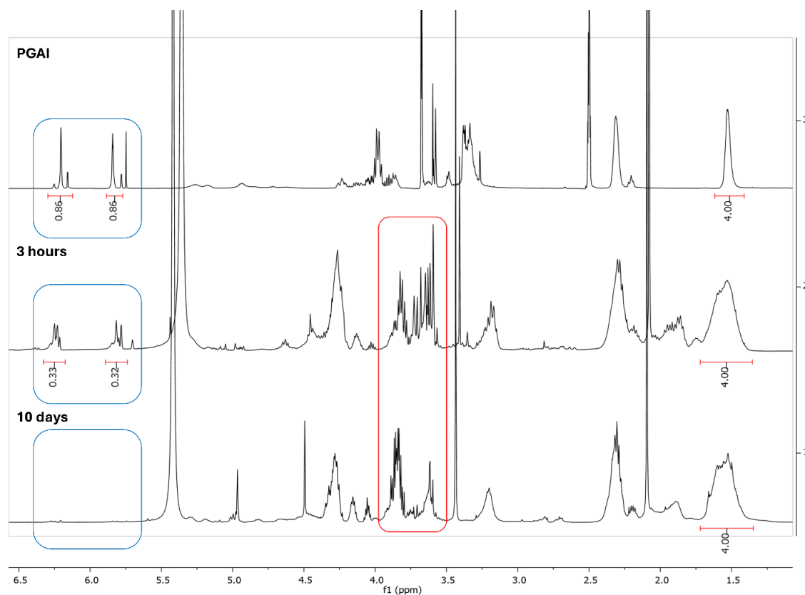
Figure 9. 1 H NMR spectra (500 MHz) of the PGAI terpolymer (above) and the reaction mixture of PGAI with trilycine after 3 hours (middle) and 10 days (bottom). The spectrum of PGAI was obtained in DMSO-d 6 , while spectra of the reaction mixture with trilycine were acquired in a 1:1 D 2 O/pyridine-d 5 mixture. The spectra chemical shifts are referred to the signal of adipic acid at 1.53 ppm.
