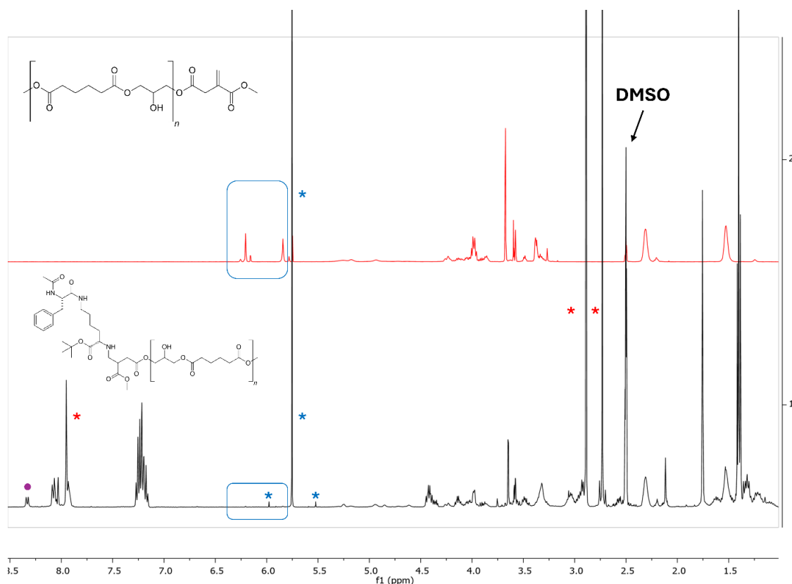
Figure 8. Comparison between the ^1\text{H} NMR spectra (400 MHz, \text{DMSO-d}_6 ) of the PGAI terpolymer (above) and its reaction product with N-Ac-Phe- \epsilon -Lys-OtBu (below). In the blue square, signals of the vinyl protons of DMI. Blue asterisks indicate DCM impurities; red asterisks indicate DMI impurities.
