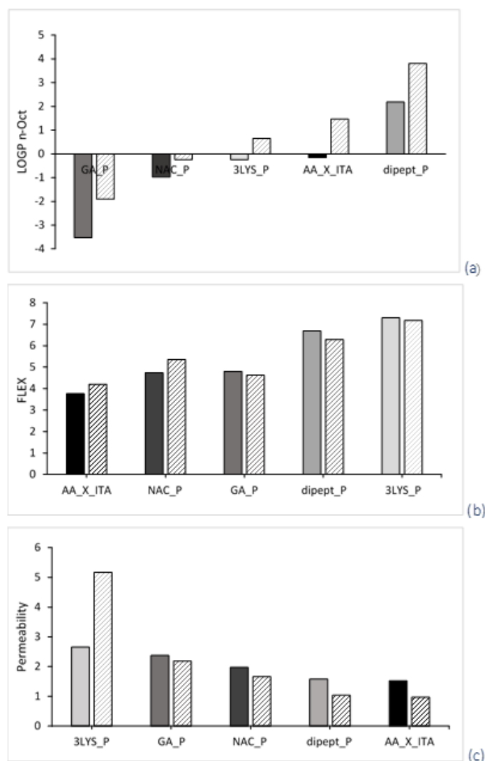
Figure 3. Predicted values of the logarithm of the partition coefficient between 1-octanol and water (a), flexibility (b) and permeability (c) of the functionalized oligoesters. For each set of data, the column in darker solid gray color refers to AA-GLY-ITA whereas the column with a diagonal striped pattern refers to AA-BDO-ITA. Legend for the oligoesters functionalized with the biomolecules: Lys-Lys-Lys (3LYS_P), N-acetylcysteine (NAC_P), N-Ac-Phe- \epsilon -Lys-OtBu (dipept_P) and glucosamine (GA_P). AA_X_ITA are the non-functionalized oligoesters.
