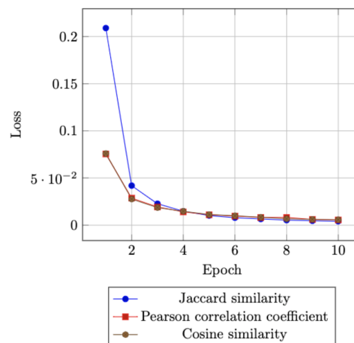
Figure 5. Training loss curves
