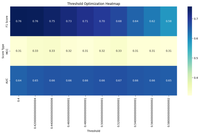
Figure 2. Heatmap of Threshold Selection for Jaccard similarity.
