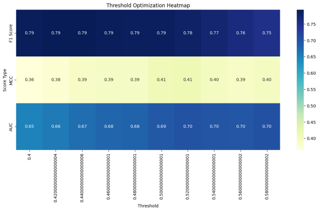
Figure 3. Heatmap of Threshold Selection for Pearson correlation coefficient
