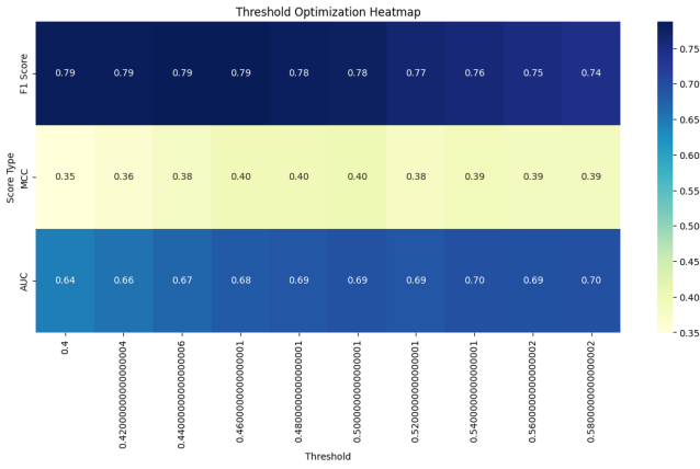
Figure 4. Heatmap of Threshold Selection for Cosine similarity
