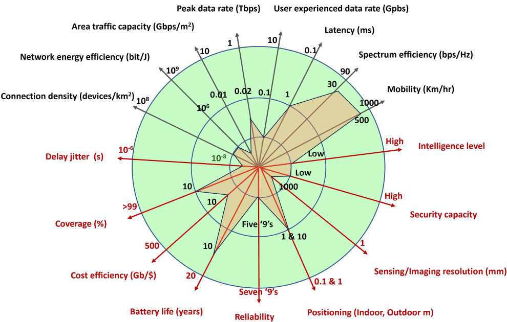
Figure 4. 6G key performance indicators (KPIs). Adopted from [17].
