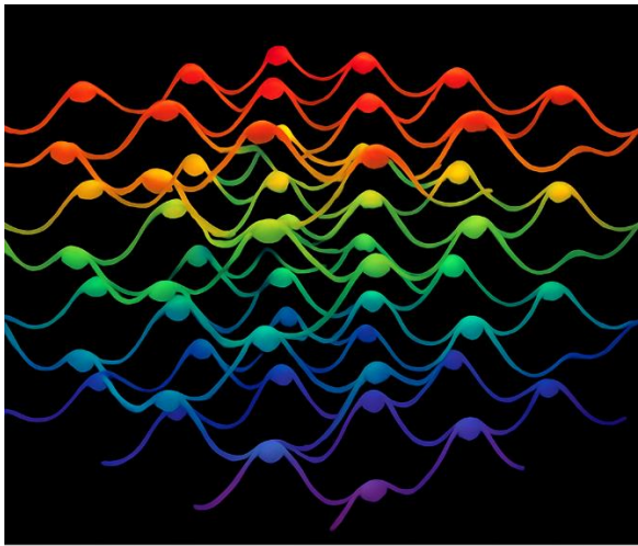
Figure 6. Final configuration of the TT resonant network. Layered representation of TT-based spatial nodes coupled via four-dimensional entanglement. Frequency and orientation modulate the spatial topology under the parameter \theta , forming a continuous non-Euclidean harmonic field.
