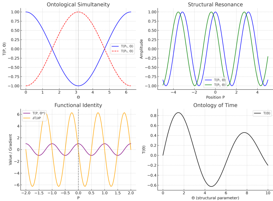
Figure 3. Mathematical illustrations of Trigonotetary concepts. From left to right: ontological simultaneity, structural resonance, functional identity, and the ontology of time. Each subpanel represents a distinct mathematical behavior derived from T(\mathbf{P}, \Theta) .
