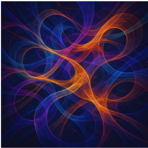
Figure 5. Entangled mesh generated by phase synchronization. Visualization of the TT field showing continuous spatial curvature and harmonic twisting across dimensions. Phase entanglement modulates structural proximity between nodes, forming a dense network.
