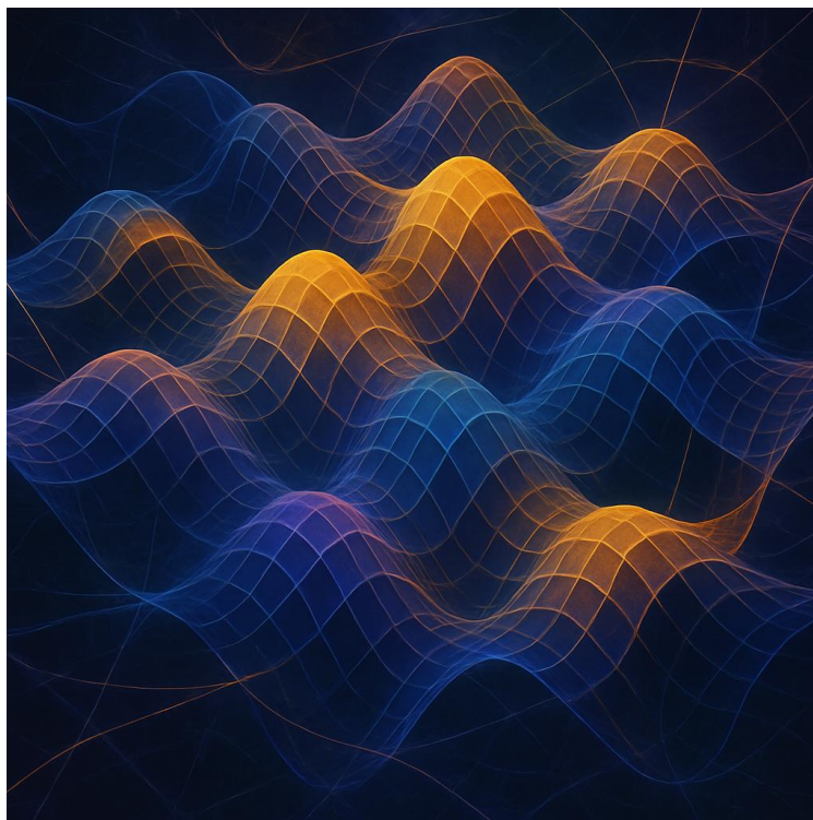
Figure 2. Multidimensional harmonic network generated by the TT function. Computer-generated rendering showing layered wave networks modulated by the fourth-dimensional parameter \theta . The amplitude and frequency variation define topological configurations based on the superposition of harmonic components.
