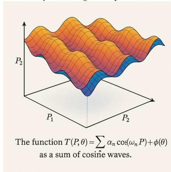
Figure 1. Trigonotetary function in two dimensions. Graphical representation of the function T(\mathbf{P}, \theta) = \sum_n \alpha_n \cos(\langle \mathbf{w}_n, \mathbf{P} \rangle + \varphi_n(\theta)) , showing a superposition of cosine waves across two spatial dimensions as the entanglement parameter \theta varies.
