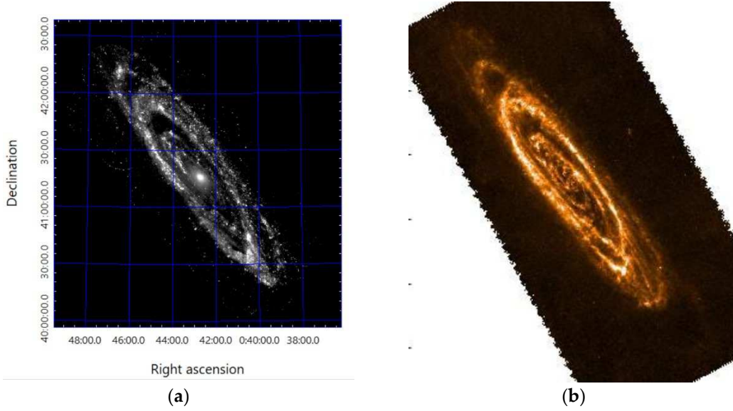
Figure 2. Images of M31 at ultraviolet and infrared wavelengths. (a) The 148 nm image of M31 [6]. (b) The far infrared 250 micron image of M31 from the Hershel SPIRE instrument [7]. The ultraviolet and far infrared images closely trace the spiral arms of M31.
