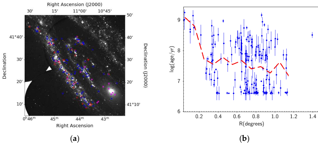
Figure 3. (a) Positions and ages of the clusters in the northeast disk and bulge of M31 studied by [32]. \text{Log}(\text{age}/\text{yr}) values are shown by the size of the circles with radius proportional to \log(\text{age}/\text{yr}) and
