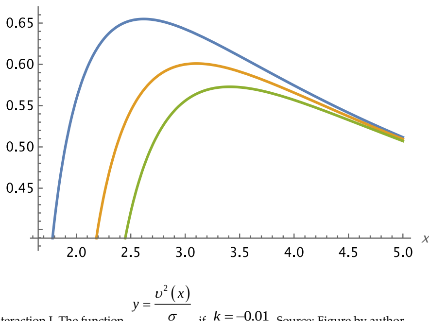
Figure 4.1. Interaction I. The function y = \frac{v^2(x)}{\sigma} if k = -0.01 . Source: Figure by author.
