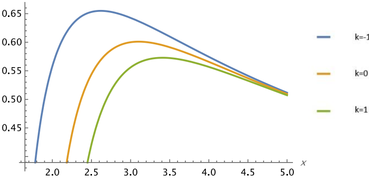
Figure 4.24. Interaction IV. The graph of the function y = \frac{v(x)}{\sqrt{\sigma}} , if k = -1 , for large values of x . Source: Figure by author.
