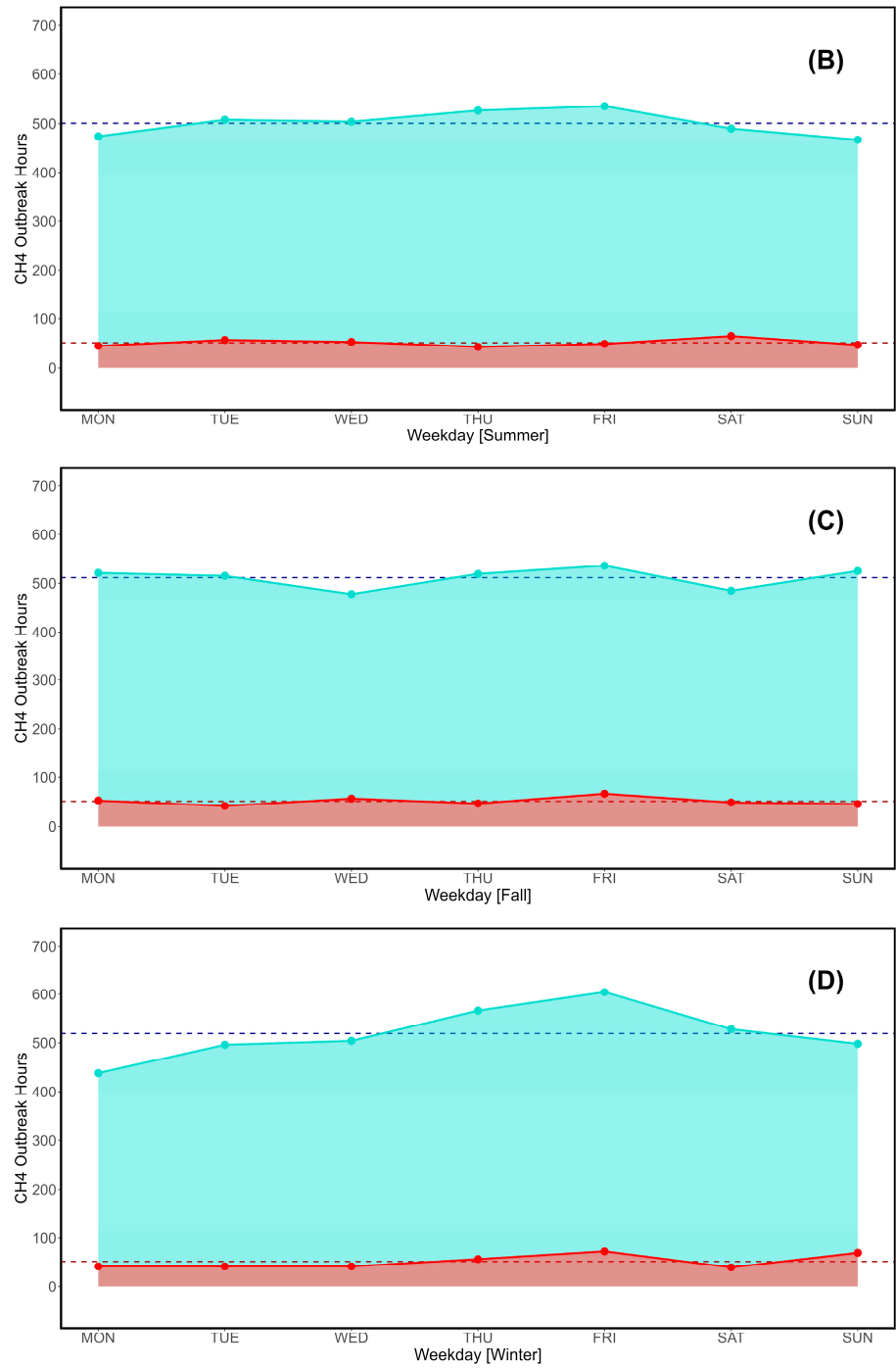
Figure 9. Seasonal variations of CH 4 (ppb) in terms of outbreak hours of occurrence (Q3 and top 2.5% interval thresholds). A: Spring; B: Summer; C: Fall; D: Winter.
