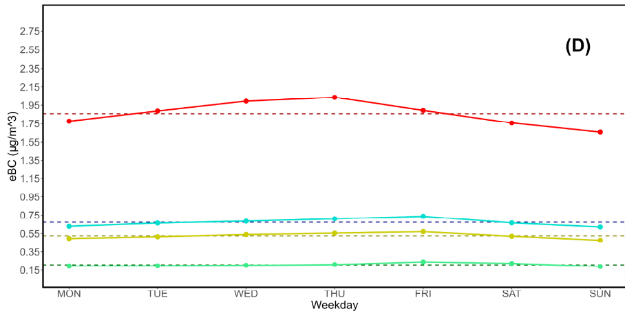
Figure 2. Q1, mean, Q3 and top 2.5% values for all four parameters (A: CO; B: CO 2 ; C: CH 4 ; D: eBC), calculated over the entire observation period (2016-2022). Dashed parallel lines show average values for each parameter and help to visualize possible differences between weekdays. Please note that the vertical axes are distinct for each parameter. The legend is shown in Figure 2A.
