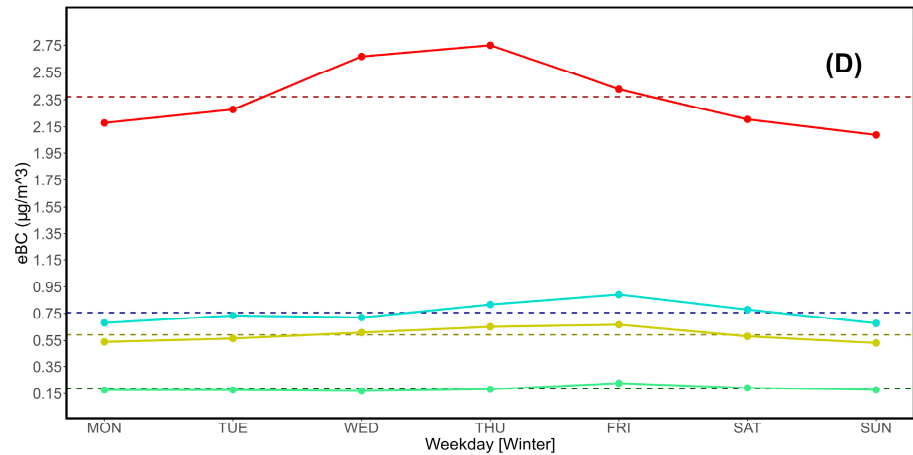
Figure 6. Seasonal variations of eBC ( \mu\text{g}/\text{m}^3 ). A: Spring; B: Summer; C: Fall; D: Winter.
