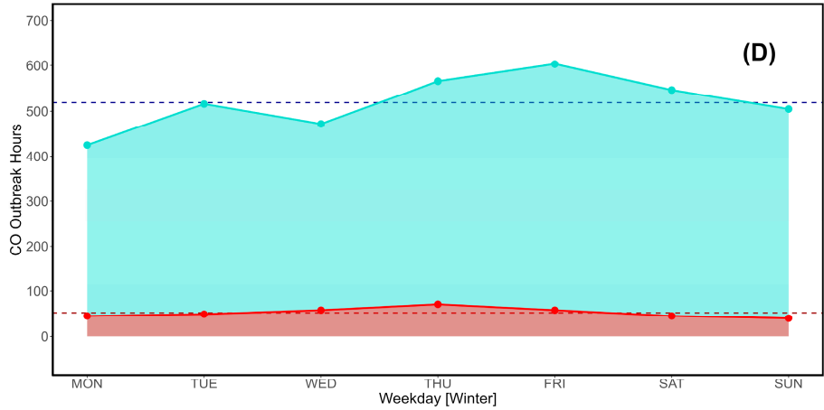
Figure 7. Seasonal variations of CO (ppb) in terms of outbreak hours of occurrence (Q3 and top 2.5% interval thresholds). A: Spring; B: Summer; C: Fall; D: Winter.
