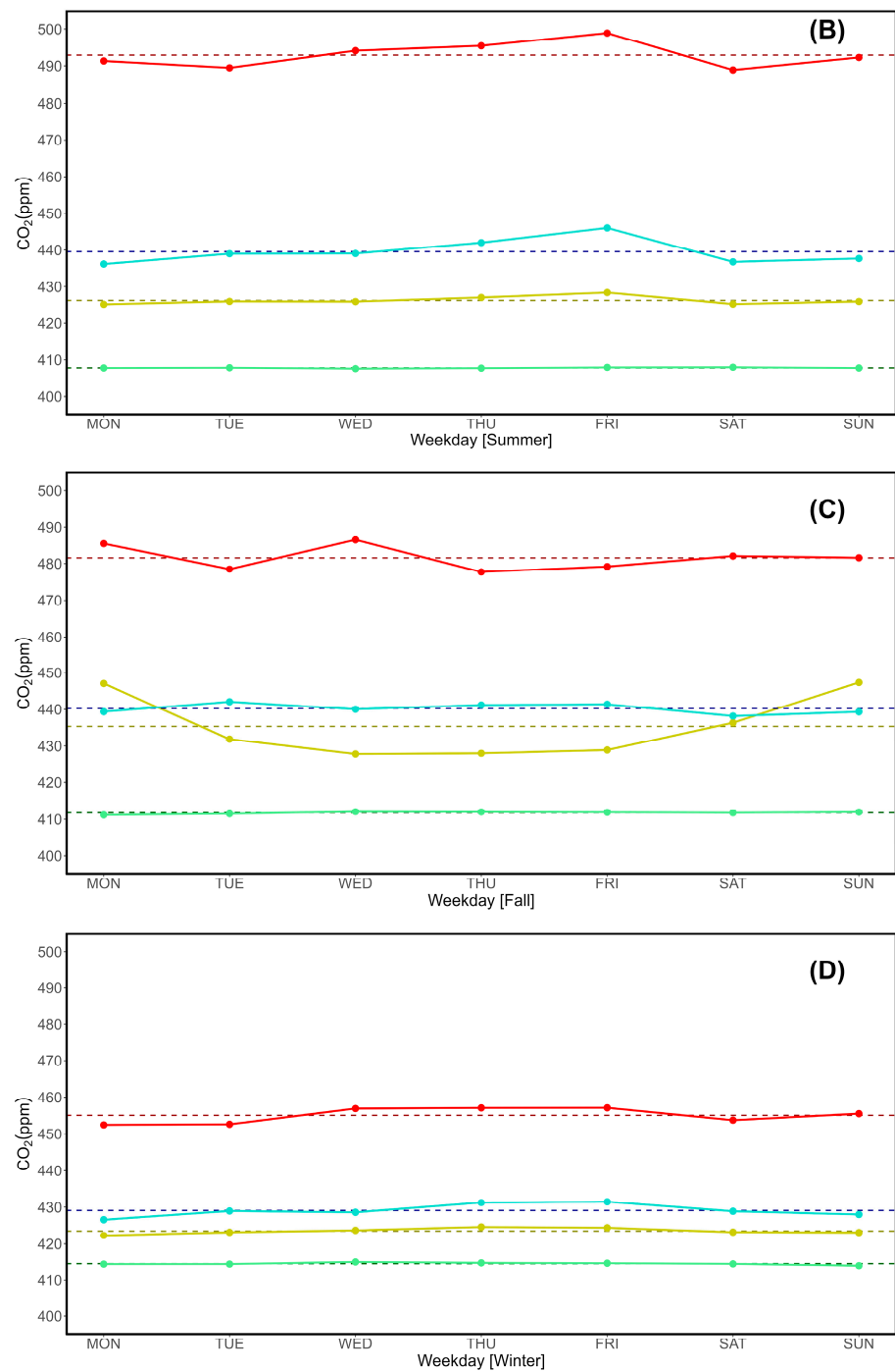
Figure 4. Seasonal variations of CO 2 (ppm). A: Spring; B: Summer; C: Fall; D: Winter.
