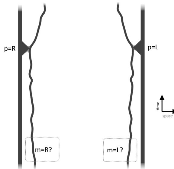
Figure 2. Spacetime structures involving alleged non-machines (thin lines) interacting with a ‘perturber’ (thick lines) in one of its two modes ( R and L ). Note the energy-momentum bridge necessarily connecting the two. Seen from this perspective, future memory should not be attributed to any single non-machine type independently of an experimental context.
