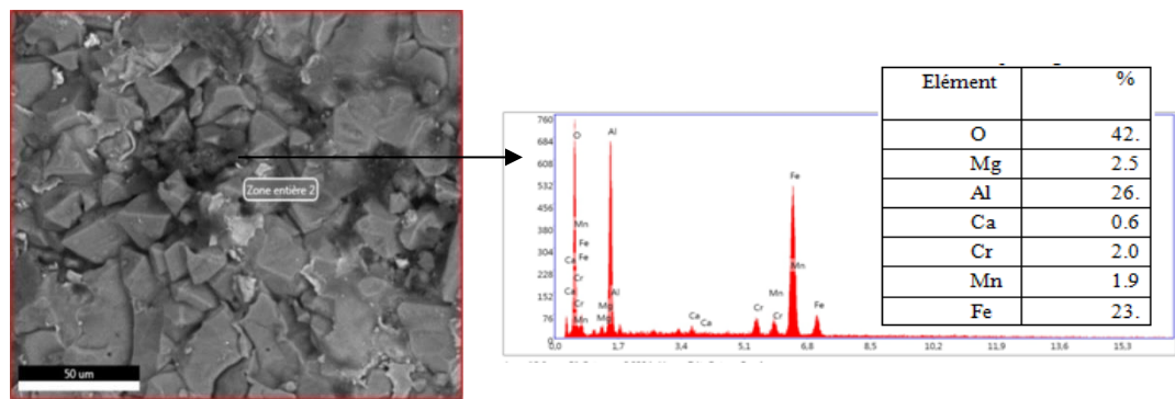
Figure 12. SEM image and chemical composition after EDSLeft side.
