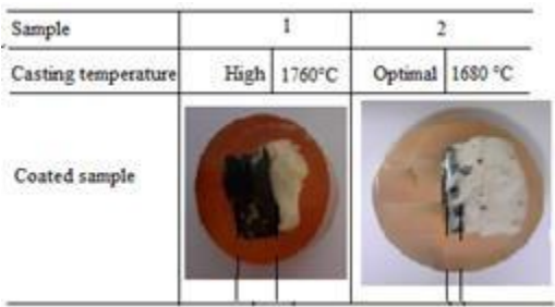
Figure 6. Samples prepared to measure interfacial indentation.
