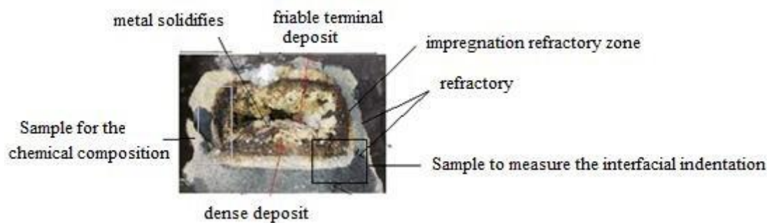
View of a cross section of the lower part of a nozzle
