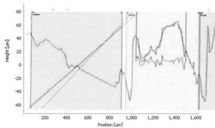
Figure 15. Roughness profile of the sample for 75 minutes of holding 750°C.
