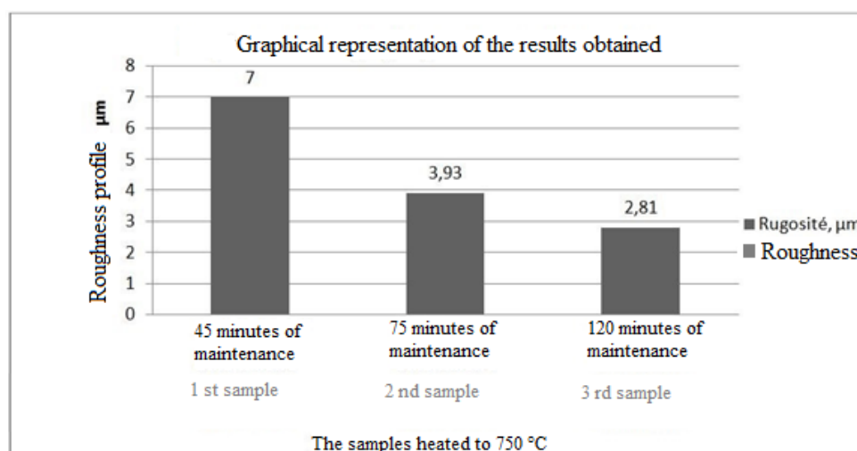
Figure 17. Histogram indicates the roughness.
