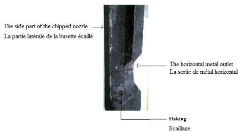
Figure 9. View of a sample of a nozzle after heating at the steelworks.
