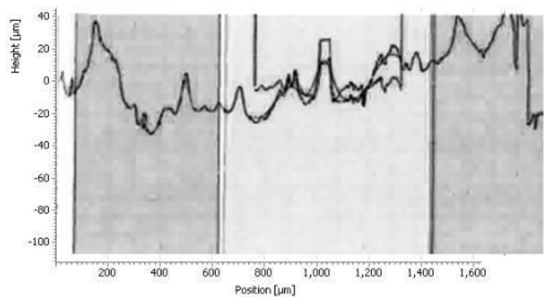
Figure 14. Roughness profile of the sample for 45 minutes of holding 750°C.
