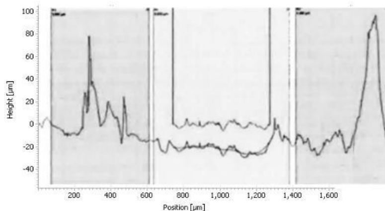
Figure 16. Roughness profile of the sample for 120 minutes of holding 750°C.
