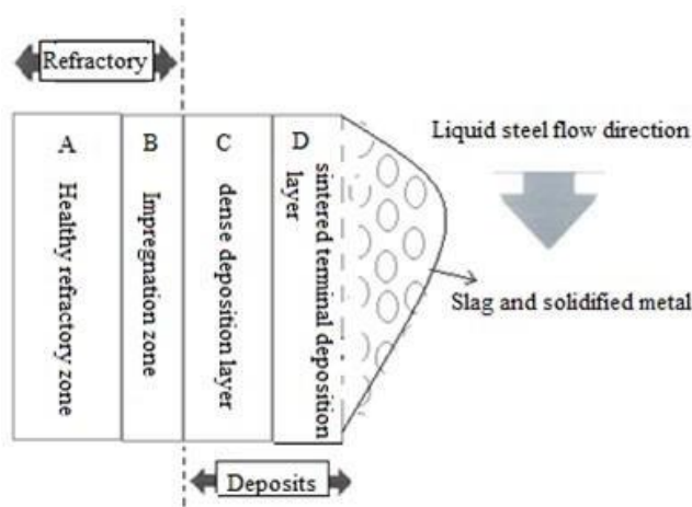
Figure 4. Layout diagram of the different layers.
