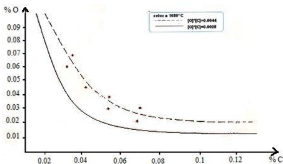
Figure 11. Relationship between carbon and oxygen.
