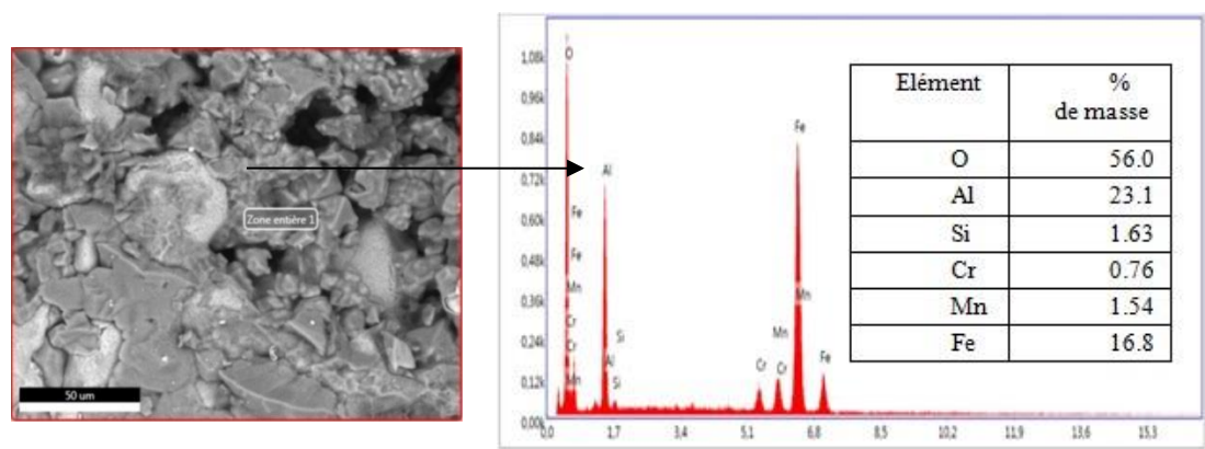
Figure 13. SEM image and chemical composition after EDS Right side.
