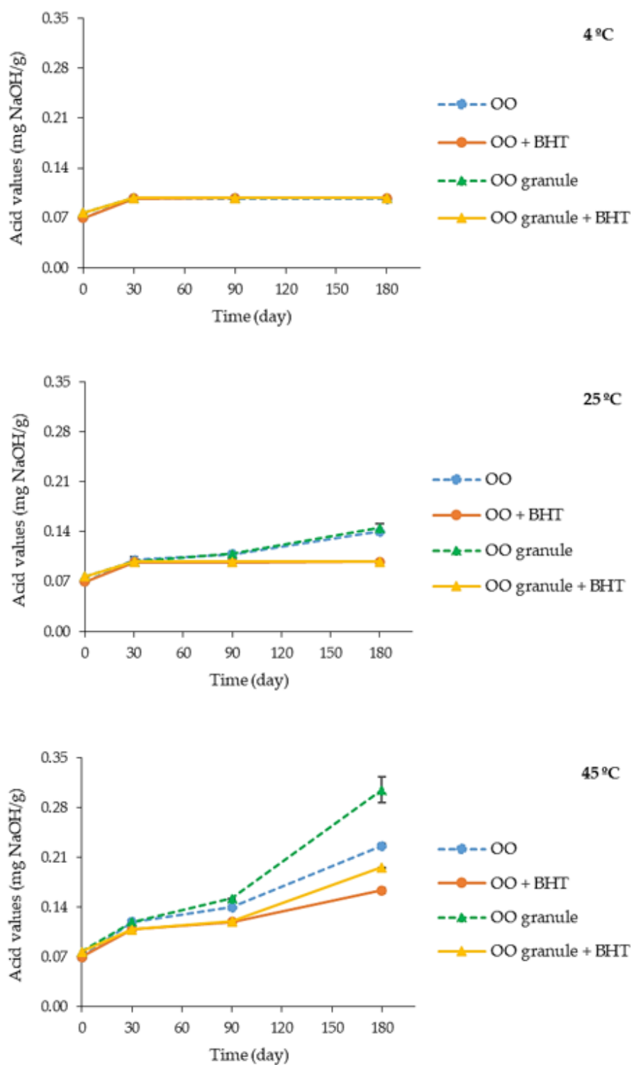
Figure 22. Acid values of ostrich oil (OO) and Avicel® PH-101 granules containing ostrich oil emulsion (OO granule), both with and without BHT, stored at 4 °C, 25 °C, and 45 °C for 180 days.
