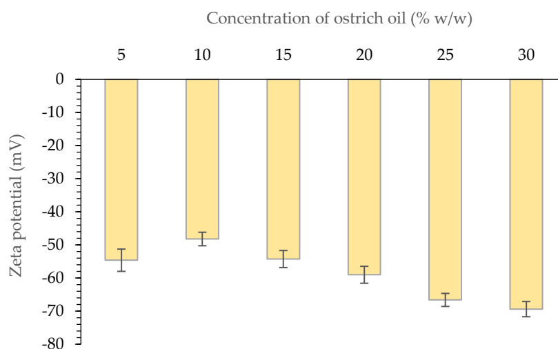
Figure 11. The zeta potential of emulsions containing 5% w/w - 30% w/w ostrich oil and 10% w/w lecithin.
