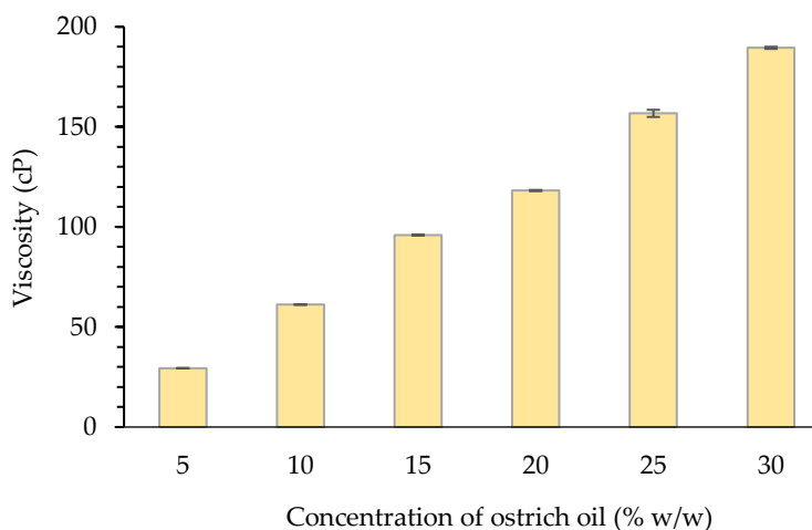
Figure 5. The viscosity of emulsions containing 5% w/w - 30% w/w ostrich oil and 10% w/w lecithin.
