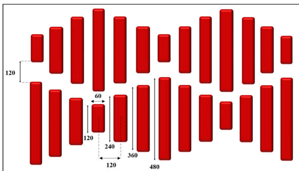
Figure 1. Schematic illustration of the pattern and dimensions of the shark skin design. Dimensions are given in micrometers.
