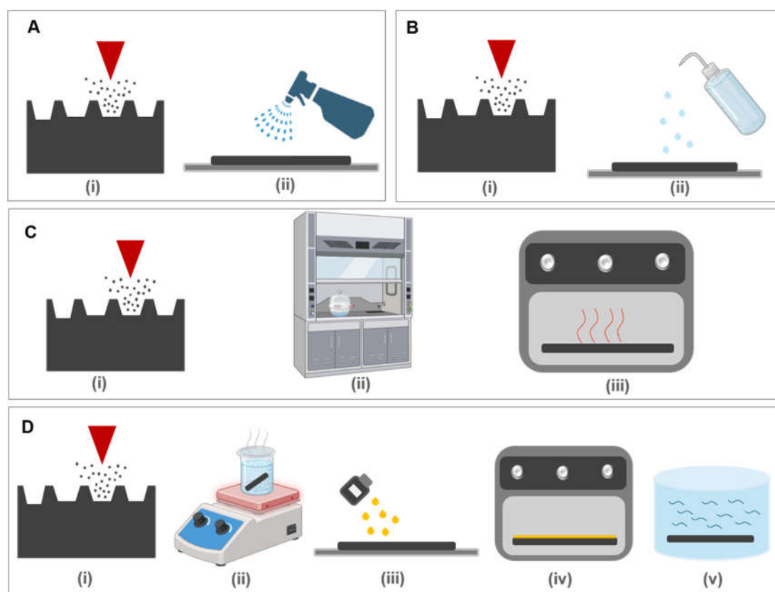
Figure 2. Schematic of the post-treatment experiments: (A) Spray coating (B) IPA coating (C) Silanization (D) Silicone oil treatment.
