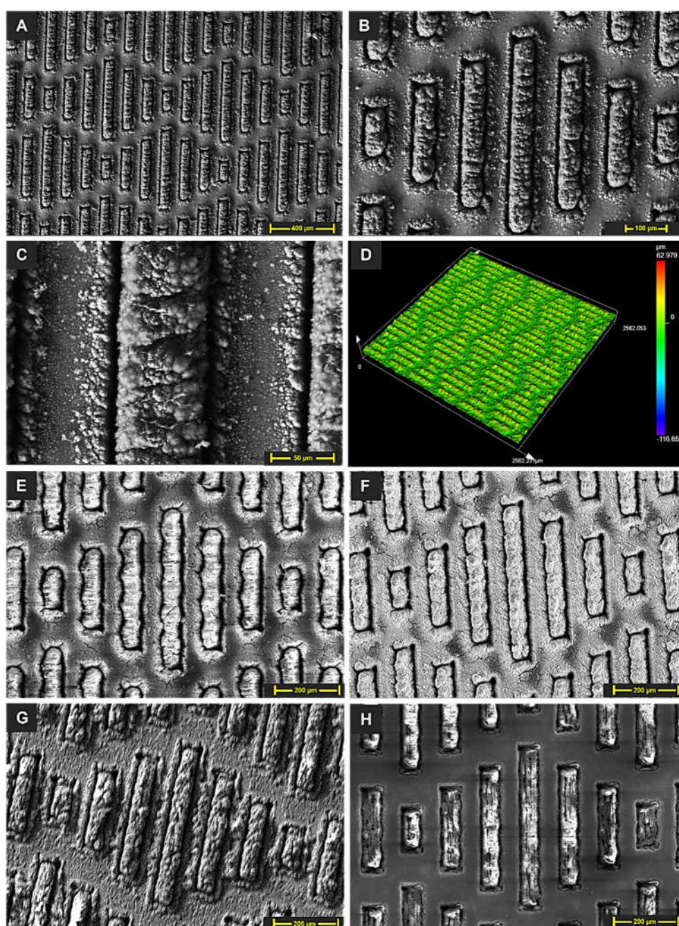
Figure 3. (A-C) SEM images of the fresh laser-textured shark skin design pattern. (D) Laser microscopy image of the fresh laser-textures sample. SEM images of the (E) Spray-coated (F) IPA-treated (G) Silanized (H) Silicone oil treated sample.
