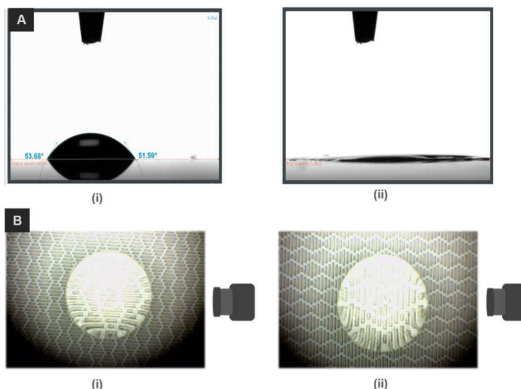
Figure 5. (A) Water contact angle on (i) pristine silicon wafer (ii) freshly laser machined shark skin pattern. (B) Top-view images of droplet contact angle capturing from two perspectives: (i) Parallel to the ribs (ii) Perpendicular to the ribs. .
