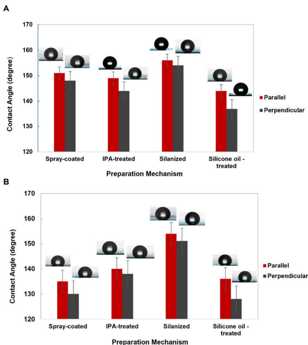
Figure 6. The measured water contact angle for four post-processed samples, Spray-coated, IPA-treated, Silanized, Silicone oil-treated. (A) right after the wetting transition. (B) one year after the wetting transition. Different levels of hydrophobicity and anisotropy can be observed among case studies. The contact angle measurements were conducted on five samples and error bars show the standard deviation.
