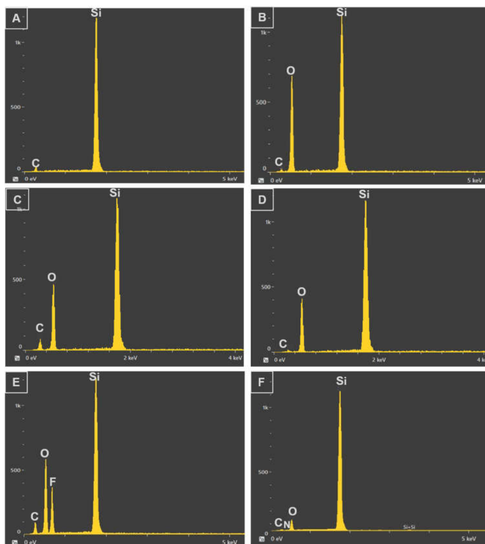
Figure 4. Chemical composition analysis (A) Pristine silicon wafer. (B) Fresh laser machined (C) Spray-coated (D) IPA-treated (E) Silanized (F) Silicone oil treated sample.
