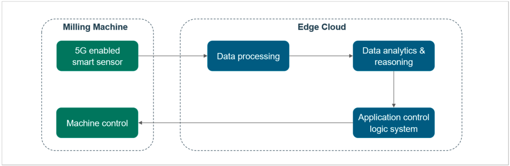
Figure 2. System Architecture Diagram Manufacturing Use Case (simplification adapted from [13]). For the implementation of the use case, a 5G-enabled smart sensor is integrated into a milling machine measuring acoustic emission signals during the machining. The measured data is wirelessly transmitted to an edge cloud system, where it is analyzed and used to implement an application control logic system to guarantee the desired quality of the machined product. The feedback from this system is then fed back into the machine control creating a seamlessly integrated quality control. For this process control to function, strict requirements regarding latency and reliability must be met. For the use case under consideration, it was defined that 99.99% of all transmitted data packets must be transmitted within 10 ms. The (simplified) FRER setup employed to guarantee this requirement is pictured in Figure 3. It uses a redundant communication setup in which the exact same packet is sent twice via two streams to guarantee that at least one of packet arrives on time which in this case is below 10 ms.
