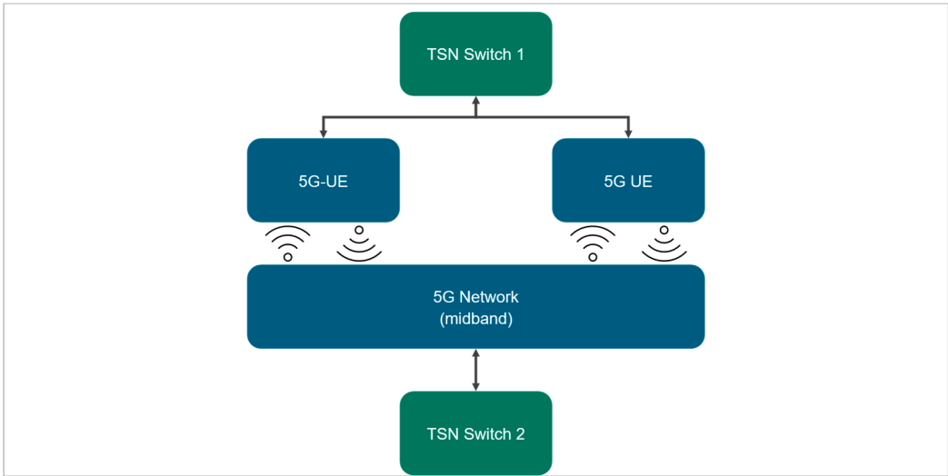
Figure 3. FRER Setup for the Inline Quality Assurance Use Case (Simplification, Adapted from [14]). Description of the Selected User-KPI and Evaluation of the Use Case The User-KPI timeliness and completeness as well as process capability have been selected from Table 1 to evaluate the use case. Process capability ( c_p and c_{pk} ) are calculated according to the following equations for the process capability indices [10]:
