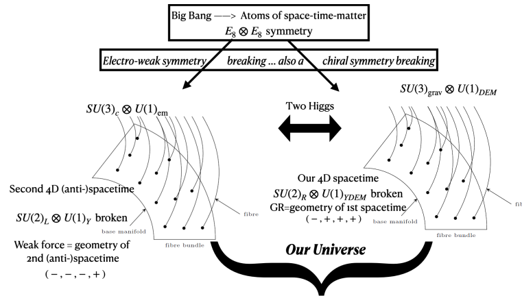
Figure 1. The proposed emergence of our universe from the breaking of E_8 \times E_8 symmetry.
