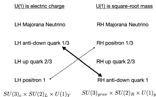
Figure 2. Left-Right fermions [18].
