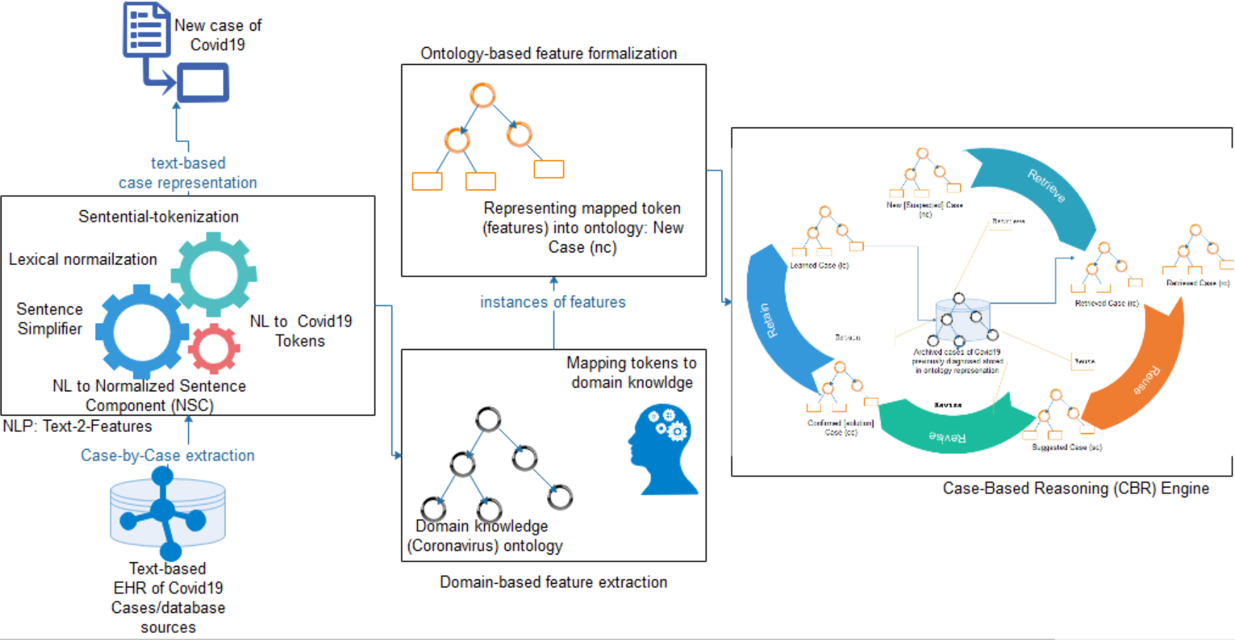
Figure 8: An overview of the proposed framework using case-based reasoning (CBR) model to classify new cases of coronavirus (COVID-19) as either positive or negative
