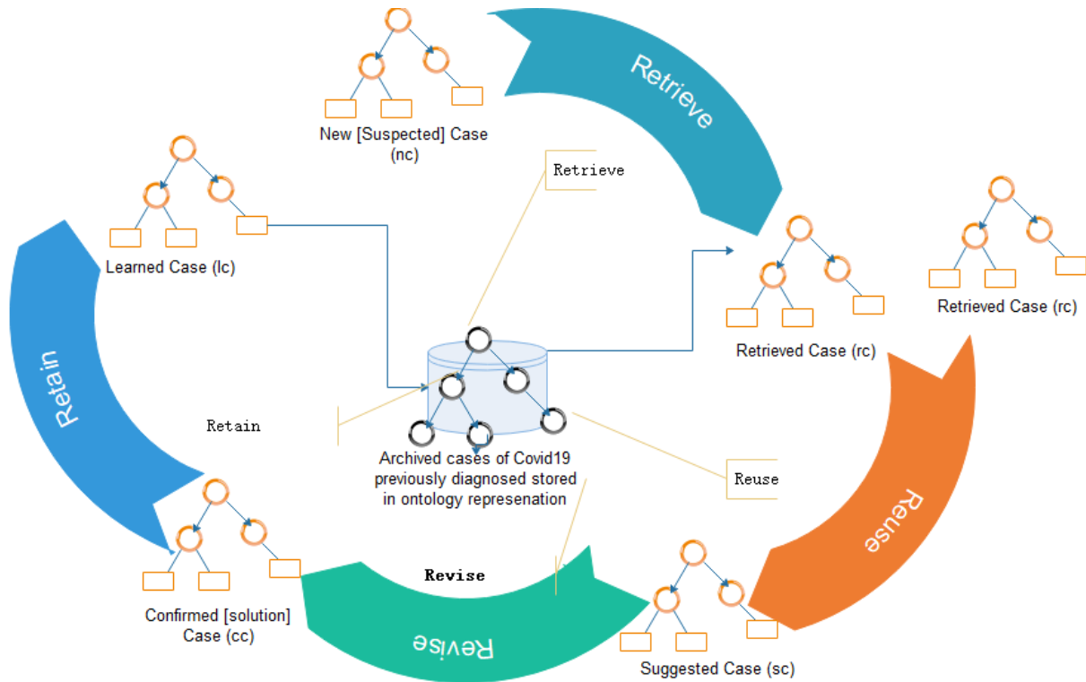
Figure 12: A model of the proposed case-based reasoning (CBR) used in the NLP-Ontology oriented Spatial temporal framework for detecting COVID-19
