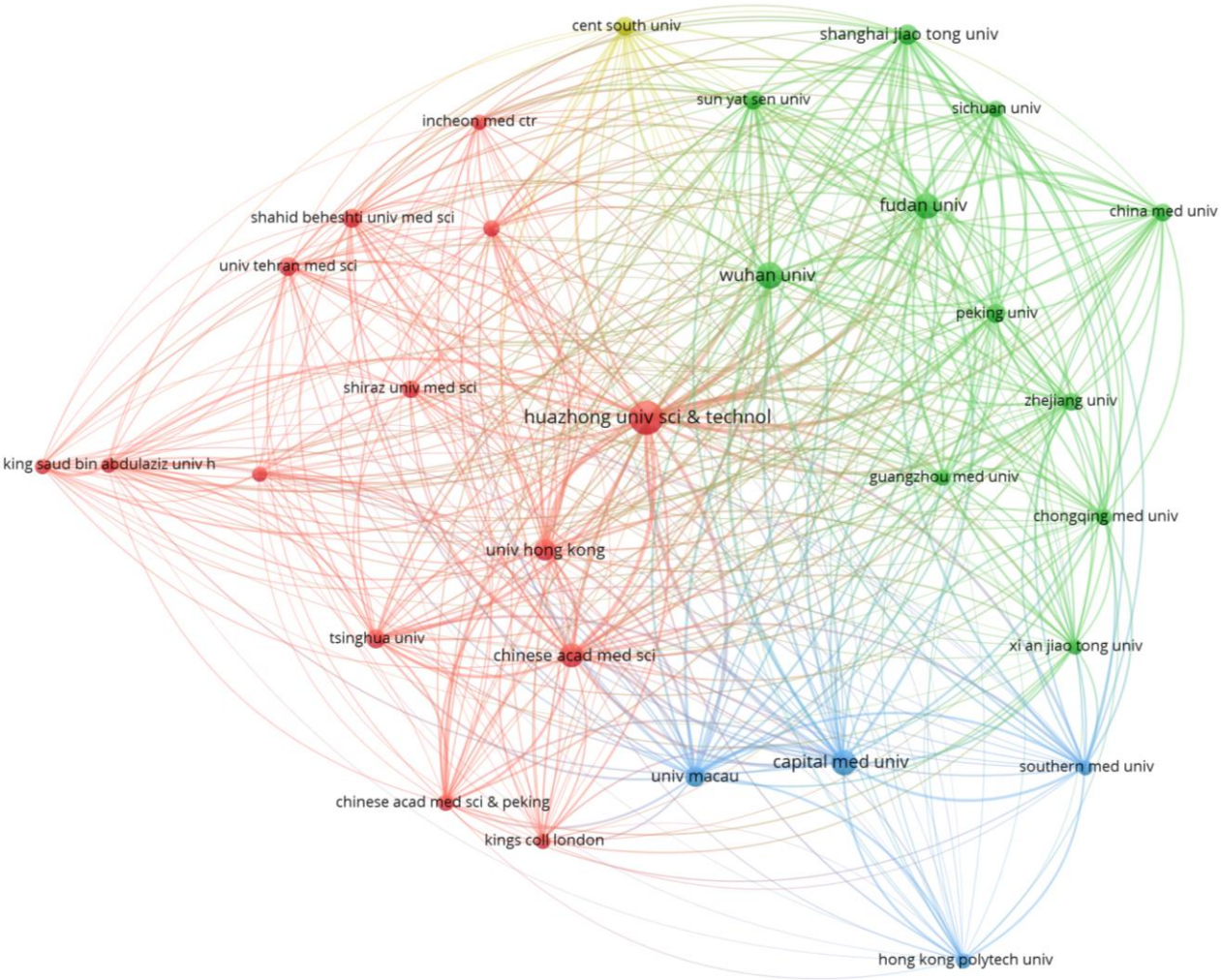
Figure 3: Bibliographic coupling among institutions
