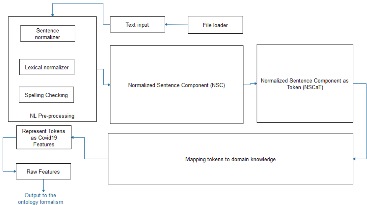
Figure 9: A patient text-based medical record natural language processing (NLP) and feature extraction architectural pipeline
