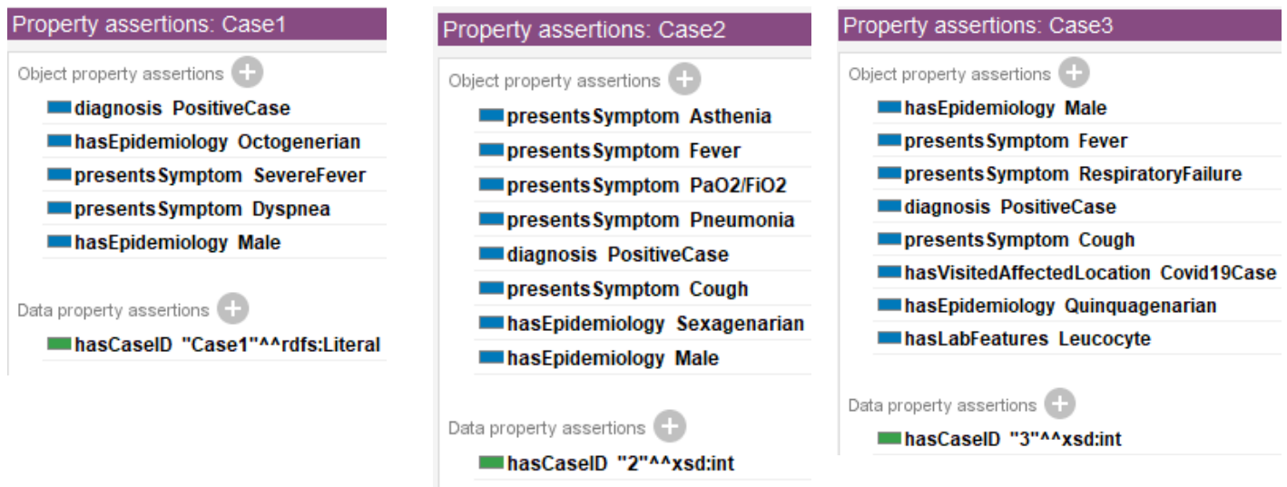
Figure 18: An illustration of case representation as shown in Protégé for cases a 1, 2, and 3 from the 68 cases extracted from the data source
