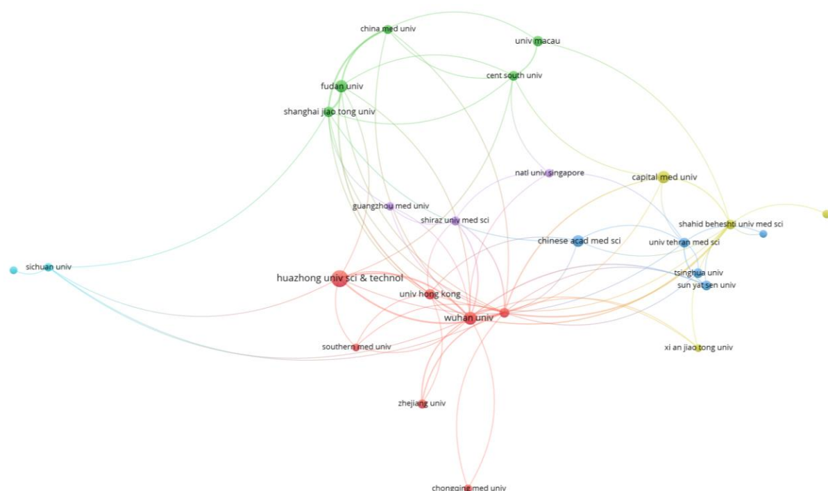
Figure 6: Author citation by institution
