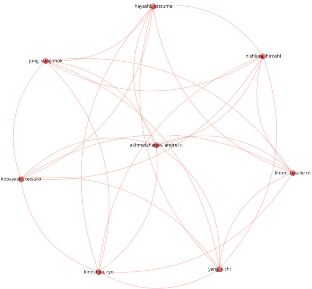
Figure 5: Co-authorship and Authors’ analysis
