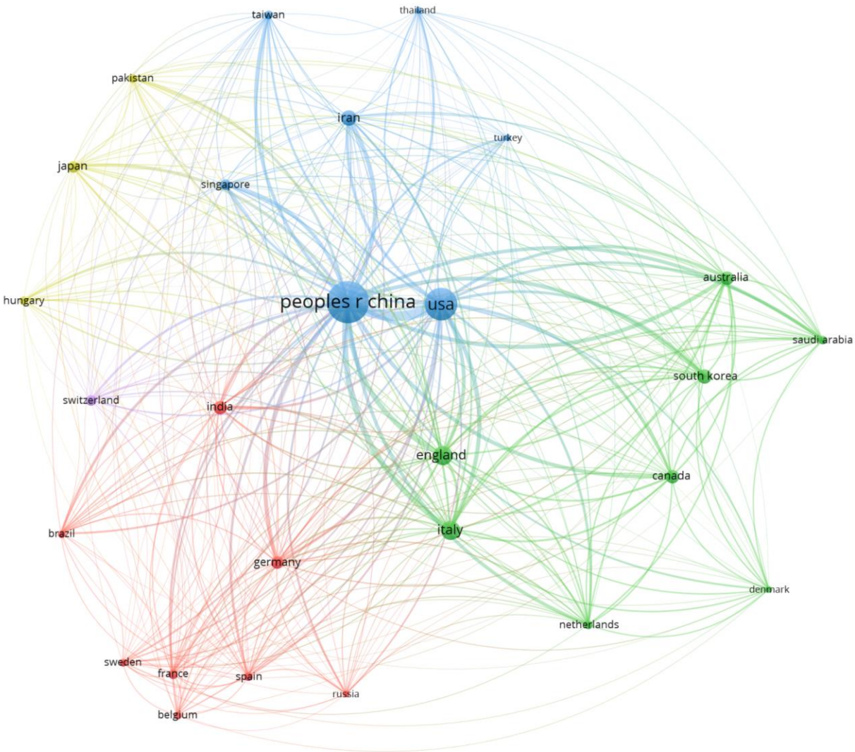
Figure 2: Bibliographic coupling among the countries
