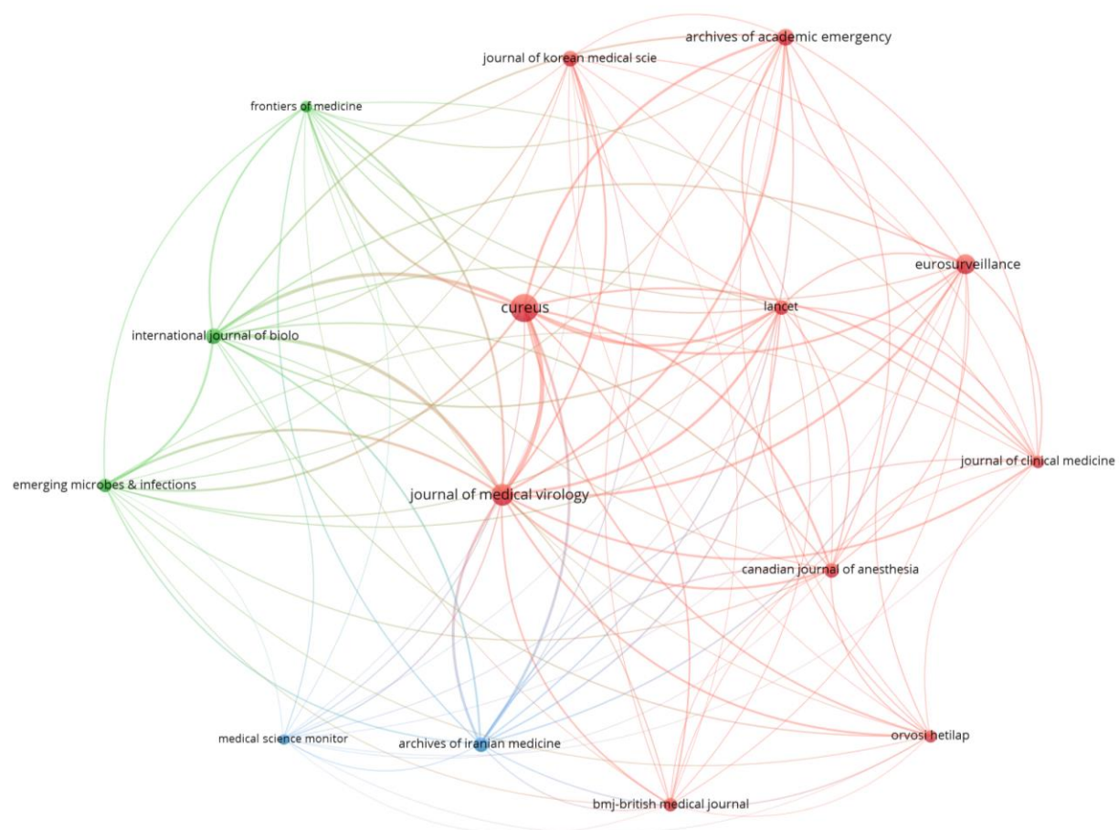
Figure 4: Bibliographic coupling among the Journals
