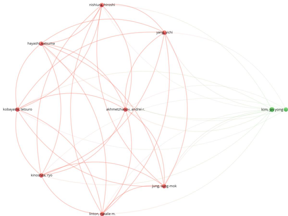
Figure 1: Bibliographic coupling among the authors
