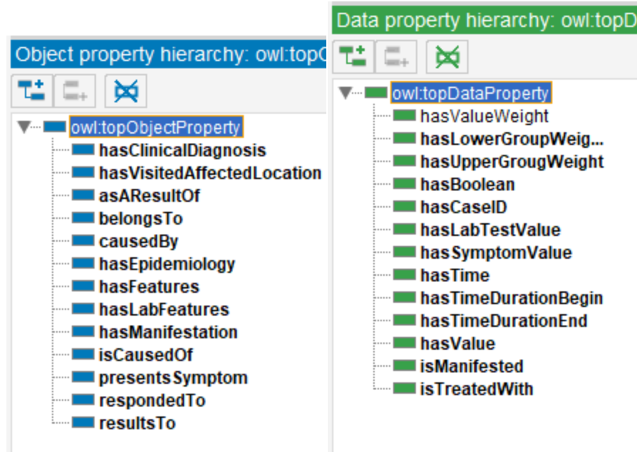
Figure 16: A listing of concepts (classes), individuals (instances of classes), object properties and data type properties modeled in a domain-based knowledge repository of COVID-19
