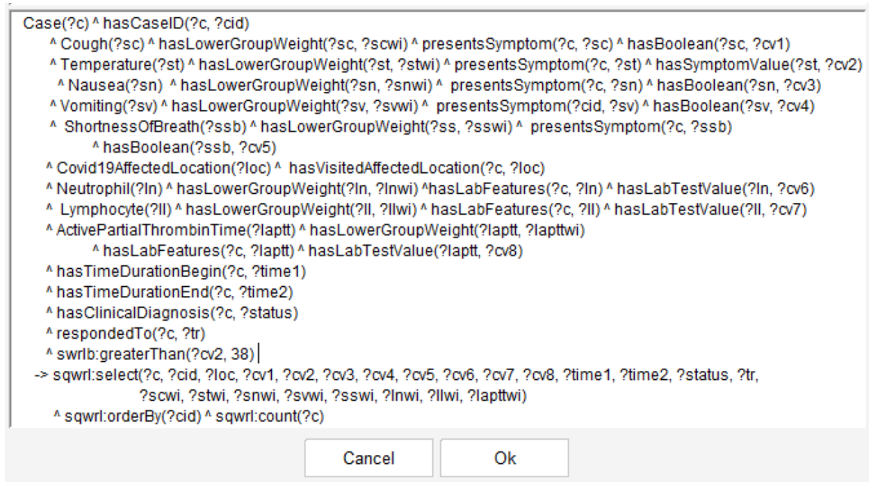
Figure 17: A sample SQWRL query constructed to retrieve similar cases corresponding with the new case ( nc ) accepted as input.
