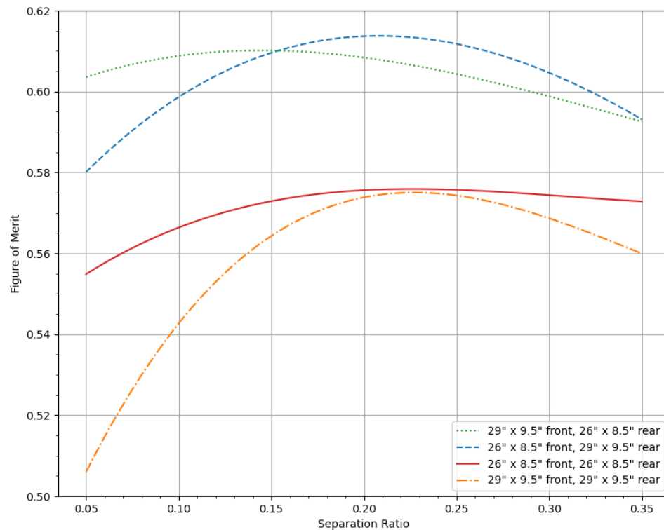
Figure 14. Variation of Figure of Merit (FM) with z/D separation ratio.
