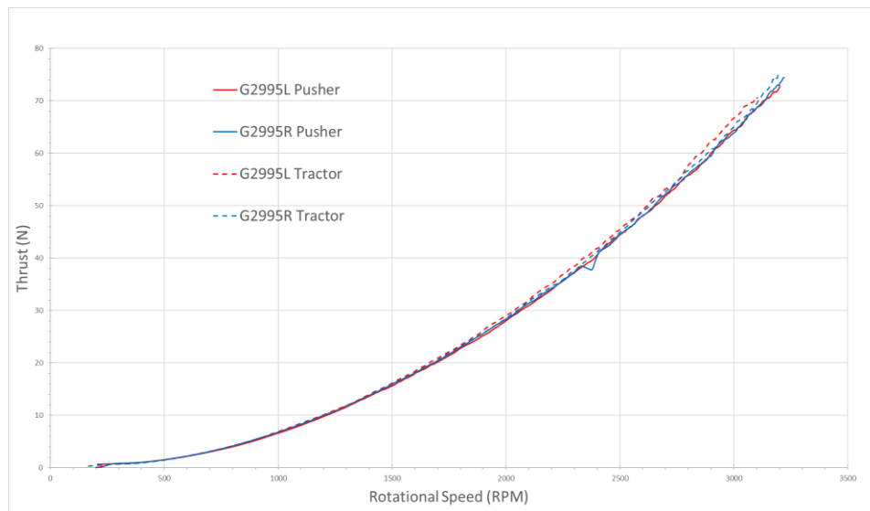
Figure 4. The thrust of isolated propellers, comparing handedness and direction (tractor or pusher). (a) Thrust comparison for the 26-inch propeller. (b) Thrust comparison for the 29-inch propeller.
