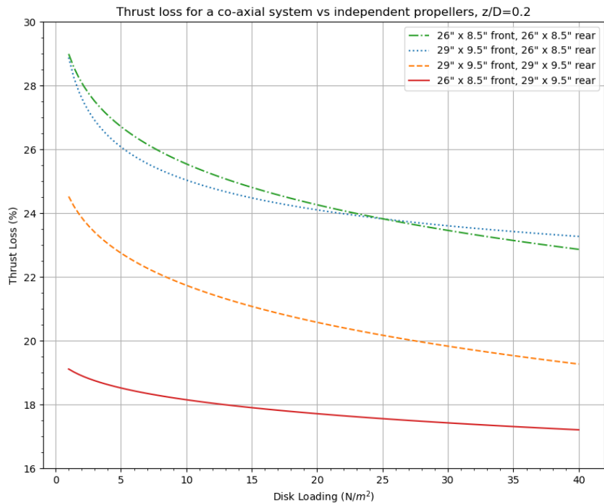
Figure 5. Percentage thrust loss for the co-axial system in comparison to an ideal system, at a z/D ratio of 0.2.
