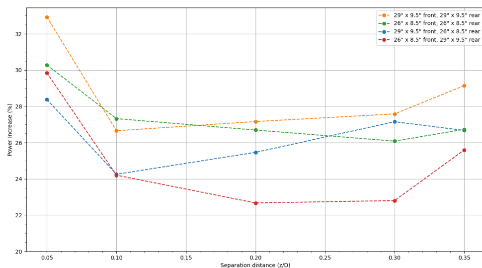
Figure 15. Power increase percentage across z/D separation ratios.
