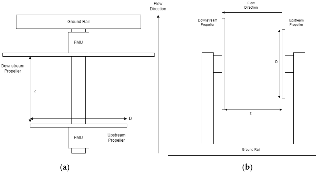
Figure 2. Diagram of the propeller testing arrangement at the maximum z/D ratio (separation). (a) Plan-view of the equipment. (b) Side-view of the equipment.
