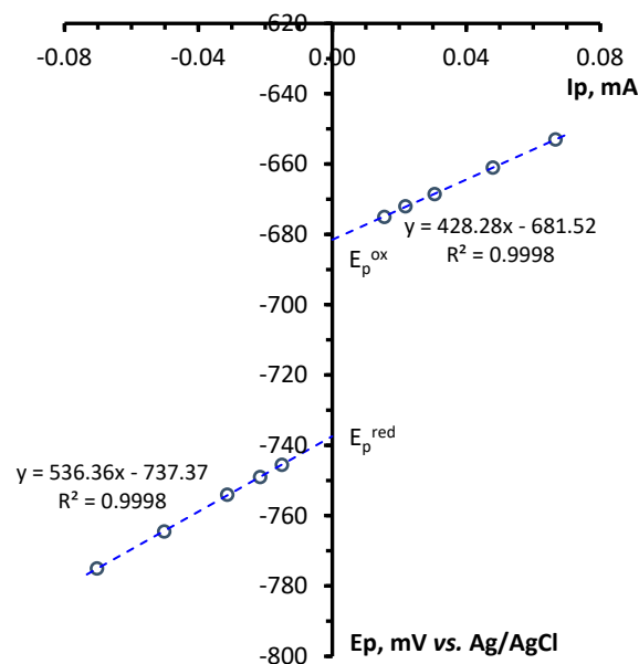
Figure 3. (left) CV curves of the reduction of 1a ( 3 \times 10^{-3} M) in 0.1 M Bu_4NBF_4/MeCN on a glassy carbon disc electrode at potential sweep rates of 0.05, 0.10, 0.20, 0.50, and 1.00 V/s. (right) Plots of reduction and reciprocal oxidation peak potentials versus the peak current for the respective process.
