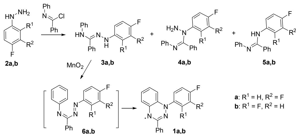
Scheme 1. Synthesis of 1-(3,4-difluorophenyl)- ( 1a ) and 1-(2,4-difluorophenyl)-3-phenyl-1,4-dihydrobenzo[e][1,2,4]triazin-4-yl ( 1b ).
