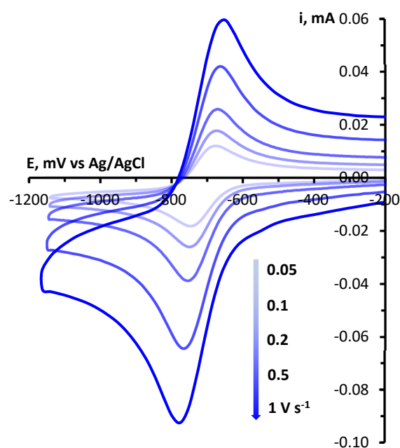
Figure 2. (left) CV curves of the oxidation of 1a ( 3 \times 10^{-3} \text{ M} ) in 0.1 M \text{Bu}_4\text{NBF}_4/\text{MeCN} on a glassy carbon disk electrode at potential sweep rates of 0.05, 0.10, 0.20, 0.50, and 1.00 V/s. (right) Dependences of the potentials of the peaks of oxidation and reciprocal reduction on the current at the peak for the corresponding process.
