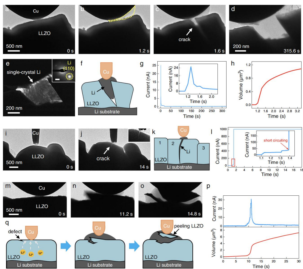
Figure 3. Crack initiation and lithium penetration in single-crystal LLZO induced by Li eruption under constrained Cu|LLZO interface. Li eruption and stress buildup lead to sudden fracture in LLZO (a–c). Li penetrates and fills the crack, eventually splitting the entire particle (d–f). Current and volume traces reveal the onset of mechanical failure during fast Li deposition (g–h). Lateral extrusion under pressure enables stable Li plating without LLZO fracture (i–k). Direct comparison of both growth modes (l–n). Schematics of pressure-modulated growth mechanisms—creep-induced lateral growth vs. high-rate vertical rupture (o–q). (Adapted with permission from ref. [100], Springer Nature 2022).
