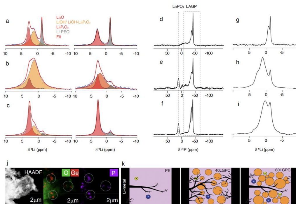
Figure 5. DNP-enhanced NMR and HAADF-STEM analysis of SEI composition and lithium dendrite suppression in polymer–ceramic composite electrolytes. ^6\text{Li} MAS NMR spectra deconvoluted into \text{Li}_2\text{O} , \text{LiOH} , \text{Li}_3\text{PO}_4 , and \text{Li-PEO} species across PE, 40LGPC, and 60LGPC compositions (a–c). ^{31}\text{P} MAS NMR spectra showing signals from \text{Li}_3\text{PO}_4 and LAGP (d–f). DNP-enhanced ^6\text{Li} NMR showing signal amplification near the \text{Li}/\text{SEI} interface (g–i). HAADF-STEM and EDX maps of O, Ge, and P revealing interphase structure (j). Schematic representations of dendrite behavior under different ceramic loadings: unrestricted in PE, blocked in 60LGPC (k). (Adapted with permission from ref. [109], Springer Nature 2024).
