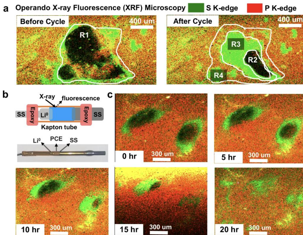
Figure 1. Self-healing behavior of plastic ceramic electrolyte (PCE) revealed by operando X-ray fluorescence (XRF) microscopy. (a) Elemental mappings of sulfur (green) and phosphorus (red) before and after cycling highlight polymer and ceramic migration into a pre-existing void; (b) Schematic of the in situ XRF measurement setup using a Kapton tube cell; (c) Time-resolved XRF images show progressive void closure within 20 hours via dual-phase polymer and ceramic infiltration. (Adapted with permission from ref. [78], Springer Nature 2024).
