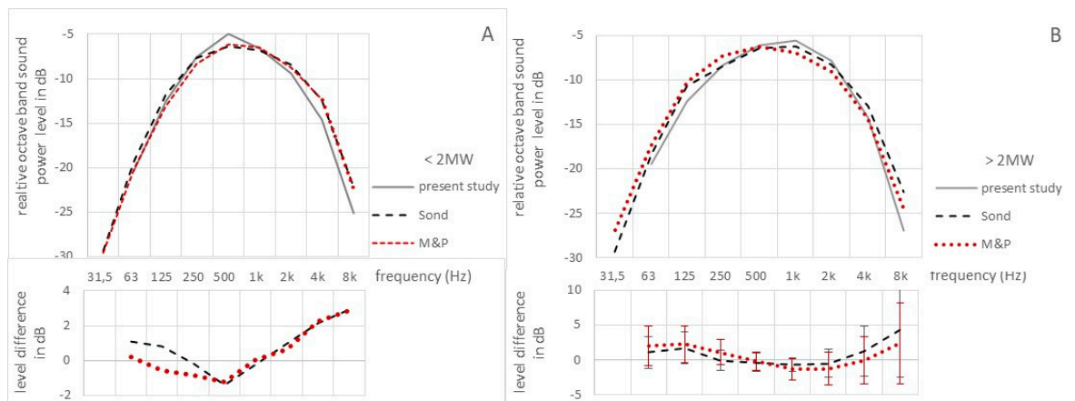
Figure 10. Above: average normalized sound power octave band spectra for wind turbines < 2 MW (A, left) and > 2 MW (B, right) in the present study compared to spectra from Sondergaard [1] and Møller and Pedersen [3]. Below: differences between earlier and present spectral levels, at right with 1 s.d. error bars; positive difference means present value is lower. Present study based on 9 turbines < 2 MW and 114 > 2 MW, the latter include 25 turbines with serrations.
