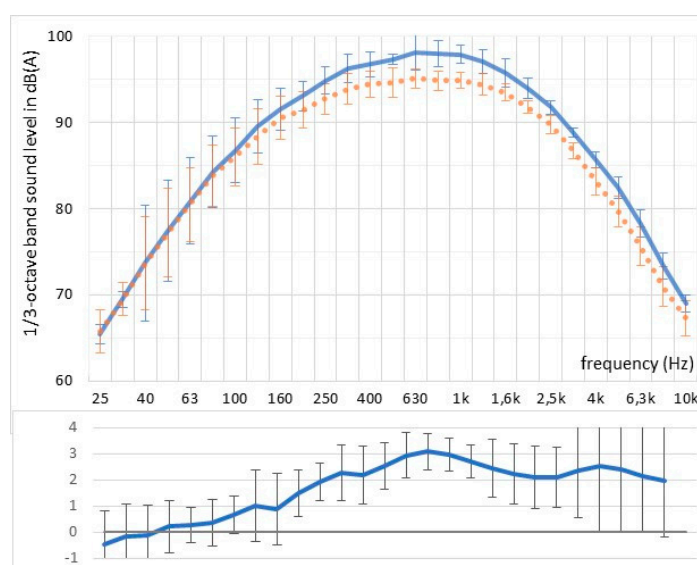
Figure 12. Above: 1/3 octave band spectra of 11 turbine types with serrations (dotted red line) and without (solid blue line). Below: difference between non-TES and TES spectral levels. Vertical bars: standard deviation.
