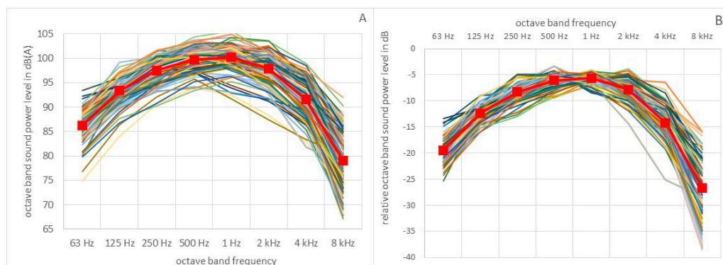
Figure 9. Individual sound power octave band spectra at rated power (A, left) and normalized to individual sound power level L_{WA,max} (B, right), with arithmetic means (bold red lines with markers). Based on data from 123 turbine types.
