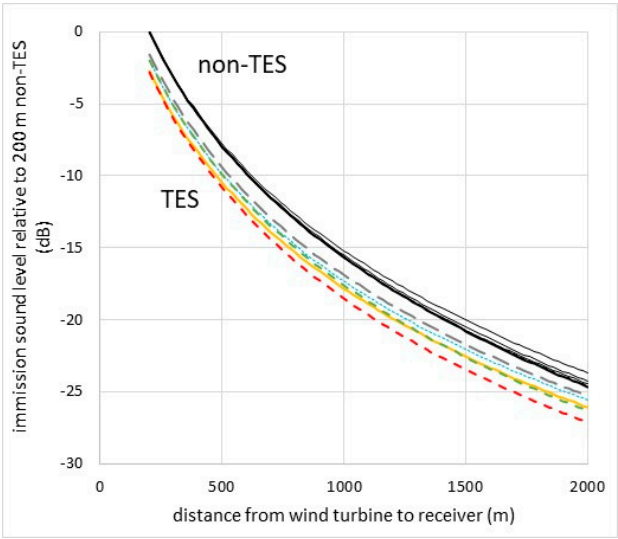
Figure 14. Attenuation (with reference 0 dB at 200 m of non-TES turbine type) at distances up to 2 km from five wind turbine types without (black lines) and with trailing edge serrations (color scheme in Figure 15).
