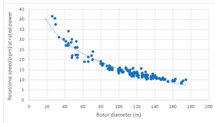
Figure 4. Maximum rotational speed (in rotations per minute or RPM) of 221 turbine types plotted versus rotor diameter with best exponential approximation (dotted line). Exceptional turbine (18 m diameter, 120 rpm) excluded.
