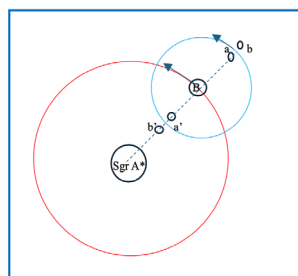
Figure 2. The orbits of a stellar cluster around the Sgr A*. B is a massive body (black hole or star) orbiting around the Sgr A* with radius R. a and a' are a group of stars orbiting around B with radius r. b and b' are another group of stars orbiting around the Sgr A*. Sgr A*, B, a and a', b and b' are on a straight line. The distance between a and b and between a' and b' are very small. The arrows are the directions of the orbits.
