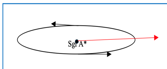
Figure 1. The Sgr A* and the motion of the Milky Way. The stars are orbiting or rotating around the Sgr A* along the black arrow while the whole galaxy is moving along the red arrow. The direction of one of the black arrows is contrary to the red one.
