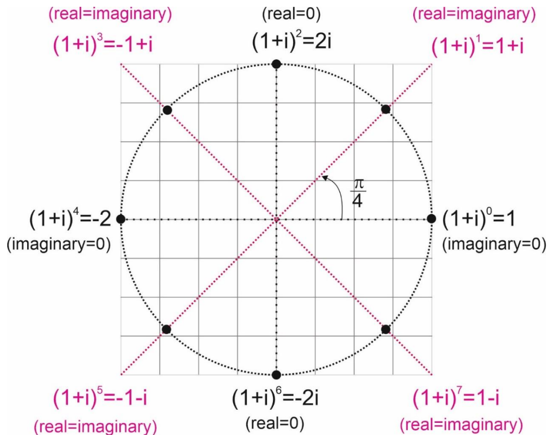
Figure 1. C_8 cyclic group when multiplications of (1+i) .
