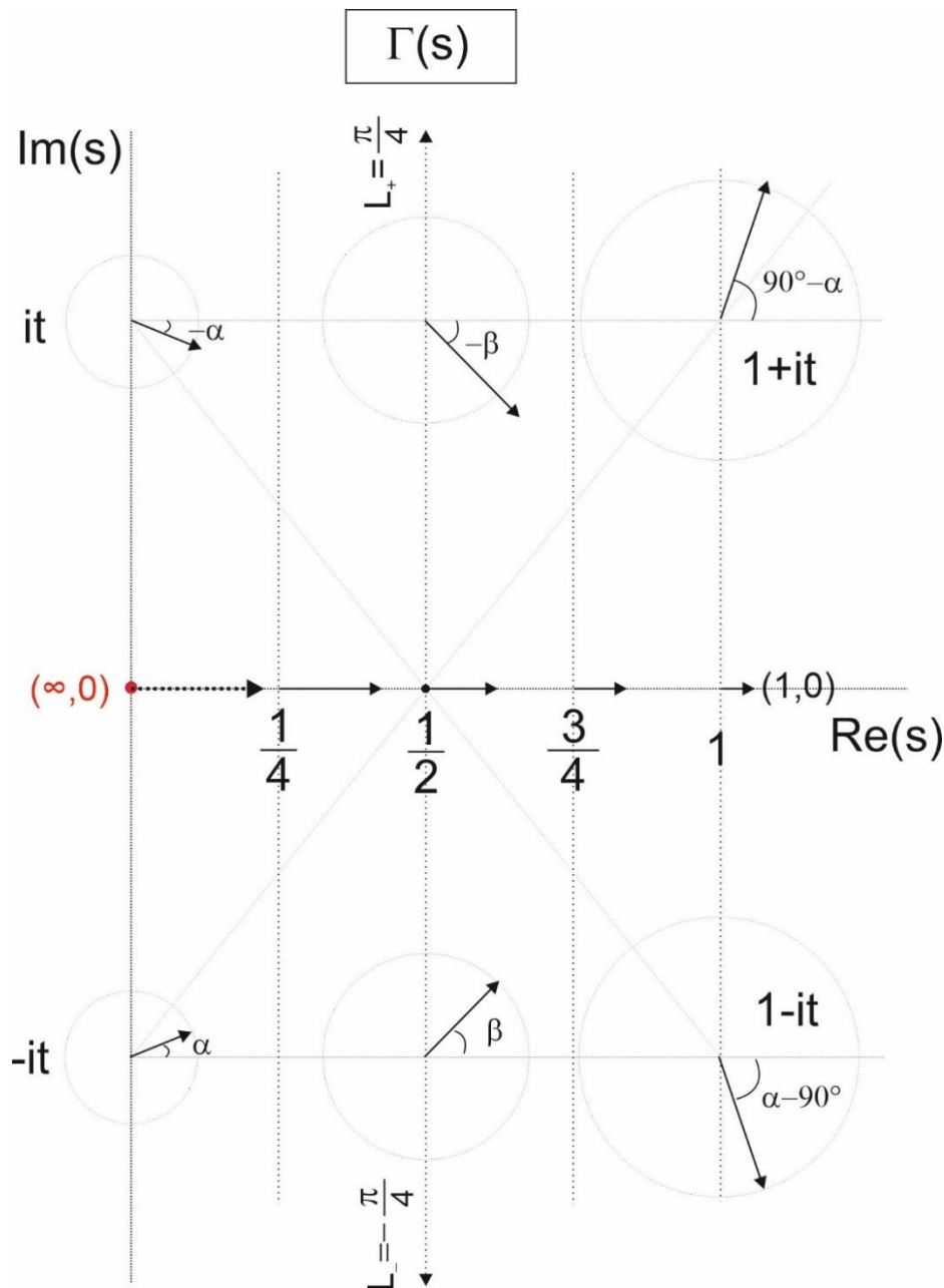
Figure 1. Gamma function vector field in the region 0 \leq \sigma \leq 1 .
