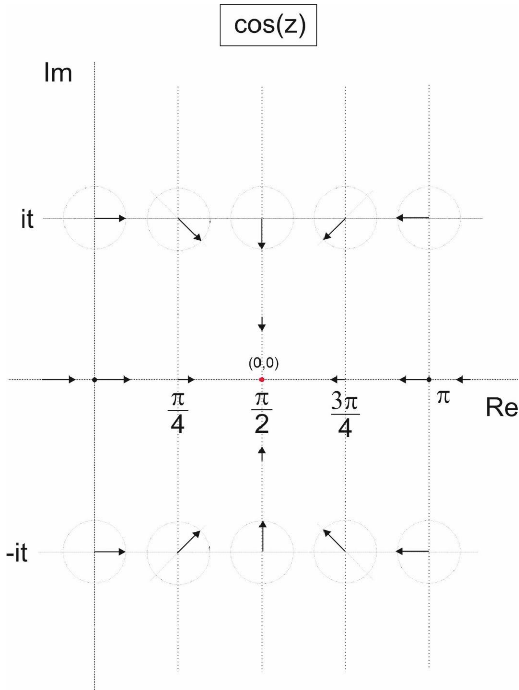
Figure A2. The \cos(\pi s) vector field in the complex plane for 0 \leq \sigma \leq 1 .
