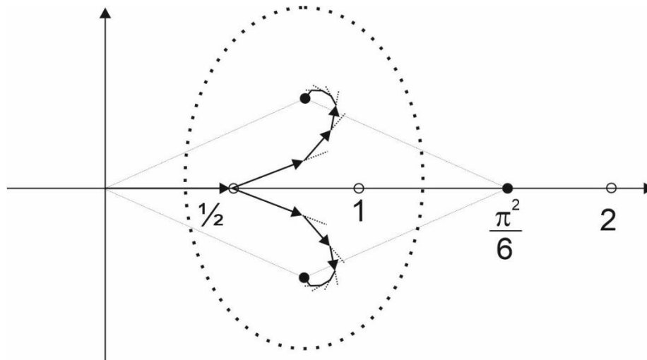
Figure 1. Initially entangled two particles ( \sigma = 2 ) is viewed as a system: total rotational energy is 2f(p^2) = \frac{\pi^2}{6} . After the decay the total vorticity.
