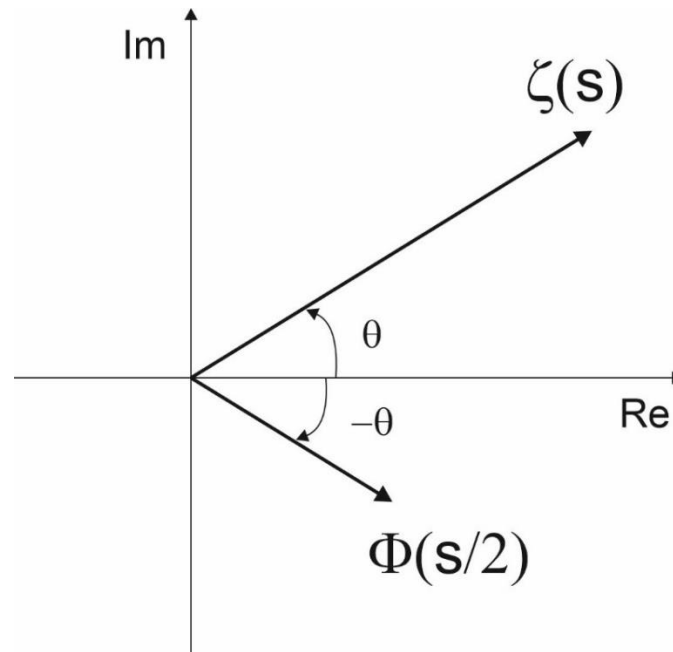
Figure 2. The absolute values of the arguments of the functions \Phi(s/2) and \zeta(s) equal to each other, but with opposite signs.
