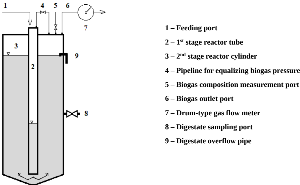
Figure 2. Two-stage psychrophilic anaerobic bioreactor.
