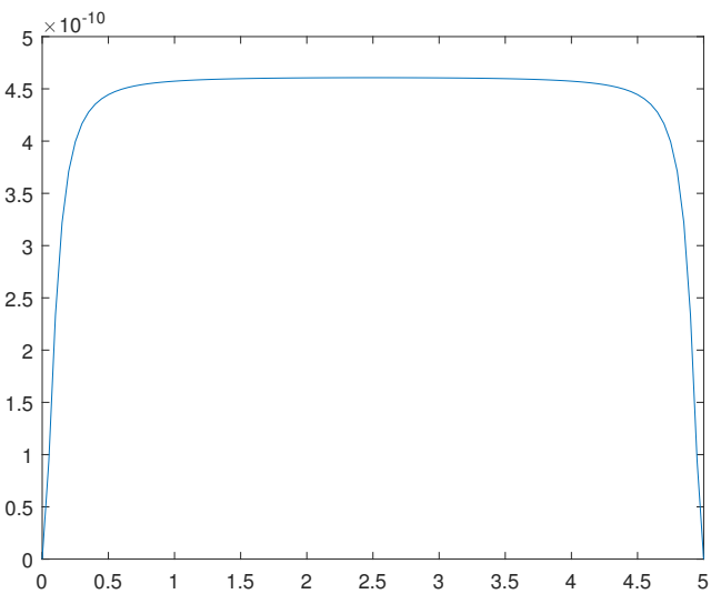
Figure 13. Solution \phi_N(x) for the \omega = 1.0 .
