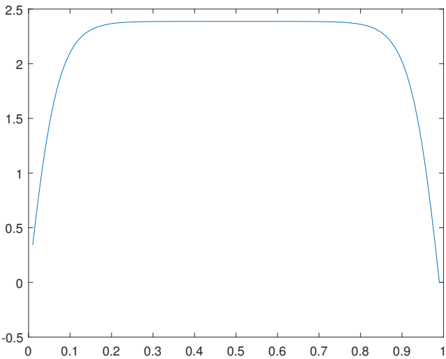
Figure 36. Optimal solution u(x) for the case A.
