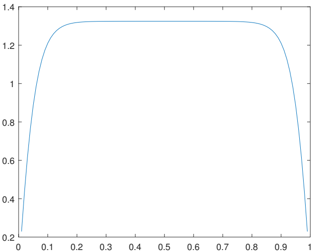
Figure 47. Solution u_0(x) through the dual functional for the case B, \varepsilon = 0.01 .
