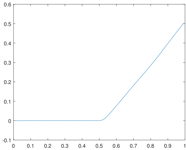
Figure 38. Optimal solution u(x) for the case f(x) = 0 .
