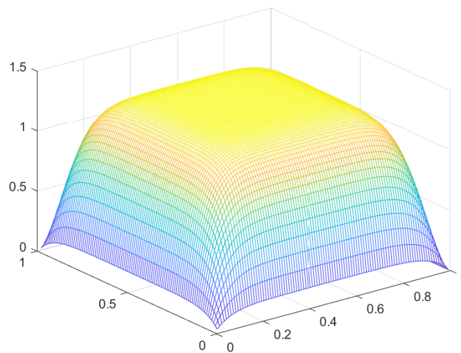
Figure 42. Solution u(x, y) for \varepsilon = 0.01
