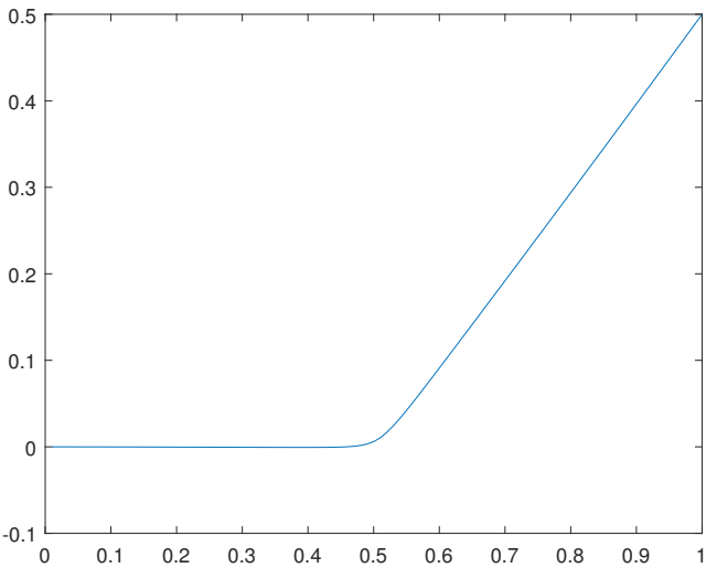
Figure 35. Optimal solution u(x) for the case f(x) = 0 .
