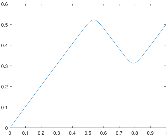
Figure 34. Optimal solution u(x) for the case f(x) = \sin(\pi x)/2 .
