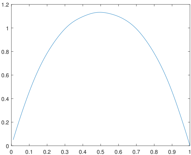
Figure 44. Solution \hat{u}_0(x) through the dual functional for \epsilon = 0.1 .
