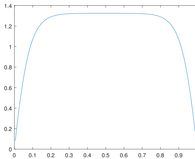
Figure 45. Solution \hat{u}_0(x) through the dual functional for \varepsilon = 0.01 .
