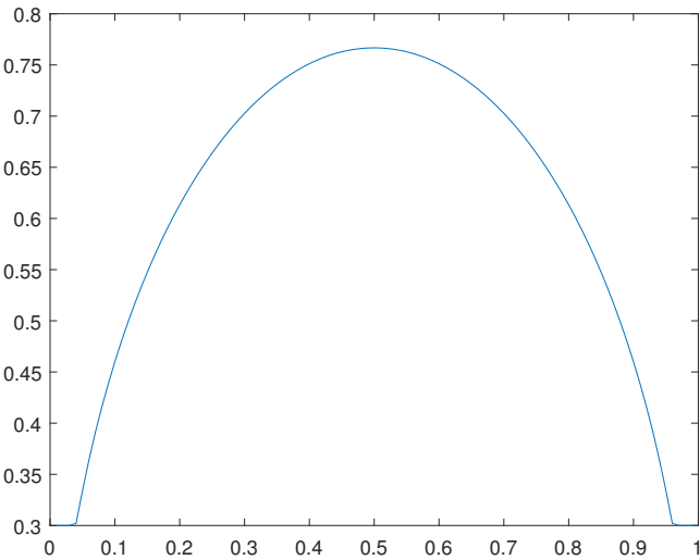
Figure 39. Optimal solution L_1(x) for the case A.
