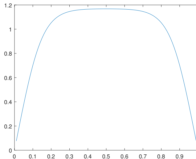
Figure 43. Solution u(x) for \varepsilon = 0.01
