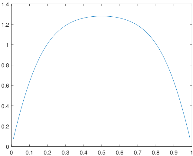
Figure 46. Solution u_0(x) through the dual functional for the case A, \varepsilon = 0.1 .
