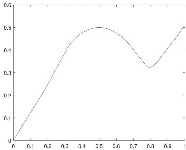
Figure 37. Optimal solution u(x) for the case f(x) = \sin(\pi x)/2 .
