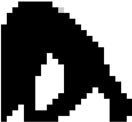
Figure 41. Optimal shape \lambda_1(x, y) for the beam of case B.
