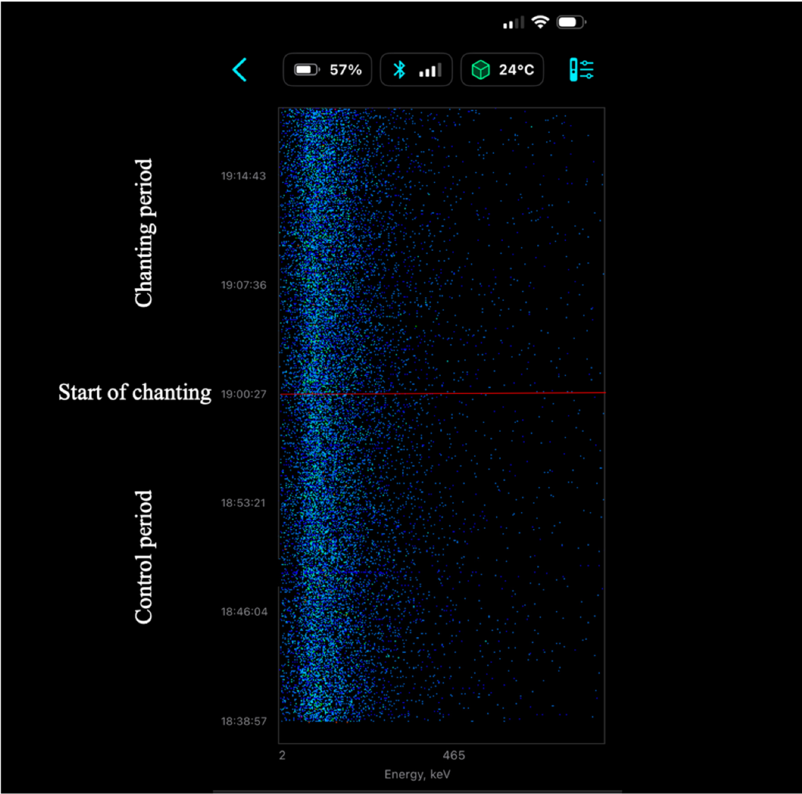
Figure 2. Representative spectrogram illustrating the temporal distribution of detected radiation events across different energy levels during a single chanting session. The X-axis represents energy (logarithmic scale), and
