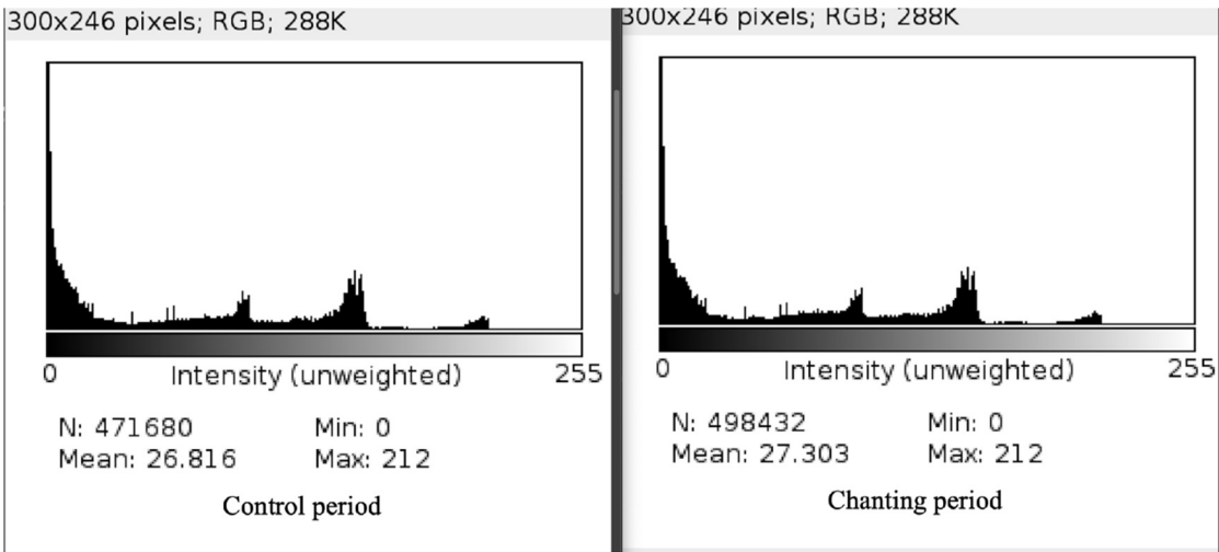
Figure 3. Histogram analysis of the spectrogram segments (Figure 2) performed using ImageJ software. The left histogram shows the pixel intensity distribution for the control period, and the right histogram shows the distribution for the chanting period. The total integrated counts for each period are indicated, representing the accumulated detection events.
