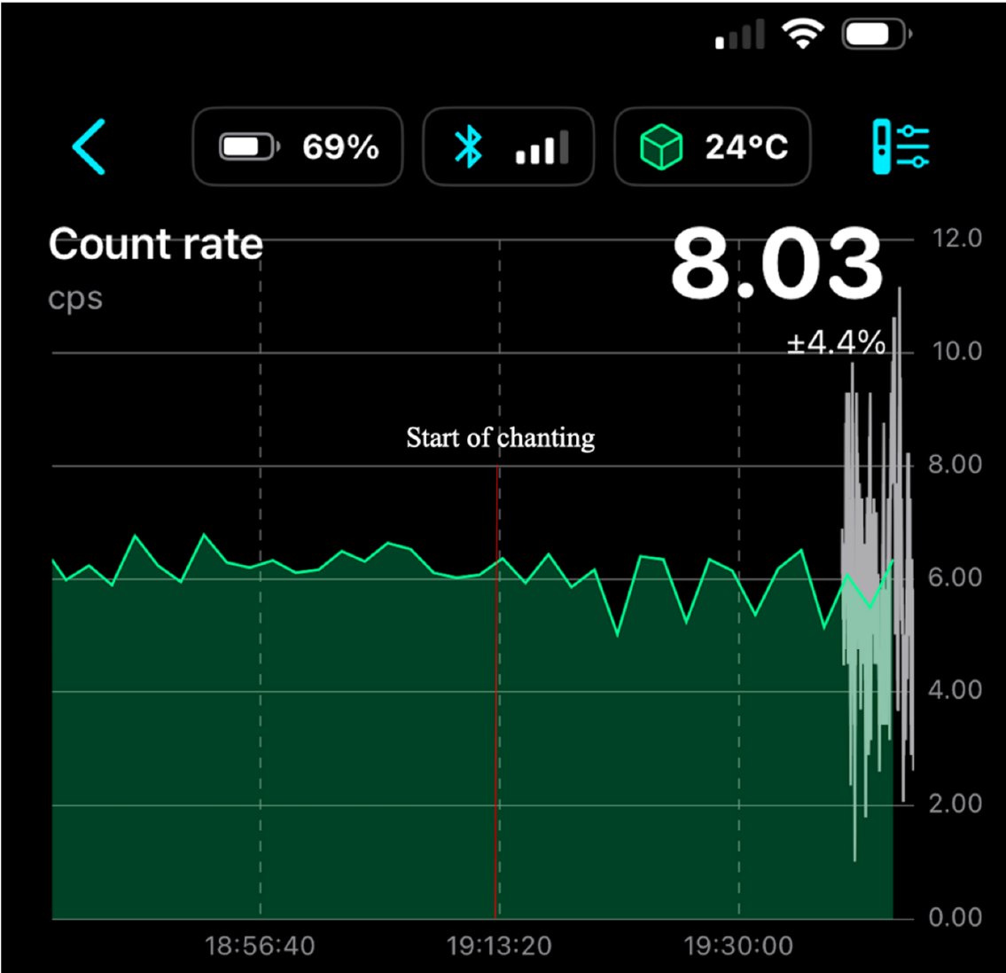
Figure 4. Temporal fluctuations of the detected natural radioactivity count rate (CPS) during representative control and chanting periods. The figure illustrates the difference in the amplitude of fluctuations between the two periods.
