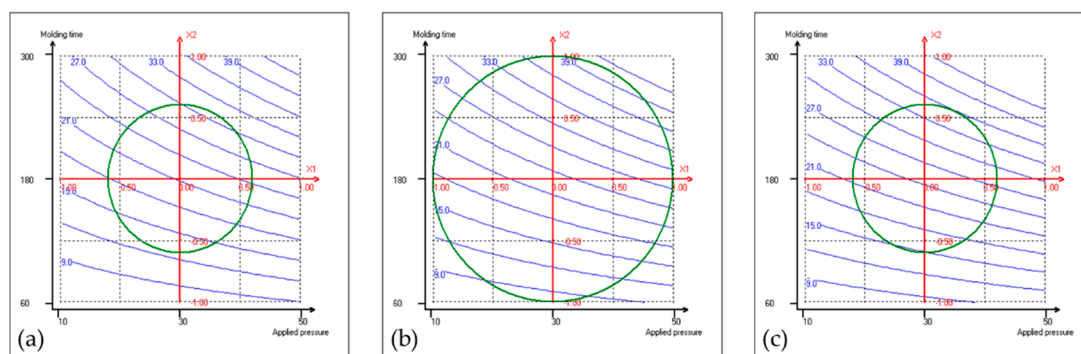
Figure 2. Isoresponse curves for energy consumption (kW h/m 2 ) at 160 °C (a), 180 °C (b) and 200 °C (c) mold temperatures.
