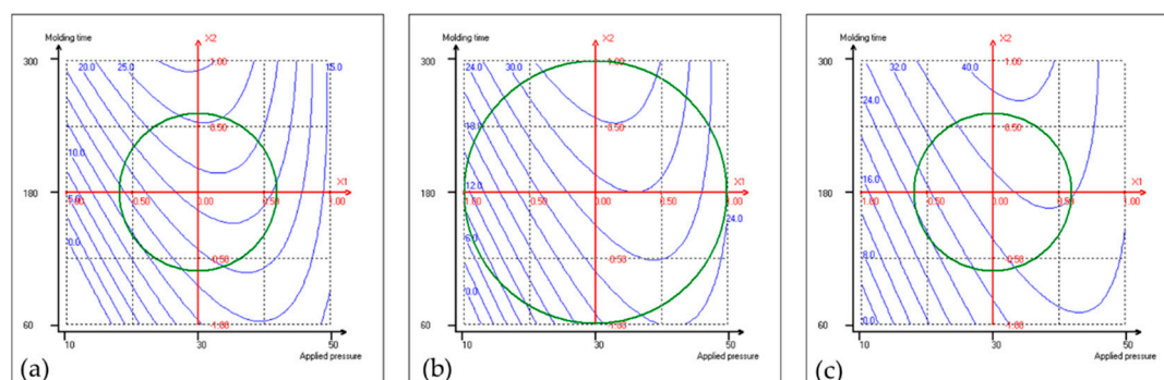
Figure 1. Isoresponse curves for flexural strength (MPa) at 160 °C (a), 180 °C (b) and 200 °C (c) mold temperatures.
