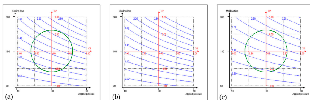
Figure 3. Isoresponse curves for climate change ( \text{kg CO}_2\text{eq/m}^2 ) at 160 °C(a), 180 °C(b) and 200 °C (c) mold temperatures.
