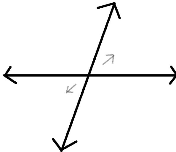
Figure 9. A two-dimensional substance.
