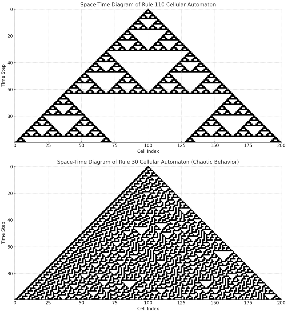
Figure 4. Cellular automata exhibiting complex behavior.
