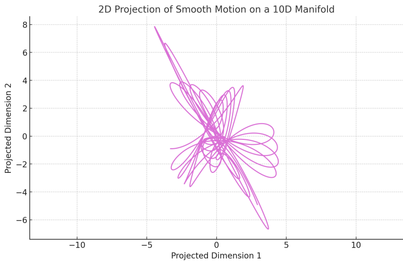
Figure 2. A chaotic system in a low-dimensional projection of a high-dimensional manifold.
