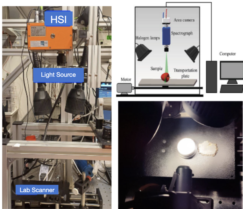
Figure 1. Overview of the hyperspectral imaging setup. (Left) The Hyperspectral Imaging System (HSI) with labeled light sources (halogen lamps) and components. (Top-right) Diagram of the experimental arrangement, clearly annotating the area camera, spectrograph, halogen lamps, transportation plate with sample, and connected computer for data acquisition. (Bottom-right) Close-up view of a sample under illumination. The white reference was obtained using a Teflon whiteboard/Spectralon reference with 99% reflectance.
