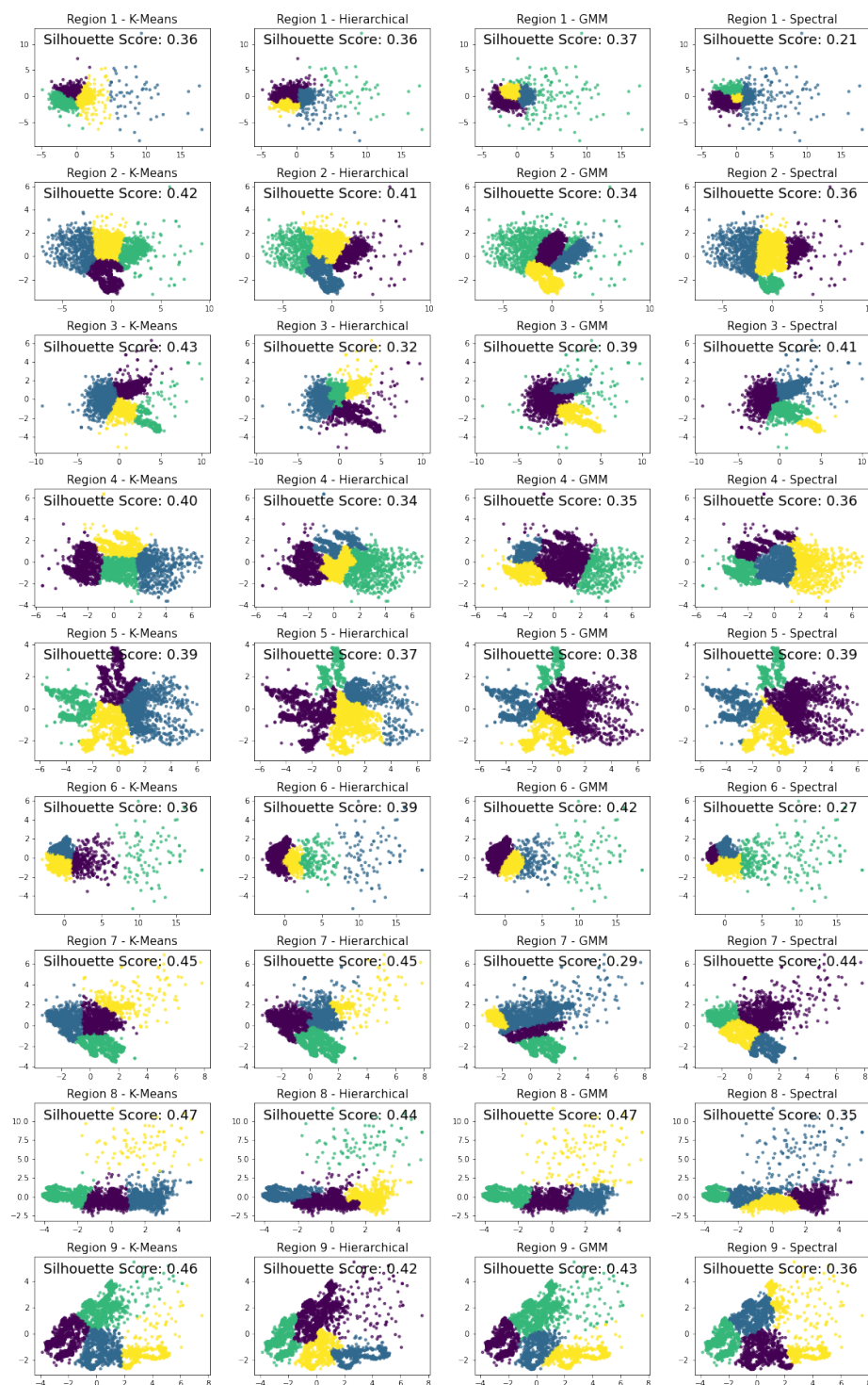
Figure 4. The visualization presents the PCA-based clustering results for volcanic hyperspectral data across nine regions (Regions 1–9), evaluated using four methods: KMeans, Hierarchical, Gaussian Mixture Model (GMM), and Spectral Clustering, with n = 4 clusters. Each panel corresponds to a specific region and clustering technique, accompanied by Silhouette Scores to assess cluster quality (with higher scores indicating better-defined clusters). Notable findings include strong clustering performance in Region 8 (KMeans: 0.47) and Region 8 (GMM: 0.47), while weaker performance is observed in Region 1 (Spectral: 0.21) and Region 6 (Spectral: 0.27).
