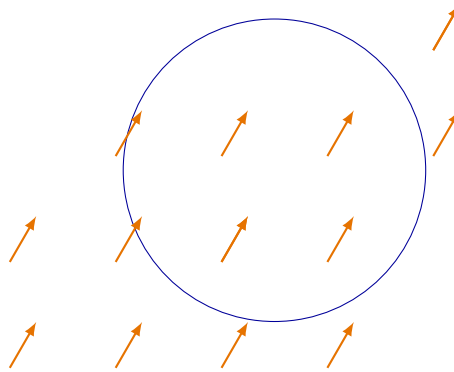
Figure 6. No equilibrium point inside the closed curve \Rightarrow index = 0
