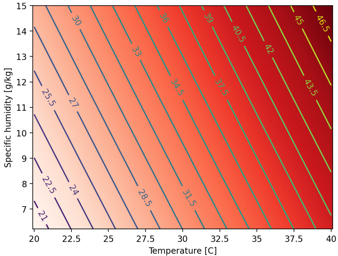
Figure 2. A representative illustration of Humidex (in ° Celsius) as a function of dry bulb temperature and specific humidity. The vapour pressure is calculated using Equation (1) and a pressure of 1015hPa. In extreme conditions (i.e. high temperature and humidity) the difference between the dry bulb temperature and that due to water vapour can exceed 6°.
