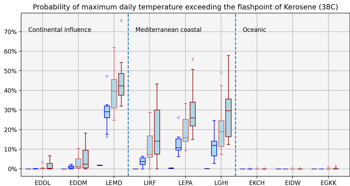
Figure 4. Probability of maximum daily JJA temperature exceeding the flash point of kerosene. The box and whisker plots show the intra-ensemble variability and the historical, SSP1, 3 and 5 results are shown in dark blue, blue, red, and dark red respectively. The three climate regimes are shown, separated by vertical dashed lines.
