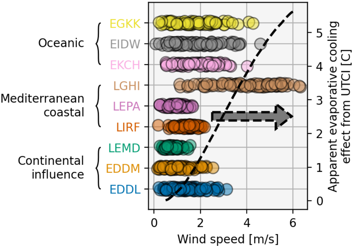
Figure A1. The monthly mean ERA5 wind speed magnitude at 10 m above ground for the airports (and climate regimes) shown on the left-hand y -axis. Some sites' precise locations correspond to ocean points and for these the nearest land point's value is given. The evaporative cooling effect contained within the Universal Thermal Climate Index is shown on the right-hand y -axis [26], calculated using the pythermalcomfort software package described in Tartarini and Schiavon [58].
