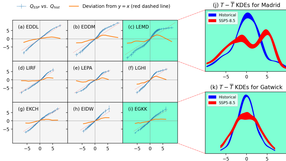
Figure 8. (a-i) Q - Q (percentile-percentile) plots are shown by the blue 'plus' symbols where the extents of the arms in each axial direction show the respective inter-model spread. The historical data is on the x axis and the y axis shows the SSP5-8.5 results. The diagonal line ( y = x ) shows the line that would be made by the Q - Q plots if the distributions were identical. The solid line is the deviation from the y = x line on the same y -axis scale. (a-c) are continentally influenced; (d-f) are Mediterranean coastal; (g-i) are oceanic. Note that the green lines in (c) and (i) show large and small amounts of deviation from y = x respectively; (j) and (k) show the Gaussian kernel density estimate distributions (and standard errors, \frac{\sigma}{\sqrt{N_{\text{models}}}} ). The x -axis ranges of the KDE plots is chosen to match the historical Q ranges in (c) and (i) respectively.
