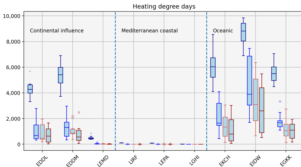
Figure 6. Heating degree days for each SSP. The box and whisker plots show the intra-ensemble variability and the SSP1, 3 and 5 results are shown in blue, red, and dark red respectively. The three climate regimes are shown, separated by vertical dashed lines.
