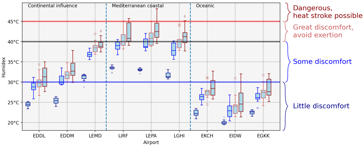
Figure 3. box-and-whisker plots of Humidex , H , for each of the airports shown in Figure 1 and for each SSP scenario. The coloured horizontal lines and the text on the right hand side illustrate the pre-defined levels of comfort shown in Table 3. The three climate regimes are shown, separated by vertical dashed lines.
