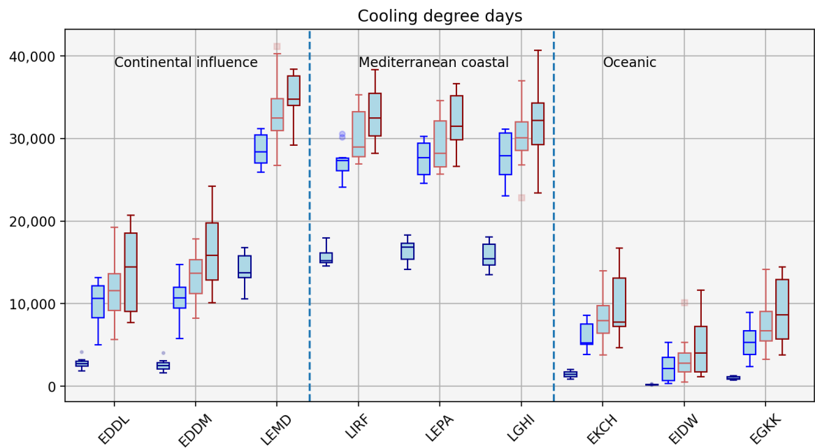
Figure 5. Number of Cooling degree days for each SSP. The box and whisker plots show the intra-ensemble variability and the SSP1, 3 and 5 results are shown in blue, red, and dark red respectively. The three climate regimes are shown, separated by vertical dashed lines.
