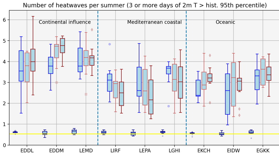
Figure 7. The number of heatwaves experienced by each site where a heatwave is defined as a 3-or-more day period of daily mean 2m temperatures exceeding the 95th percentile of the historical simulations for each model respectively. The box and whisker plots show the intra-model ensemble variability and the historical, SSP1, 3 and 5 results are shown in dark blue, blue, red, and dark red respectively. The three climate regimes are shown, separated by vertical dashed lines and the yellow horizontal is the 1985-2014 JJA heatwave occurrence from the Central England Data set.
