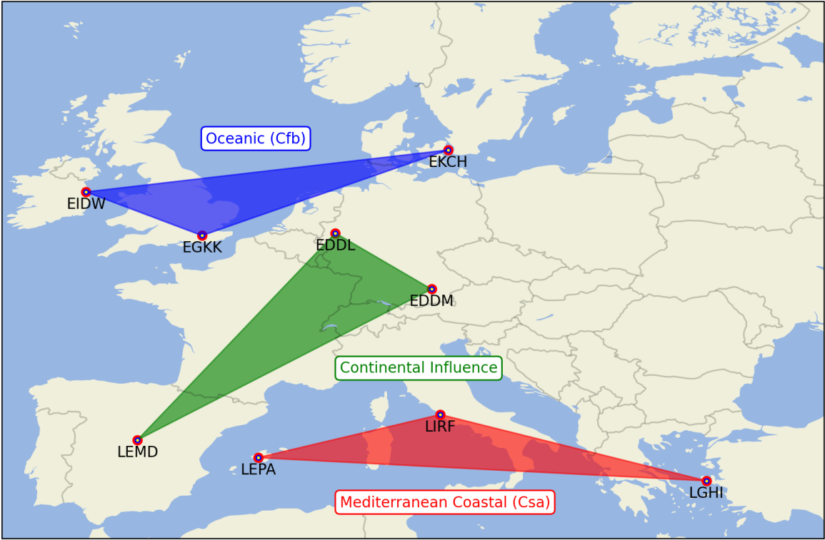
Figure 1. The subset of 9 airports chosen to better visually represent the larger 30 airport ensemble. The blue region represents oceanically-controlled sites, the green regions shows those with a large continental influence and the red region shows those of a coastal Mediterranean nature. Precise coordinates are given in Table 2.
