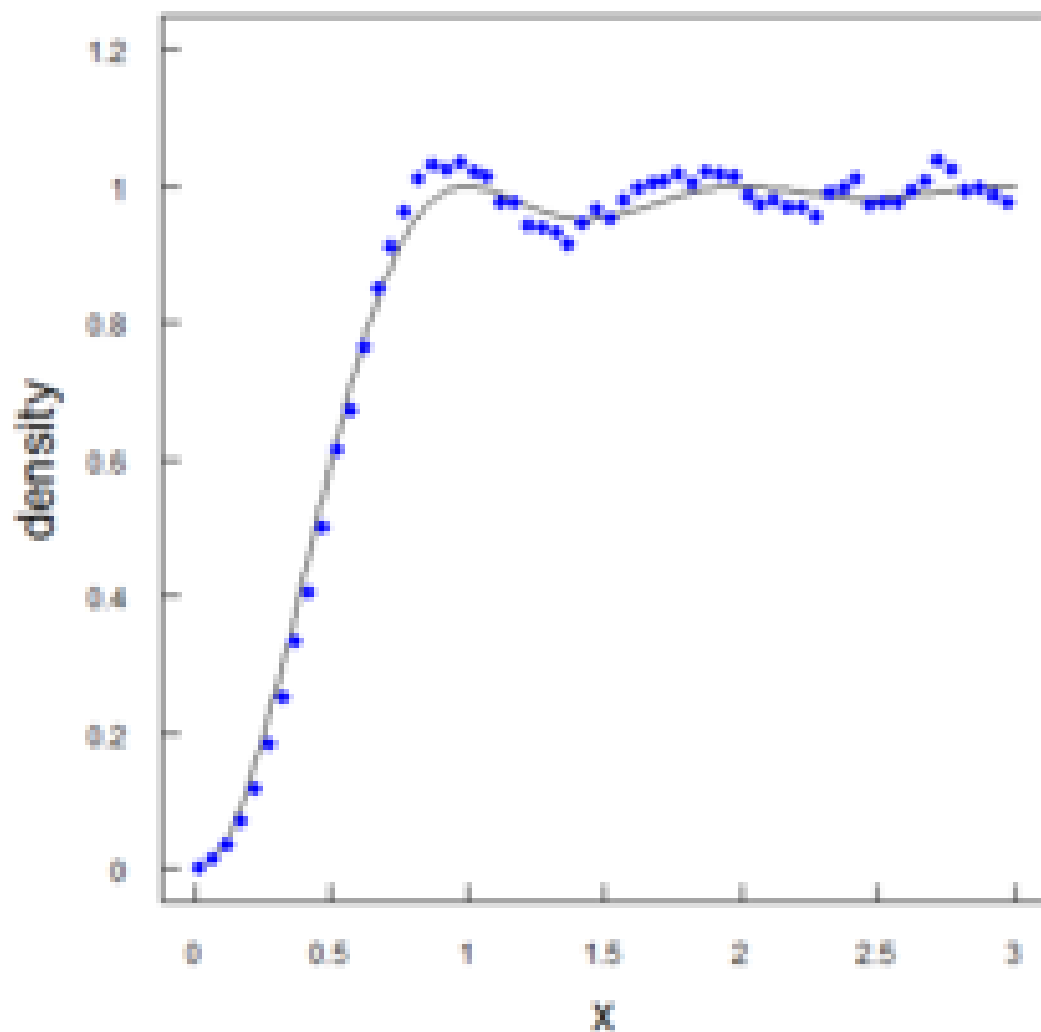
Figure 3. Connection between zeta zeros and quantum statistics
