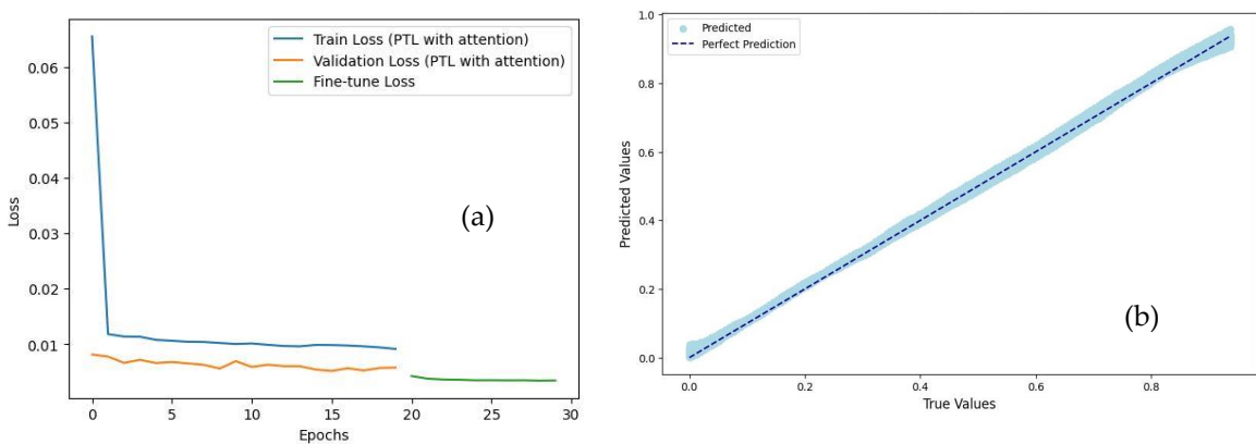
Figure 4. (a) Training, validation, and fine-tuning loss curves; (b) Predicted vs. actual damage index from regression model.
