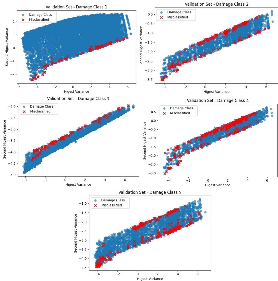
Figure 6. Comparison between actual and predicted class distribution of structural damage states using PTL classifier.
