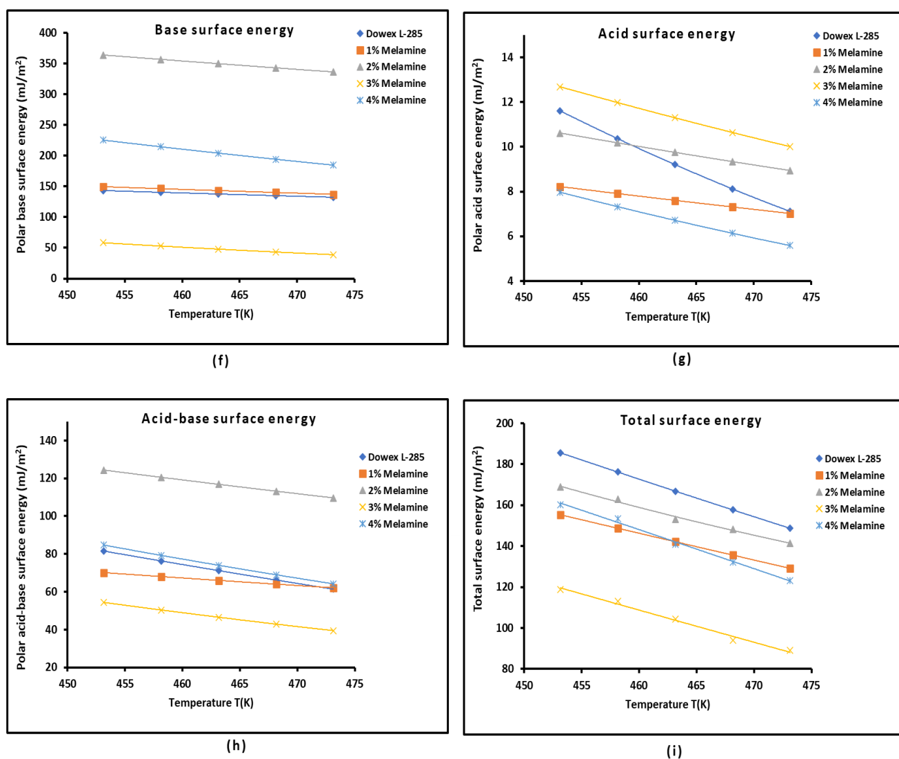
Figure 7. Variations of acid and base surface energy components, and total energy (in mJ/m 2 ) of Dowex L-285 modified by different melamine percentages as a function of temperature: Dowex L-285 (a), 1% Melamine (b), 2% Melamine (c), 3% Melamine (d), 4% Melamine (e), base surface energy (f), acid surface energy (g), acid-base surface energy (h), total surface energy (i).
