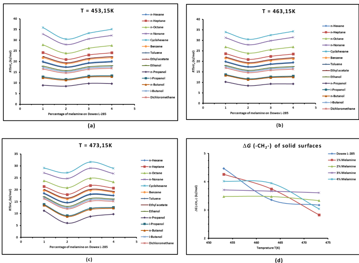
Figure 1. Effect of the percentage of melamine on the values of RT\ln V_n(T) of different adsorbed organic solvents at various temperatures: T = 453.15K (a), T = 463.15K (b), T = 473.15K (c), and variations of \Delta G_a(-CH_2-) of n-alkanes adsorbed on solid surfaces as a function of temperature (d).
