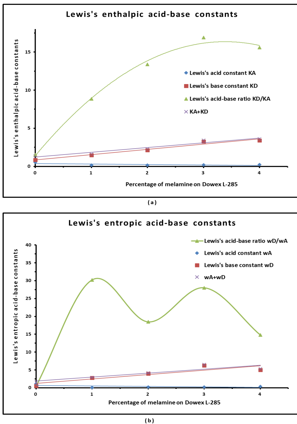
Figure 6. Curves of the Lewis's enthalpic and entropic acid-base constants K_A , K_D , \omega_A , \omega_D , the acid-base ratios, and the corresponding parameters S_K = K_A + K_D and S_K = \omega_A + \omega_D , as a function of melamine percentage.
