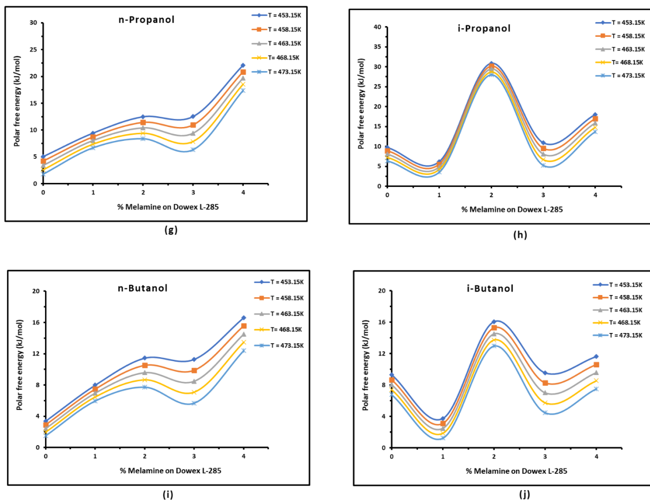
Figure 4. Variations of the free polar energy [-\Delta G_a^p(T)] of polar organic probes adsorbed on the different solid materials as a function of melamine percentage on Dowex L-285 at various temperatures. (a): dichloromethane, (b): cyclohexane, (c): benzene, (d): toluene, (e): ethyl acetate, (f): ethanol, (g): n -propanol, (h): i -propanol, (i): n -butanol, and (j): i -butanol.
