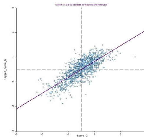
Figure 3. Calculation of the Moran's Index for educational quality.
