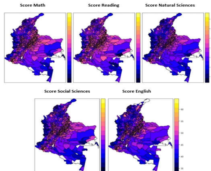
Figure 1. Spatial distribution of scores obtained by evaluated area.
