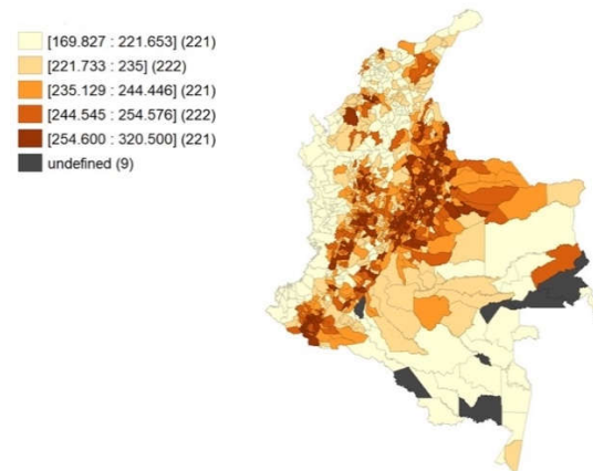
Figure 2. Spatial distribution of the Global Score.
