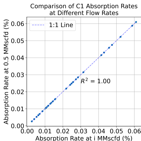
Figure 6. Effect of flow rate on C1 absorption rate. Gas flow rates, (i), were varied from 2.9 to 17.5 MMscfd, with a fixed baseline case at 0.5 MMscfd as described in sub-section 2.4.
