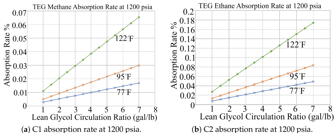
Figure 5. Simulated absorption behavior of (a) C1 and (a) C2 in TEG at 1200 psia. At this elevated pressure, C1 absorption increases under all conditions, whereas C2 absorption decreases. C2 remains considerably more soluble than C1, representing the upper bound of absorption behavior modeled in MAES.
