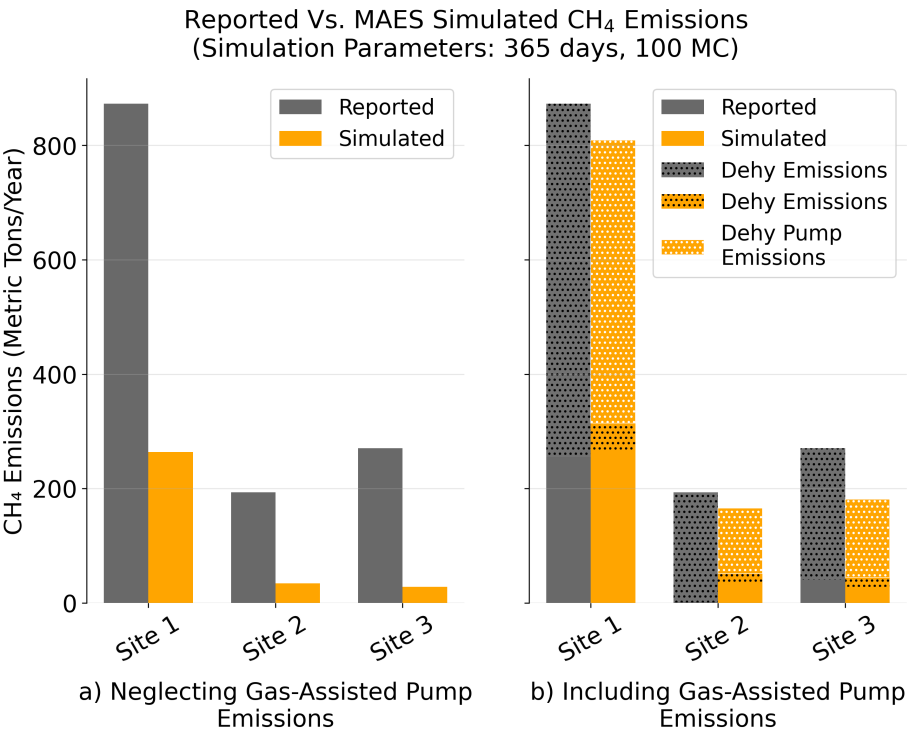
Figure 7. Comparison of reported and MAES-simulated CH 4 emissions for three midstream facilities under two modeling scenarios: (a) MAES dehydrator model neglecting gas-assisted pump emissions, and (b) the model with gas-assisted pump emissions included, explicitly highlighting hatched dehydrator emissions. Each subplot displays reported emissions (gray bars) alongside simulated emissions (orange bars) for each site.
