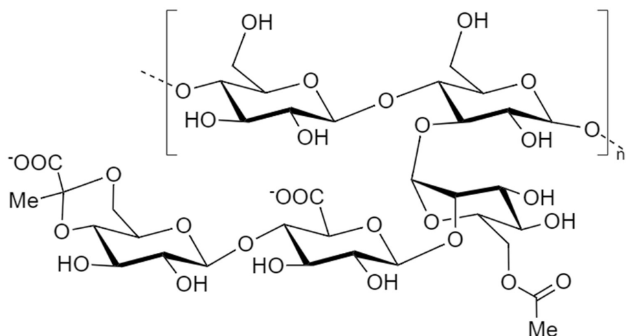
Figure 8. Chemical structures of Xanthan gum.
