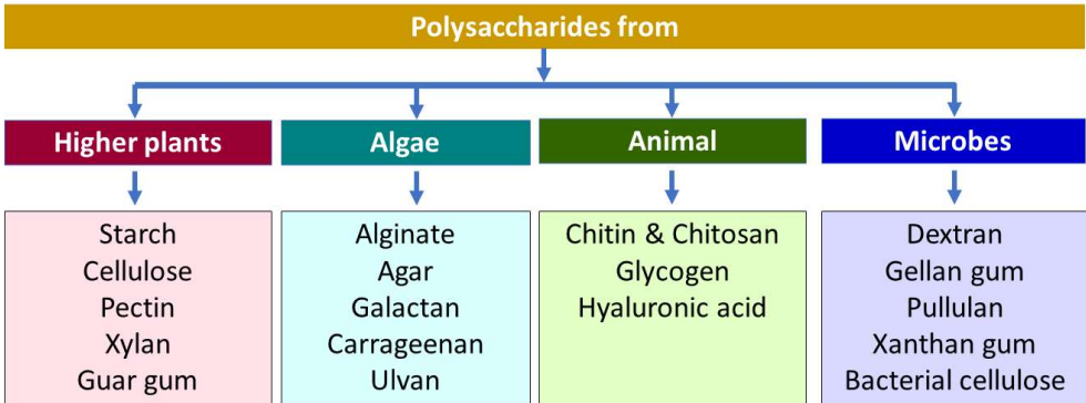
Figure 2. Classification of polysaccharides based on their origin.
