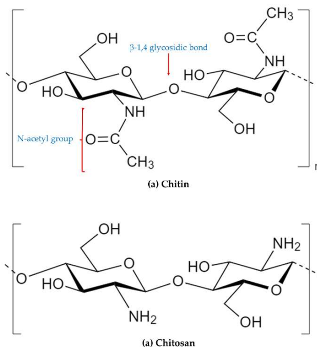
Figure 5. Chemical structure of (a) chitin and (b) chitosan.
