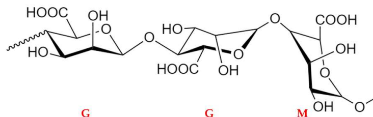
Figure 3. Structure of alginic acid.
