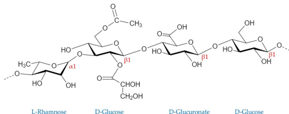
Figure 7. Chemical structures of gellan gum.
