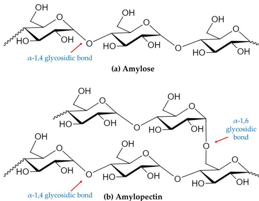
Figure 2. Structure of the amylose and amylopectin.
