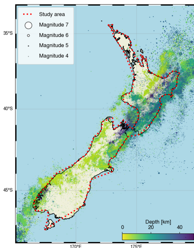
Figure 2. Earthquake locations by magnitude and depth of the events used in this study. The dotted line marks the NESTORE study area.
