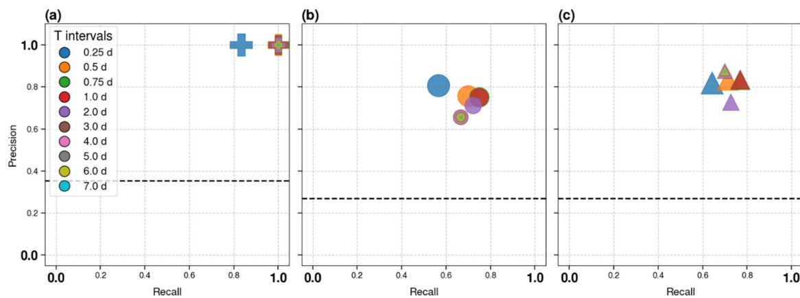
Figure 7. Precision-Recall diagrams for the (a) chronological, (b) k-fold, and (c) autotest approaches.
