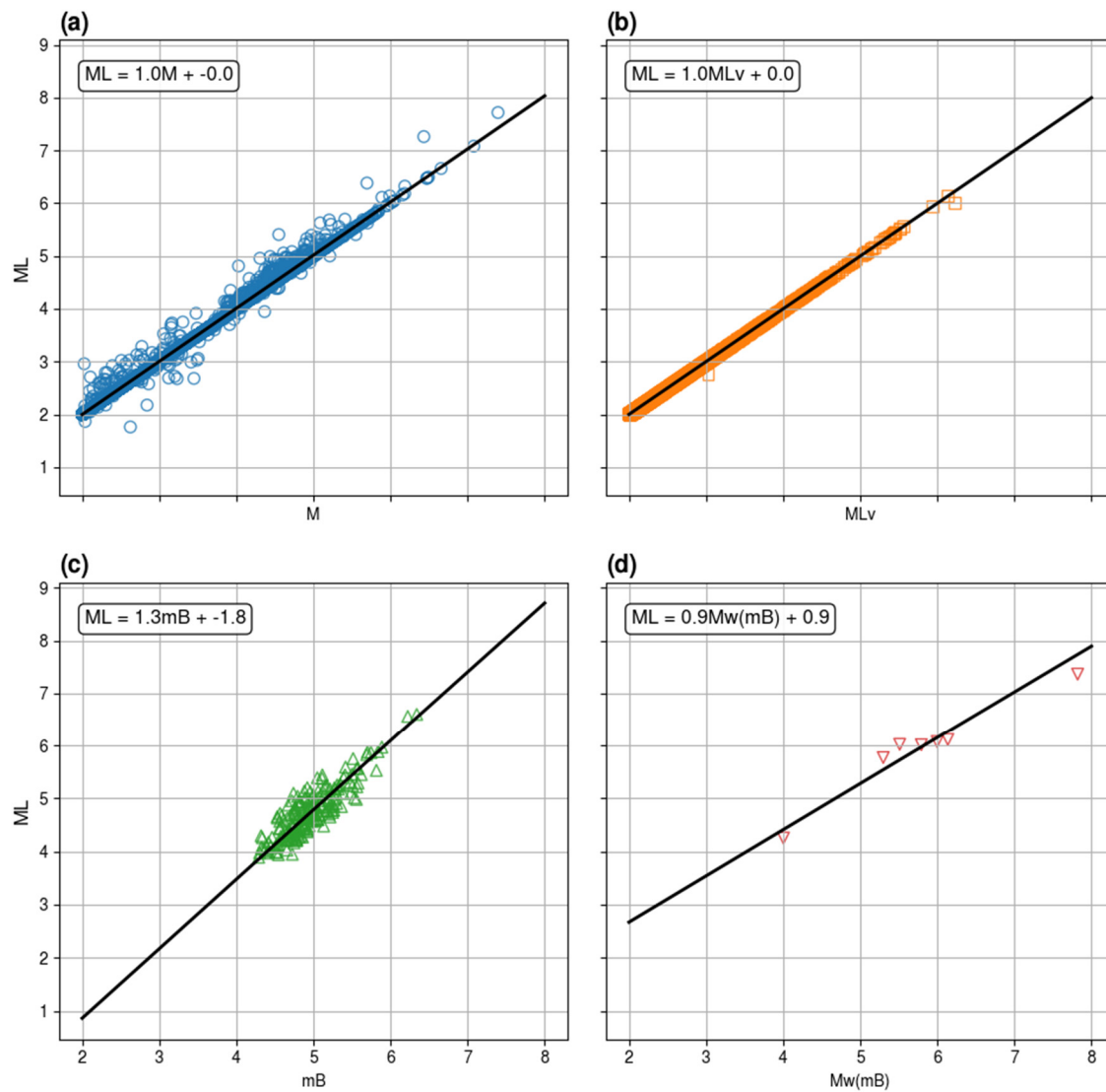
Figure 3. Orthogonal regression between magnitude scales listed in GeoNet Quake Search system and ML from the revised earthquake catalogue for New Zealand [61]. Both M and MLv fit the data approximately 1:1.
