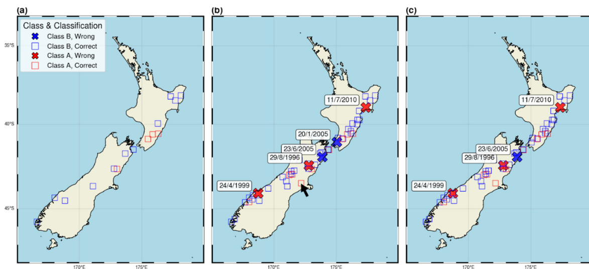
Figure 5. Test set in the three analyzed cases: (a) chronological; (b) k-fold; (c) autotest. The black arrow in (b) marks the September 2010 Canterbury earthquake.
