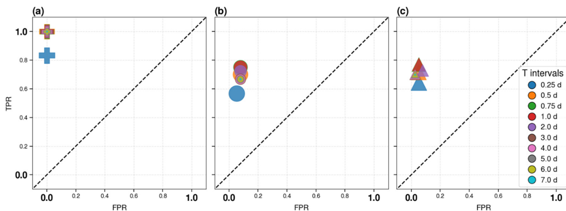
Figure 6. ROC diagram in the (a) chronological, (b) k-fold, and (c) autotest approach. The Time interval end is expressed in fraction of day.
