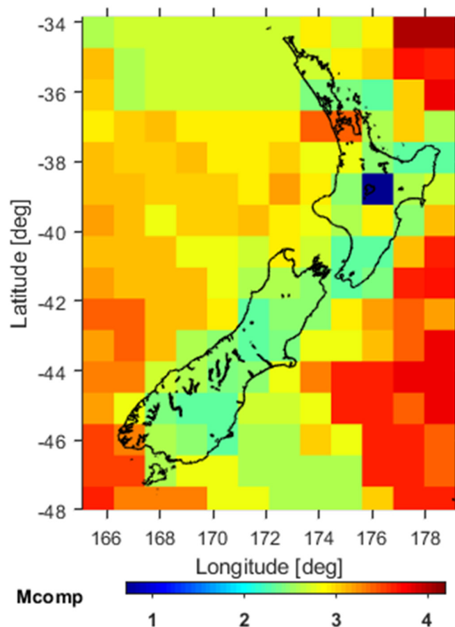
Figure 4. Completeness magnitude of the catalogue in space.
