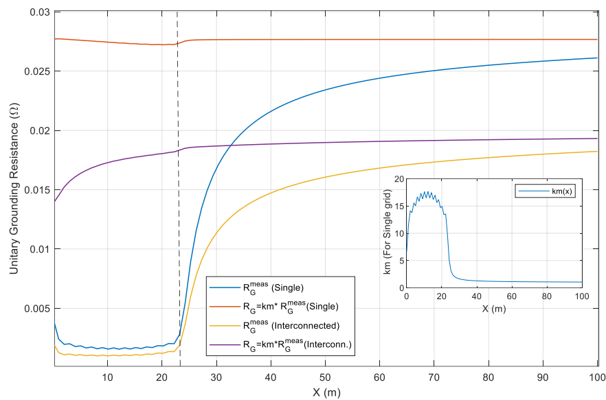
Figure 6. Representation of the different measurement procedure parameters as a function of the distance from the edge of the Balaidos grid. An interconnected case with other grounding system is also considered.
