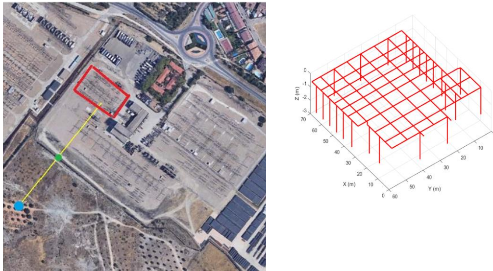
Figure 7. In the left panel, the Loeches substation, marked in red. The blue dot is the auxiliary current electrode 211 meters away from the grid edge. (Courtesy of Union Fenosa Distribucion, UFD). The grounding grid is shown on the right panel.
