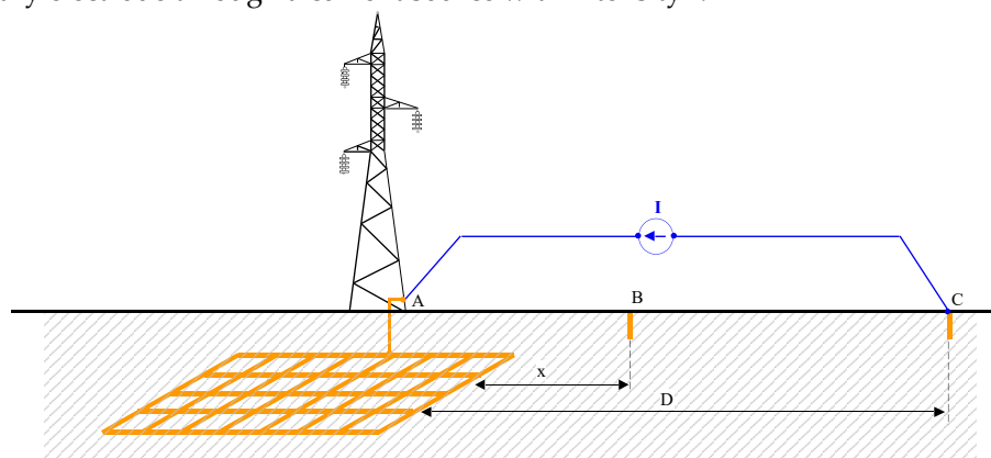
Figure 1. Practical illustration of the Three-Pin method for measuring the grounding resistance R_G .
