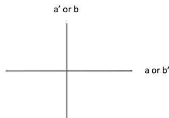
Figure 9. Relative eigenbases configuration for the like states of Eq. (30) satisfying the last three PR correlations.
