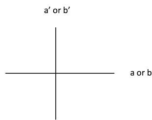
Figure 8. Relative eigenbases configuration for the unlike states of Eq. (30) satisfying the last three PR correlations.
