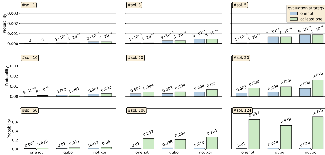
Figure 2. Probabilities of measuring a feasible solution as a function of the number of feasible solutions in the instance and the chosen encoding. The probabilities are evaluated in two ways. First, we sum the probabilities for all correct one-hot measured bitstrings (blue bars). Second, we sum the probabilities for all bitstrings that correspond to the aircraft performing at least one maneuver (green bars).
