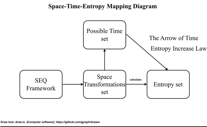
Figure 1. Space-Time-Entropy Mapping Diagram.
