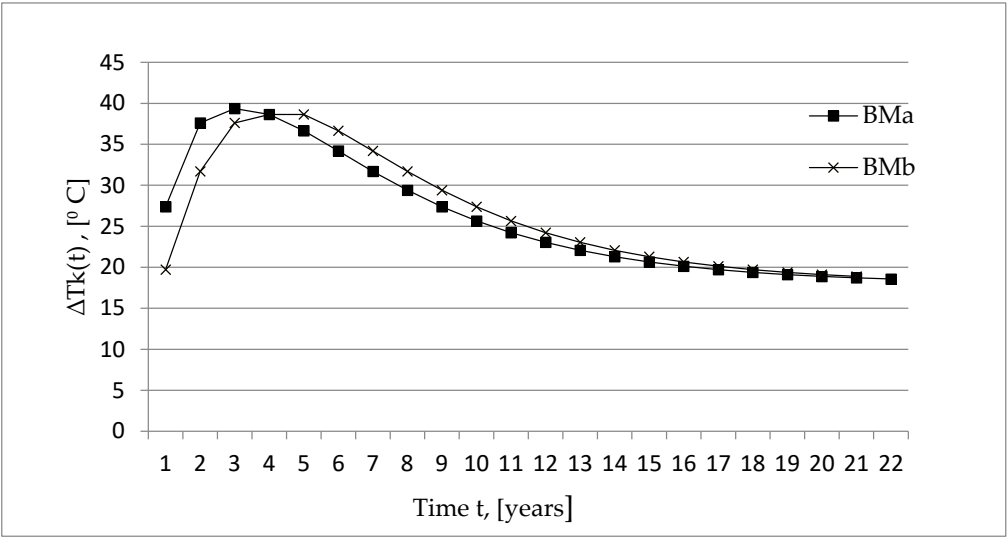
Figure 10. Function \Delta T_K(t) of the RPV base metals BM.
