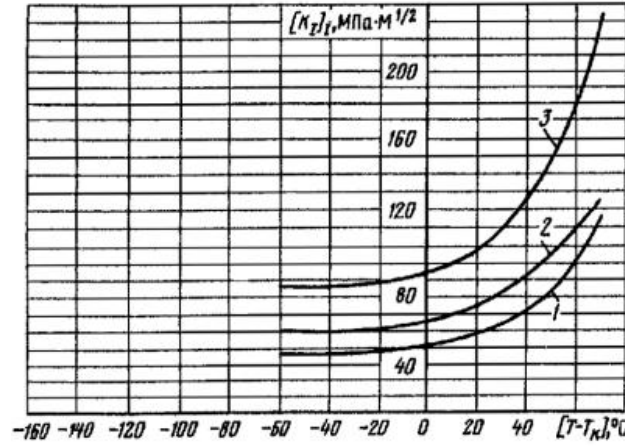
Figure 6. [K_I] is a function of \Delta T_K of RPV metal, [7]. Curve 1 – NOC of the unit; curve 2 – NNOC&HT if the unit; curve 3 – EC of the unit.
