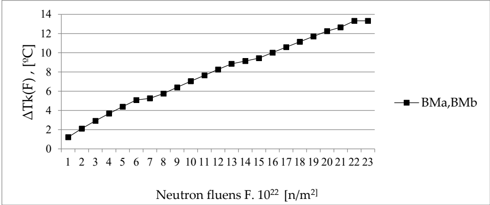
Figure 9. Function \Delta T_K(F) for base metal BM of the RPV metals.
