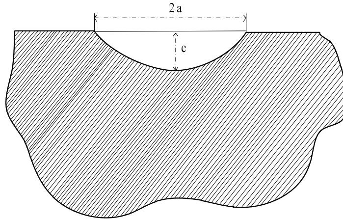
Figure 3. Surface defect diagram (Semi-ellipse with a semi-major axis “a” and a semi-minor axis “c”).
