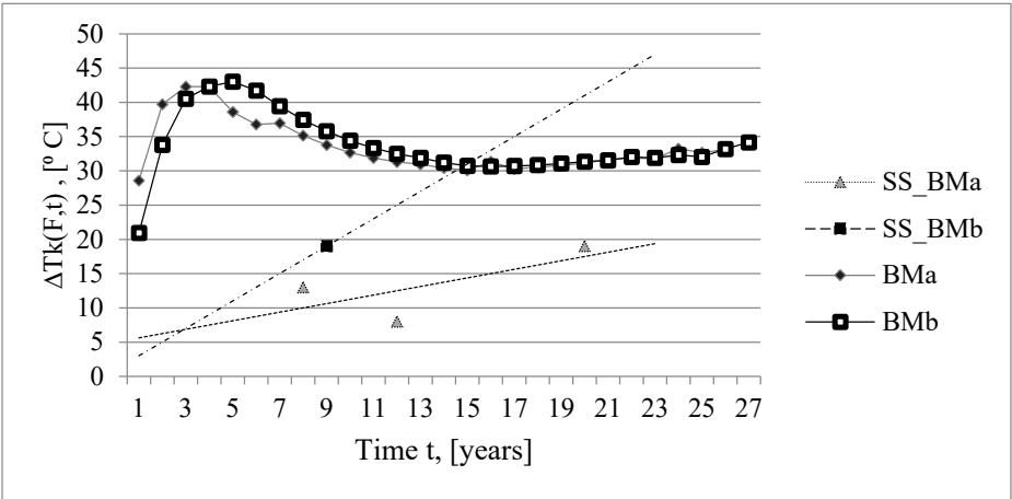
Figure 11. Function \Delta T_K(F, t) of the time t for the base metal BM. A mediated line of experimental data from the surveillance specimens SS for the base metal BM.
