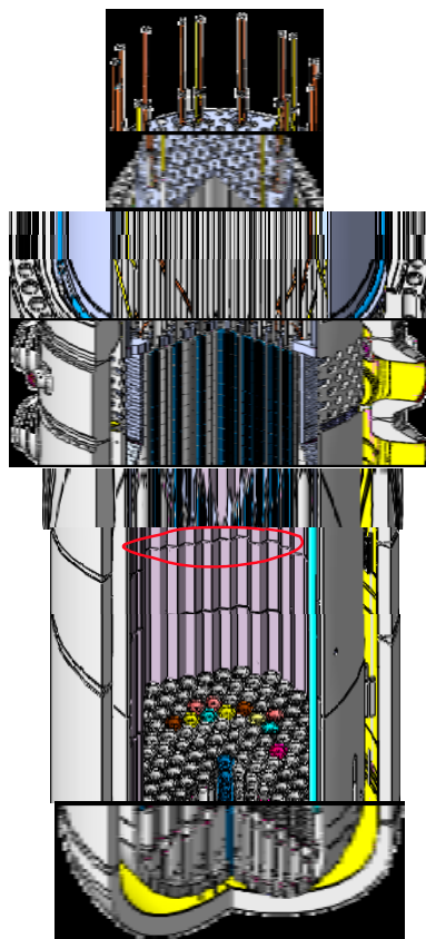
Figure 1. Reactor Pressure Vessel Internals, area with detected defects is shown in red.
