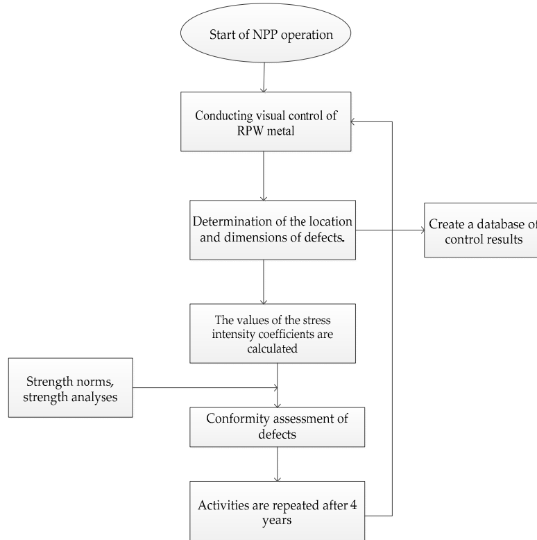
Figure 5. Planning and Conducting Visual control of Reactor Metal.
