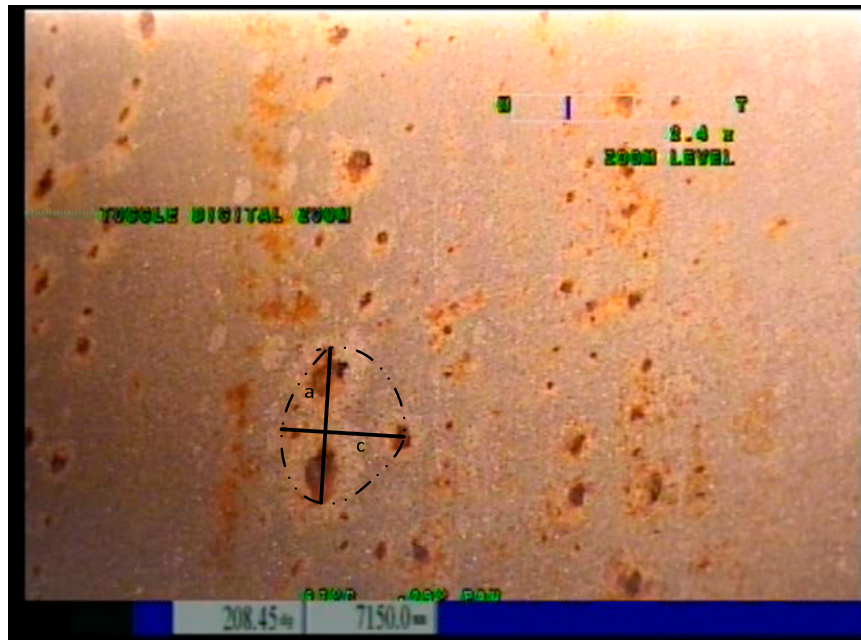
Figure 7. Cluster of defects on the inner surface of the reactor vessel.
