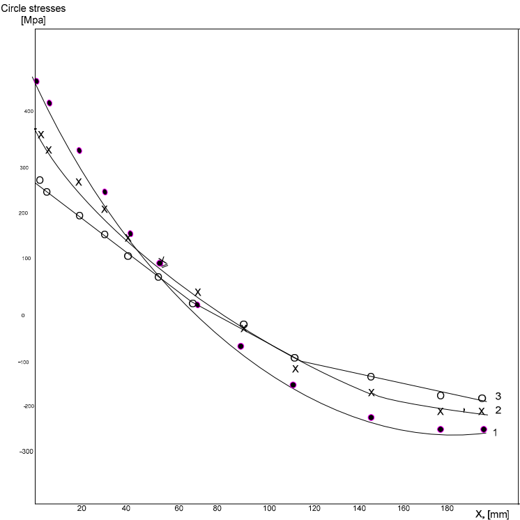
Figure 8. Relative Stress Distribution as a Function of the Distance X from the Boundary of the Overlay with the Base Metal. ( X = 0 e position closest to the inner surface of the Reactor vessel. The current loads have maximum values). Curve 1 – currently 0,2 hours from the time interval of the “Big Primary Leak” mode; Curve 2 – at 0.4 hours; Curve 3 – at 0.6 hours.
