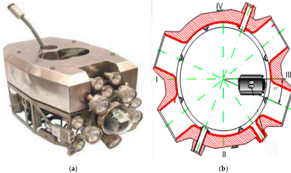
Figure 2. Visual control equipment and scheme for scanning the RPV inner surface: (a) Underwater system for RPV visual testing; (b) Scheme of visual testing of the RPV metal.
