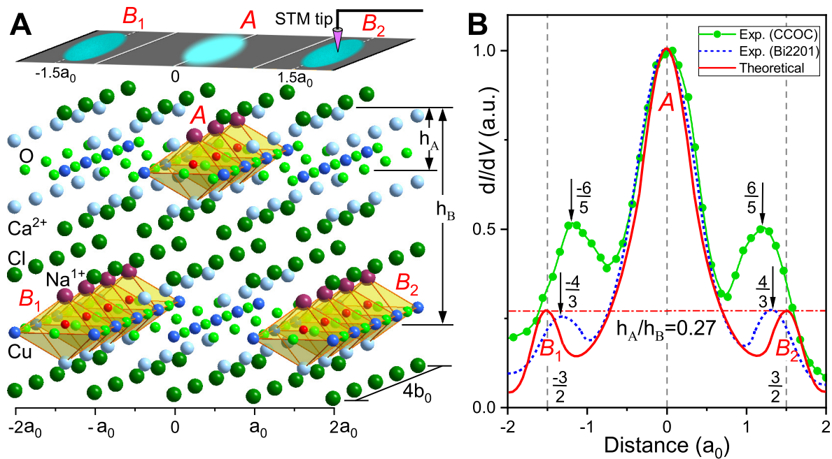
Figure 3. Explanation of local nematic states in Copper-based Superconductors. (A) In the 4a_0 \times 4b_0 plaquette of CCOC, the metallic electrons from the three quantum wells (A) in the central of the upper CuO 2 layer contribute to the central brightest bar in the STM experiment, while electrons from the four quantum wells (B 1 and B 2 ) on both sides of the lower layer contribute to the two sidebars. (B) The normalized DOS peaks are represented by red as theoretical results, with smaller peaks appearing at \pm 1.5a_0 . The experimental results for CCOC and Bi2201 are shown in green and blue, respectively, with smaller peaks around \pm 1.2a_0 and \pm 1.3a_0 . The red dotted line represents the weak peak value of 0.27, which is determined by the distances ( h_A and h_B ) between the CuO 2 planes and the cleavage plane.
