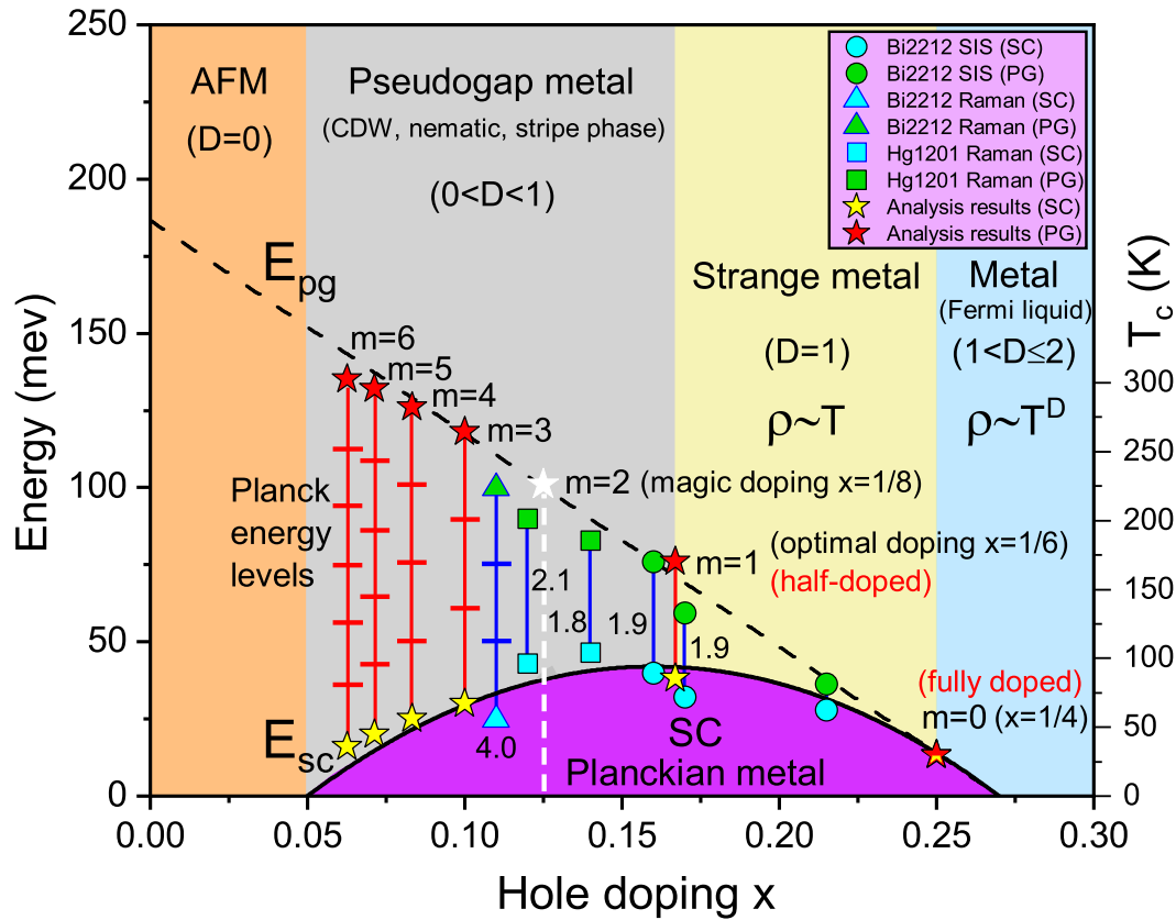
Figure 4. HTSC theoretical phase diagram. The diagram shows five phases: a dome-shaped superconducting phase and four others separated by half-doping ( x = 1/6 ) and full-doping ( x = 1/4 ): undoped AFM (orange), underdoped pseudogap metal (gray), overdoped strange metal (yellow), and heavily overdoped Fermi liquid (blue). Triangles/squares represent experimental two-gap measurements in HTSCs, consistent with Hüfner et al.'s fitting for the dome-shaped superconducting scale and linear pseudogap [29]. Pentagrams denote theoretical dual gaps: yellow star (Planck ground state) and red pseudogap (Planck excited state related to doping quantum number m ), with distinct evolution patterns. In the model, normal-state phenomena depend on real-space electron structure dimension D : D = 0 (undoped), 0 < D < 1 (weak doping, short-range clusters), D = 1 (strange metal region, 1D electron states causing linear-in-T resistivity), and D > 1 (Fermi liquid, disrupting 1D charge order in Figure 2A and \pi -shift structure in Figure 1E, leading to failed linear resistivity).
