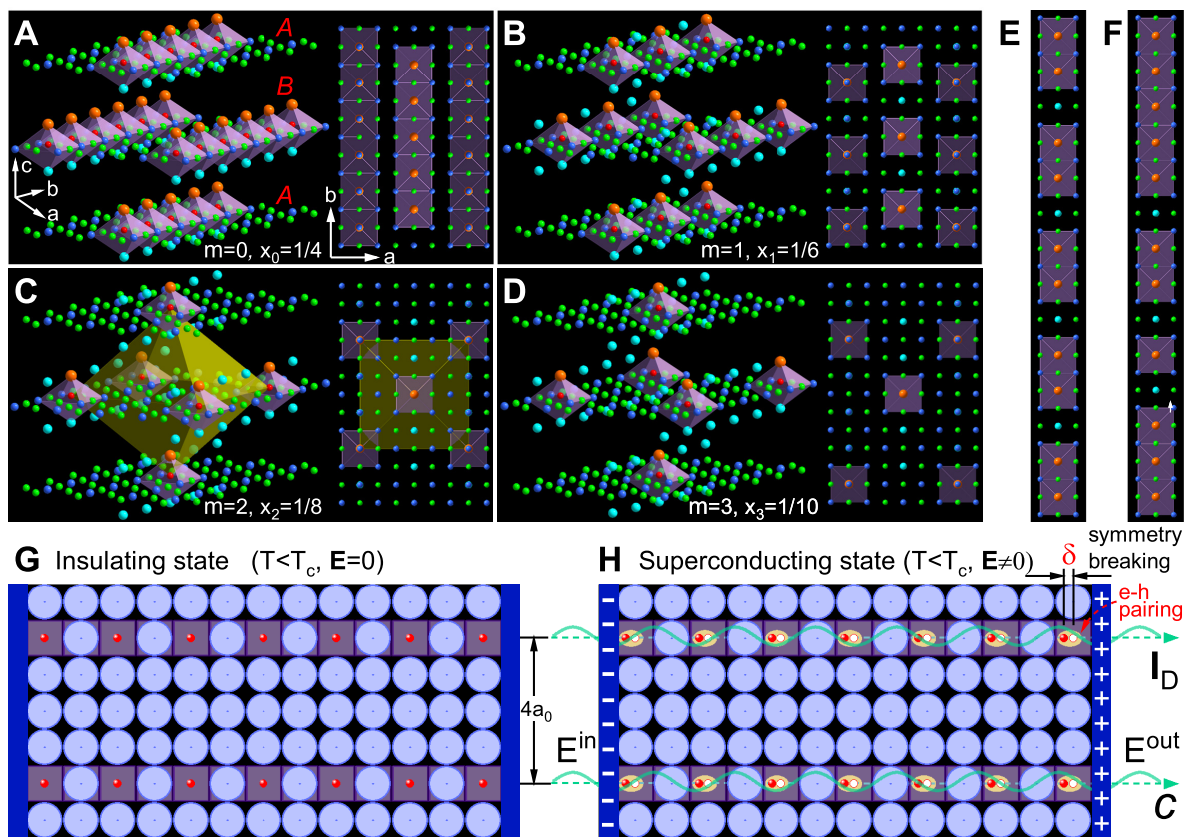
Figure 2. Evolution of charge-ordered structures with doping and two-step superconducting transitions in cuprates. (A) At m = 0 : Highest-doped superconducting state with saturated quasi-1D charge stripes as inset. (B) At m = 1 (optimal doping): Semi-filled charge stripes; inset shows coexisting doped conducting and undoped insulating domains [24]. (C) At m = 2 (magic doping): Electrons form non-superconducting 4 \times 4 checkerboard charge order via repinning. (D) At m = 3 (underdoped). (E) At fractional m = 1/2, x = 1/5 . (F) Disordered-doped quasi-1D stripes. (G) Below T_c , electrons in optimally doped \text{CuO}_2 (A) condense into a rigid insulating state; coherent condensation occurs without superconducting transition. (H) External electric fields induce symmetry breaking and e-h pairing, forming polarization capacitors for lossless Maxwell displacement currents (Electromagnetic field energy propagating at speed c ).
